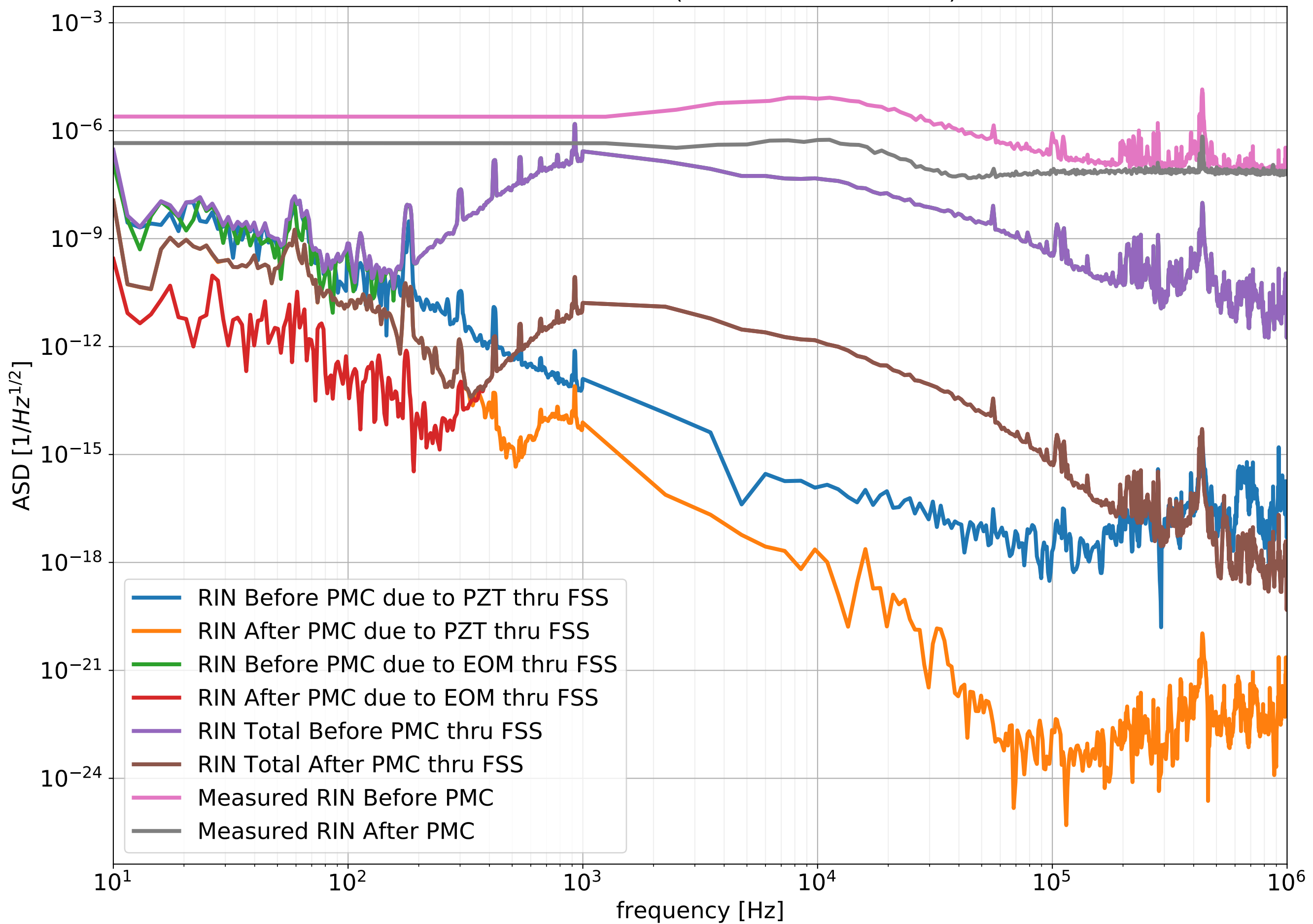
RIN ASD due to FSS (Estimated vs Measured)
