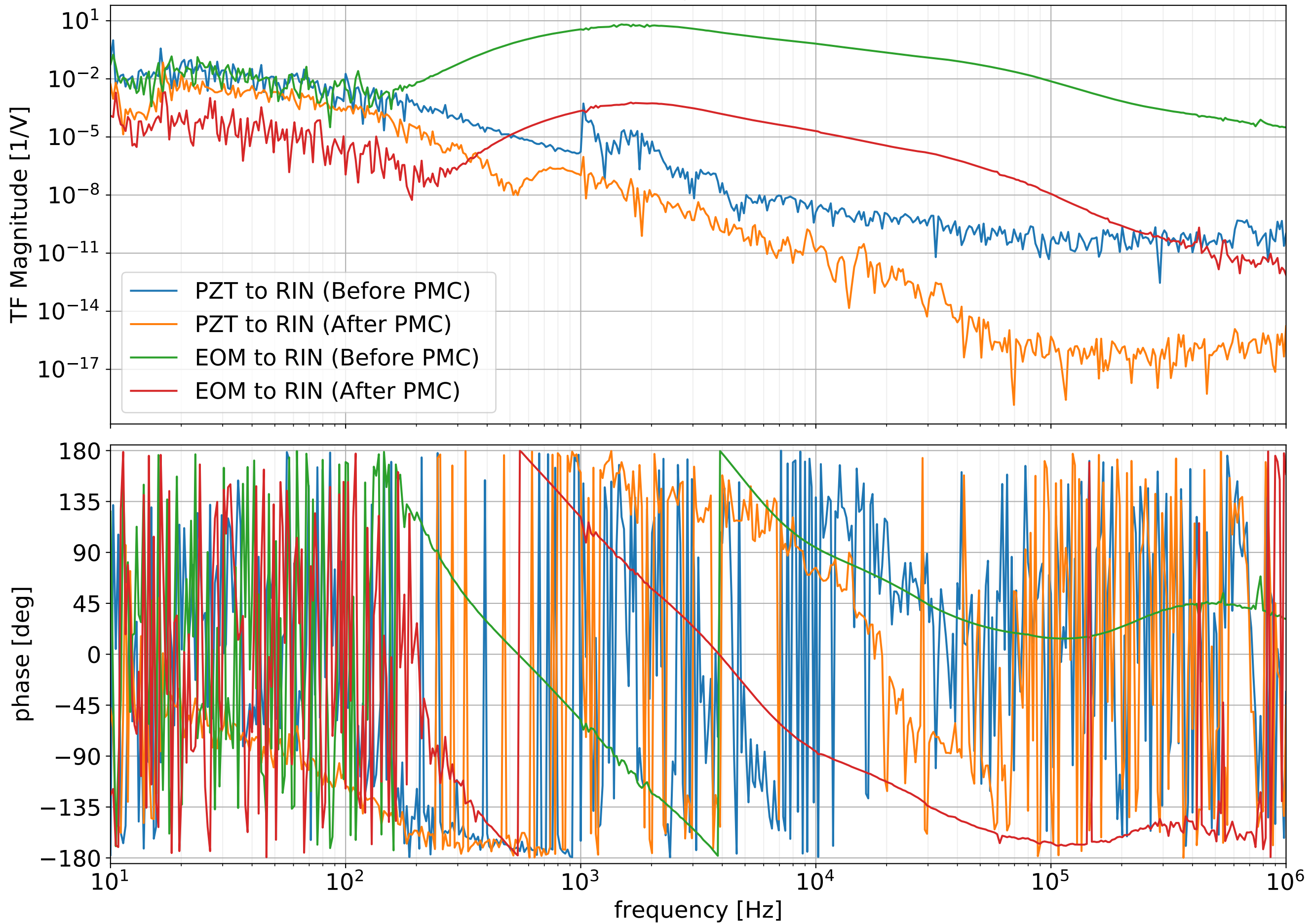
Transfer Function from Test2 EXC to RIN COM Gain = 6 dB, FAST Gain = 10 dB
