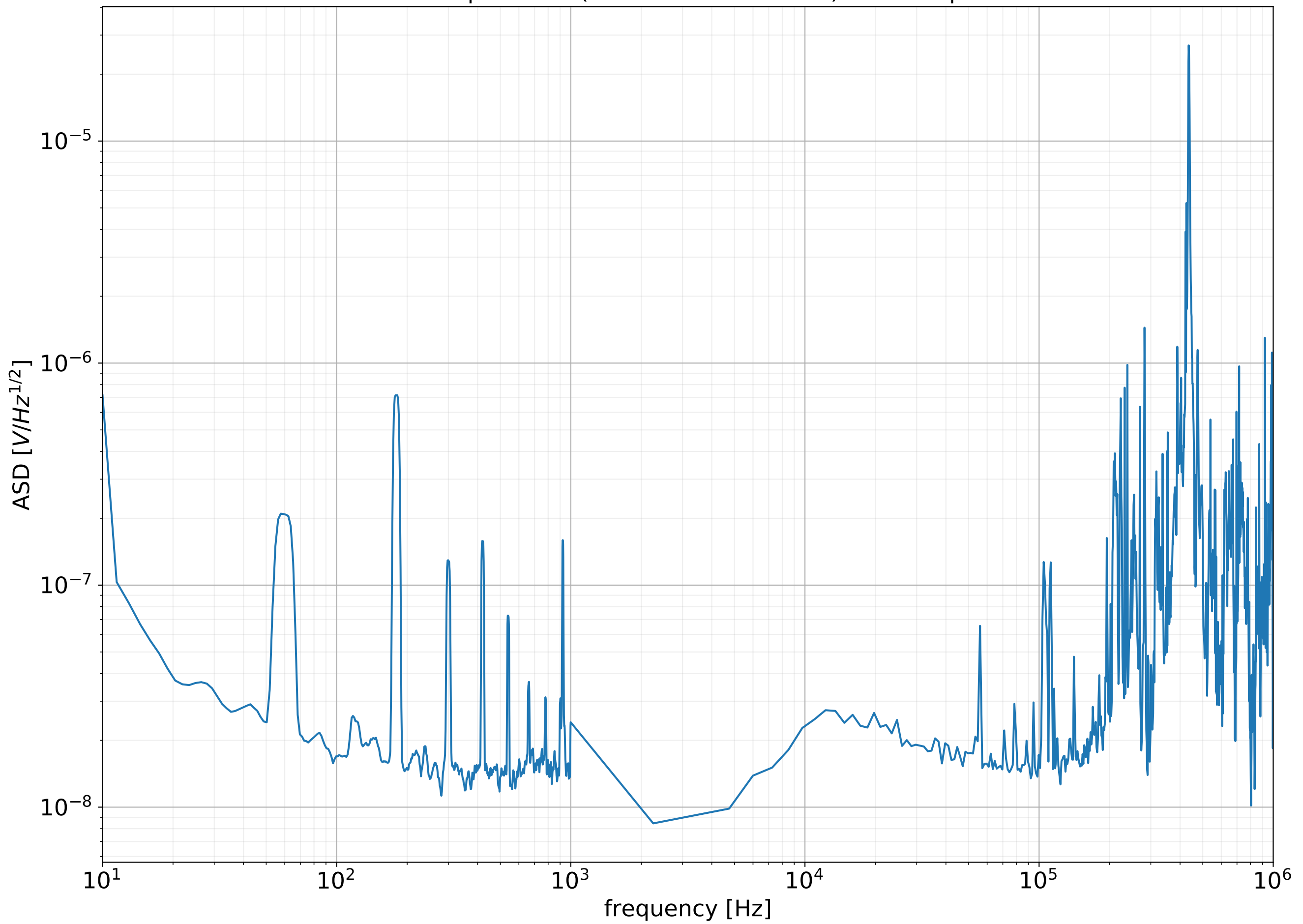
ASD at output of U3 (NFSS Common Board) when loop is ON
