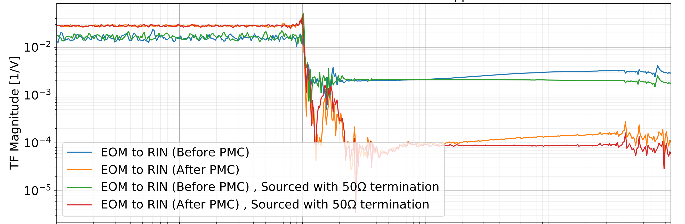
EOM to RIN Transfer Function with 20 dBm applied on EOM
