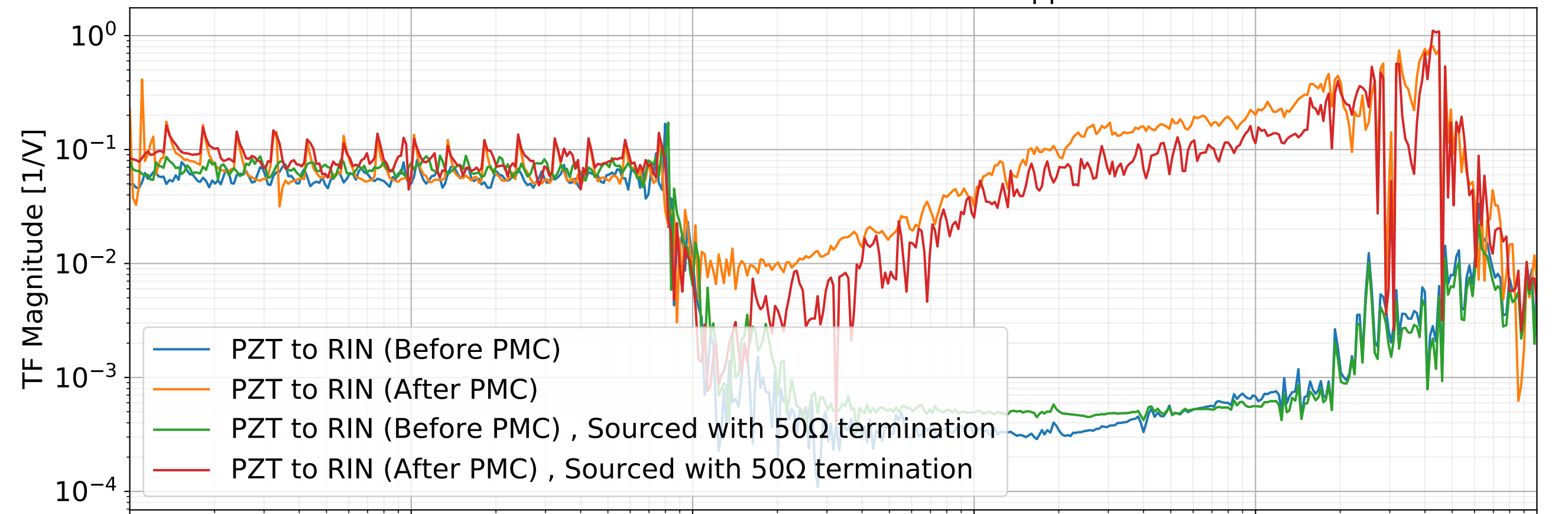
PZT to RIN Transfer Function with 0 dBm applied on PZT
