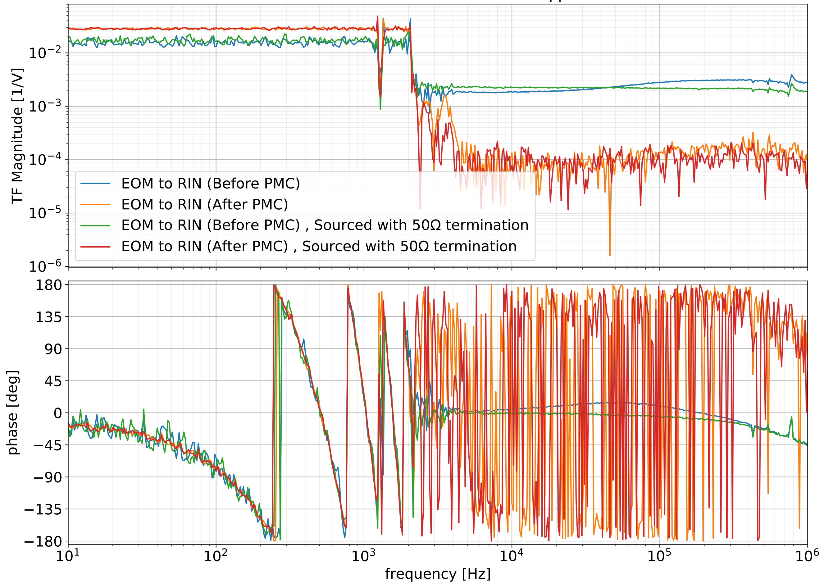
EOM to RIN Transfer Function with -20 dBm applied on EOM
