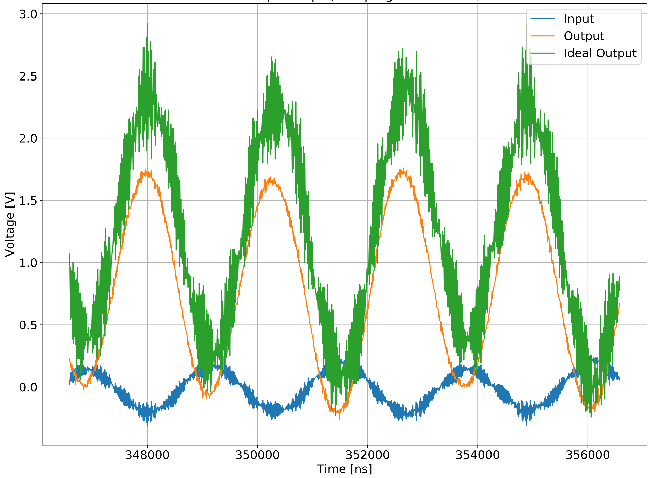
NFSS U7 Input Output, Sampling Rate 0.1 GSa/s
