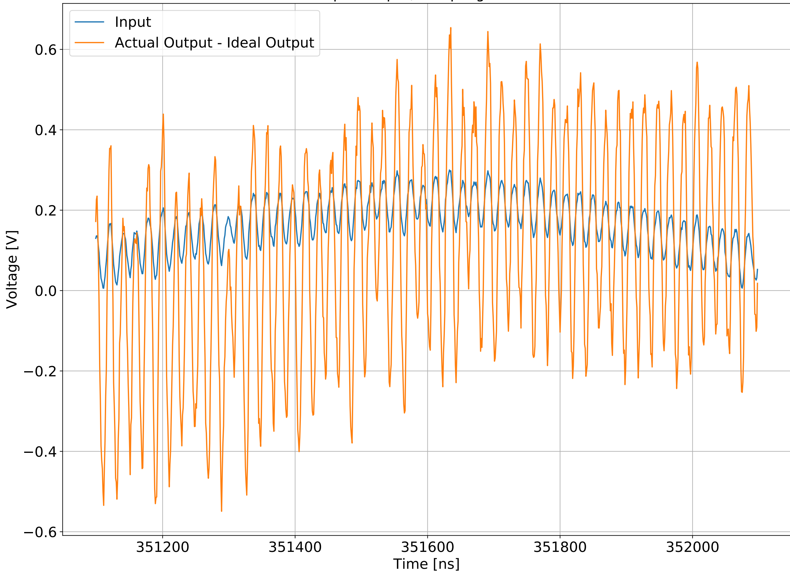
NFSS U7 Input Output, Sampling Rate 1.0 GSa/s
