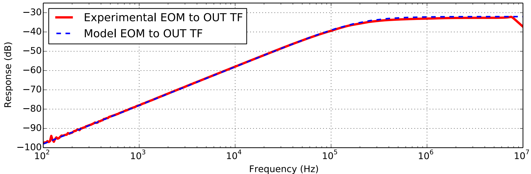
Transfer Function of EOM
