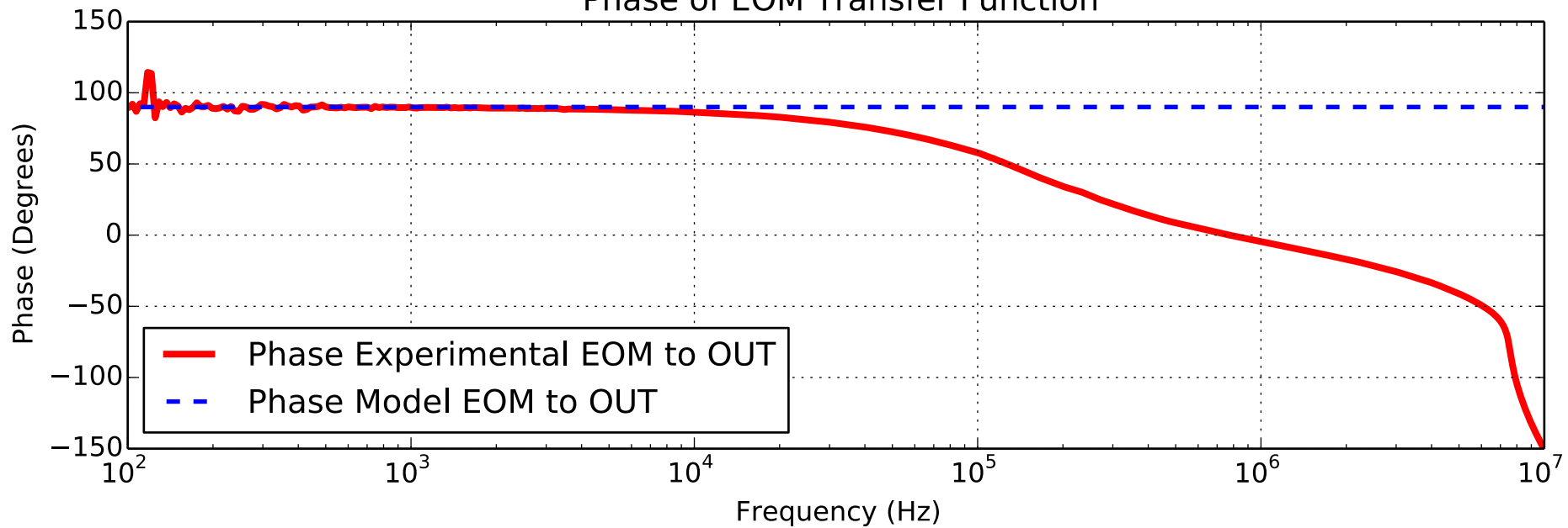
Phase of EOM Transfer Function
