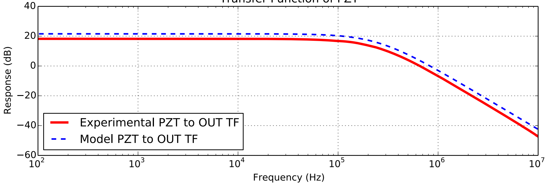
Transfer Function of PZT
