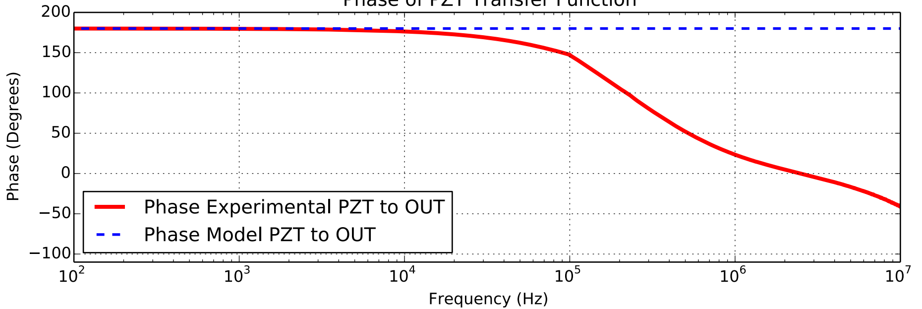
Phase of PZT Transfer Function
