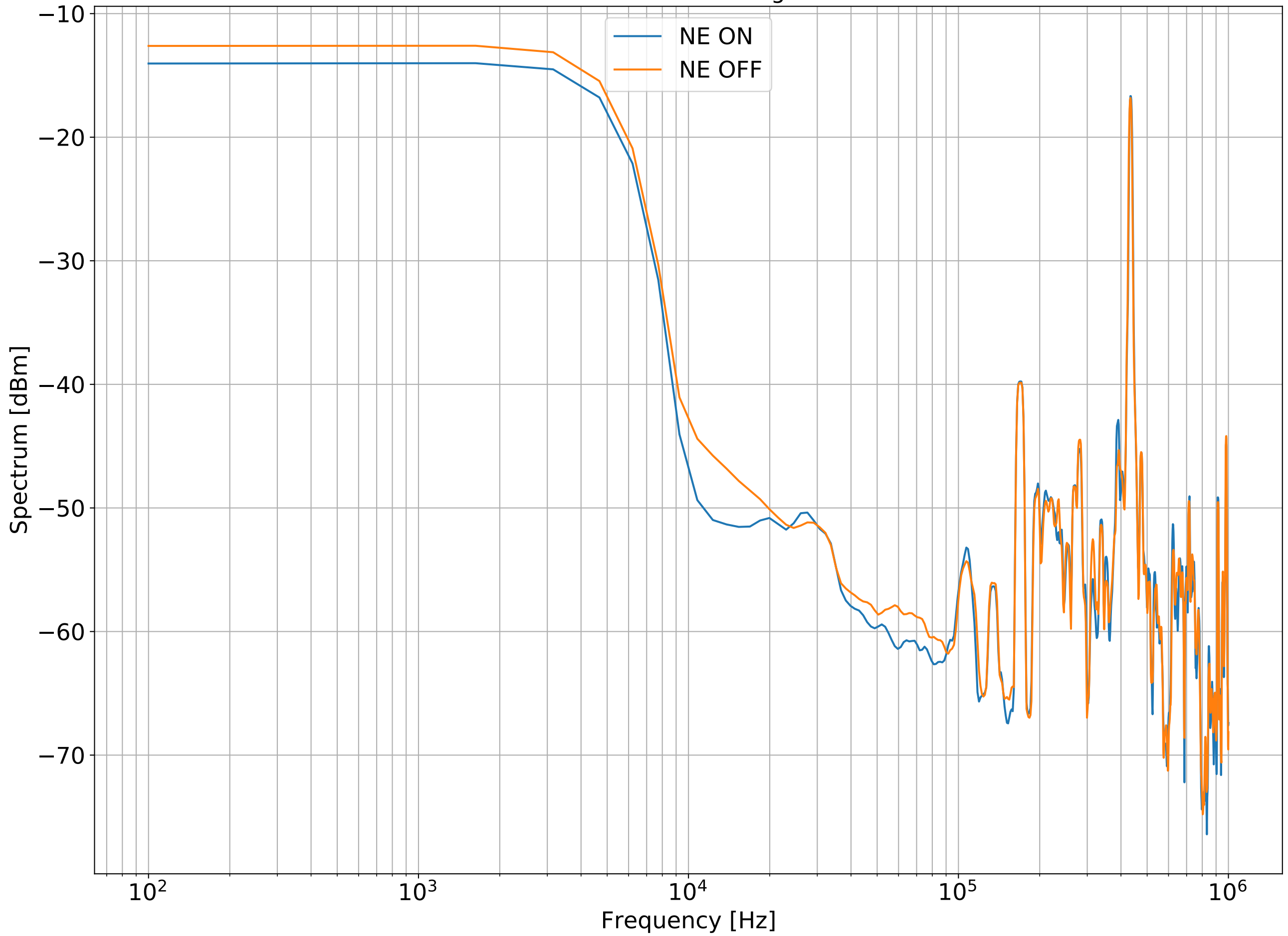
North PMC Error Signal
