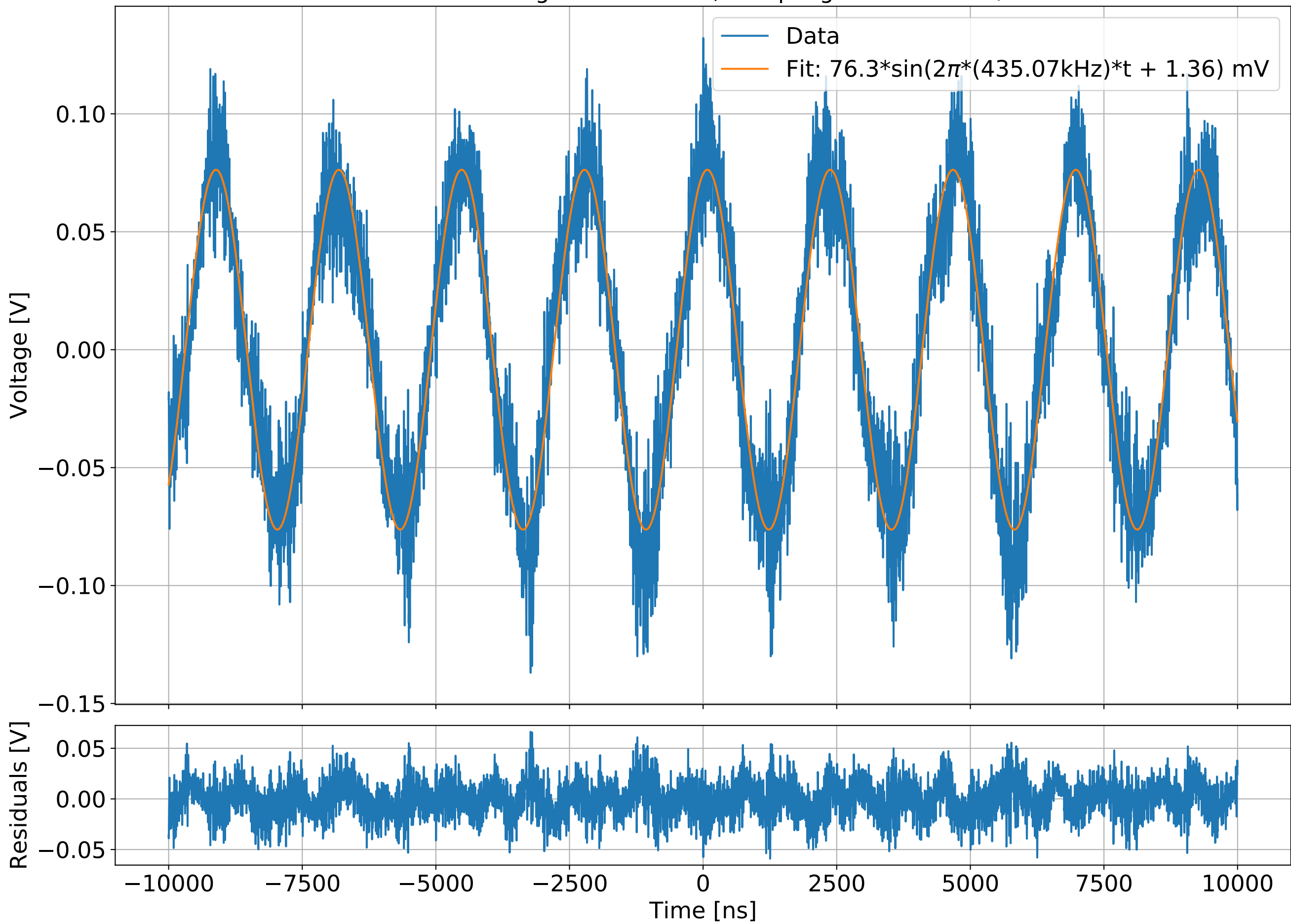
NFSS TP1 Trig Level 128 mV, Sampling Rate 0.5 GSa/s
