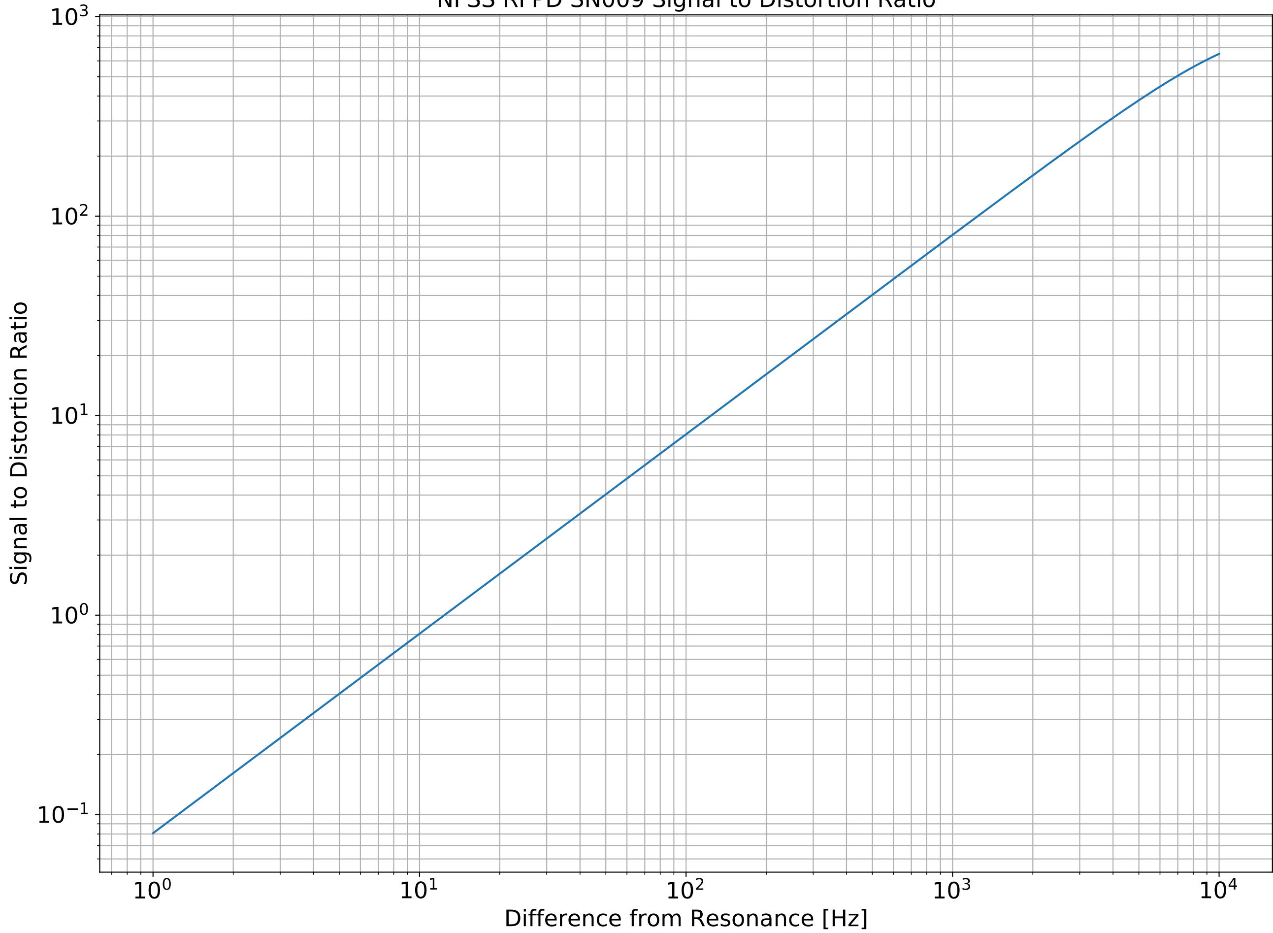
NFSS RFPD SN009 Signal to Distortion Ratio
