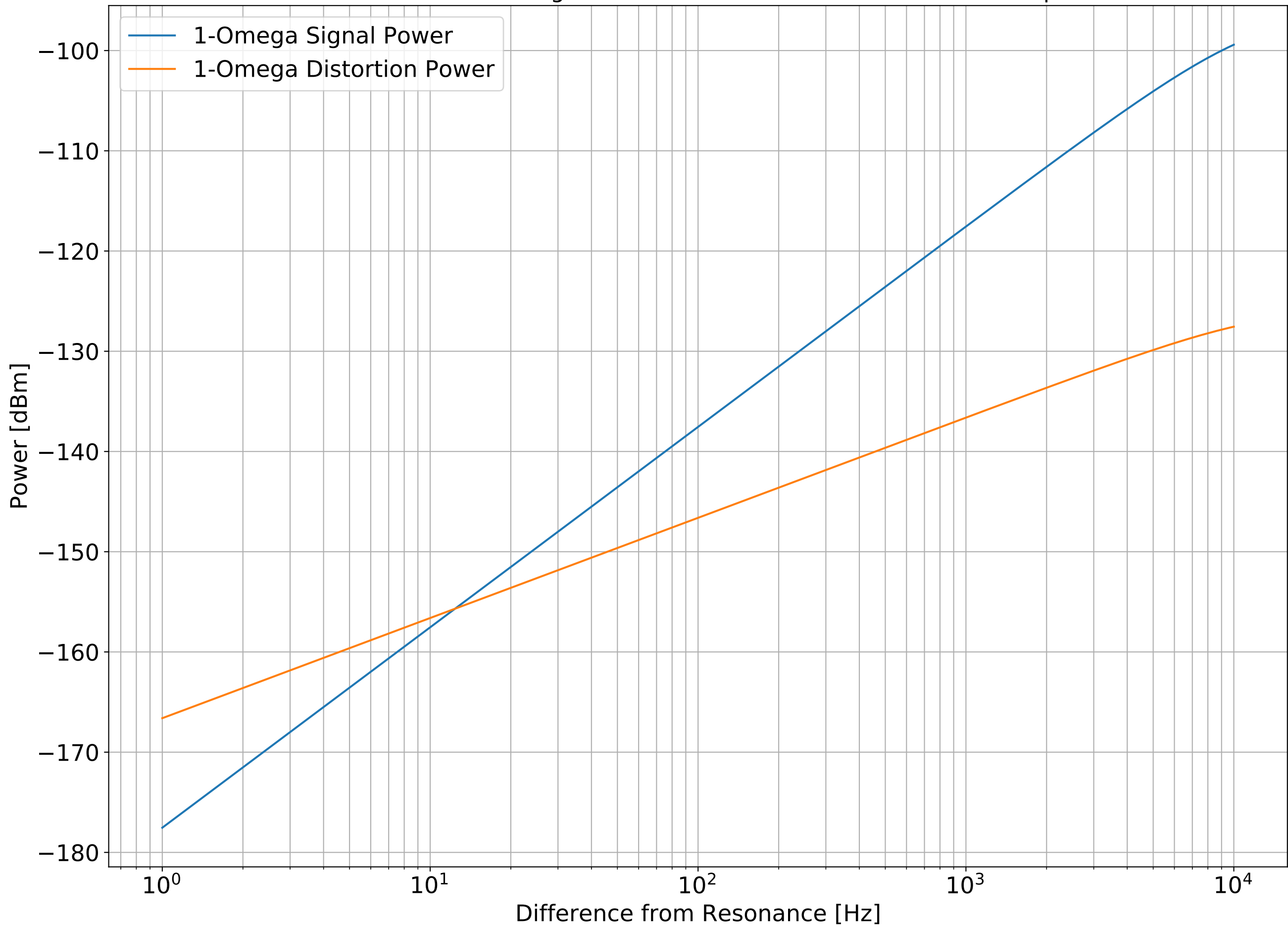
SFSS RFPD SN010 Signal and Distortion referred to MAX4107 input
