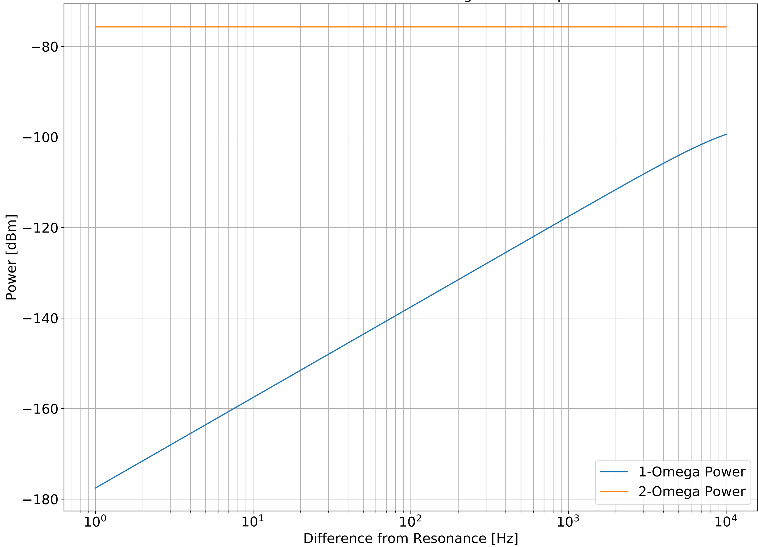
SFSS RFPD SN010 Power reaching MAX4107 input
