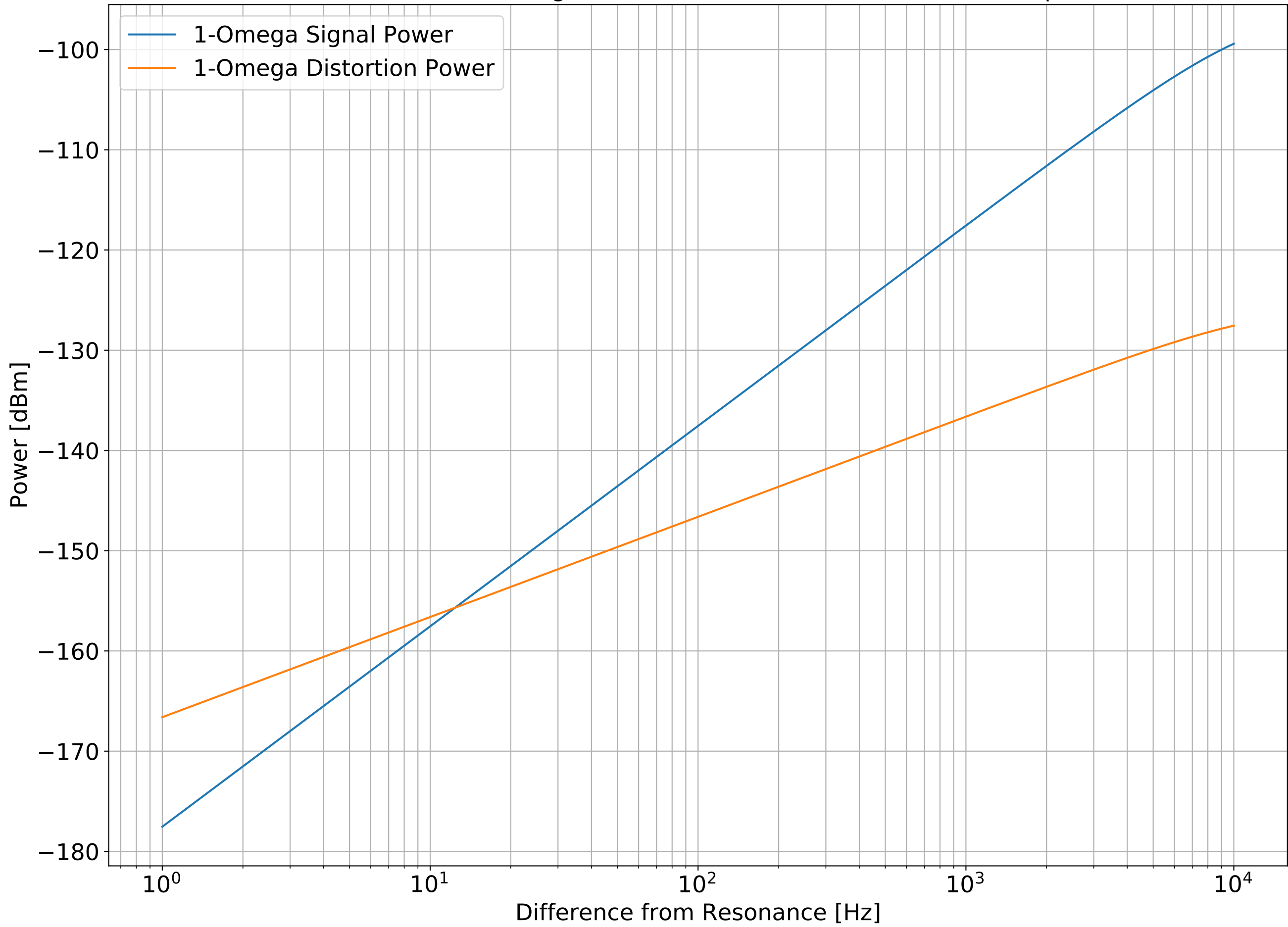
NFSS RFPD SN009 Signal and Distortion referred to MAX4107 input
