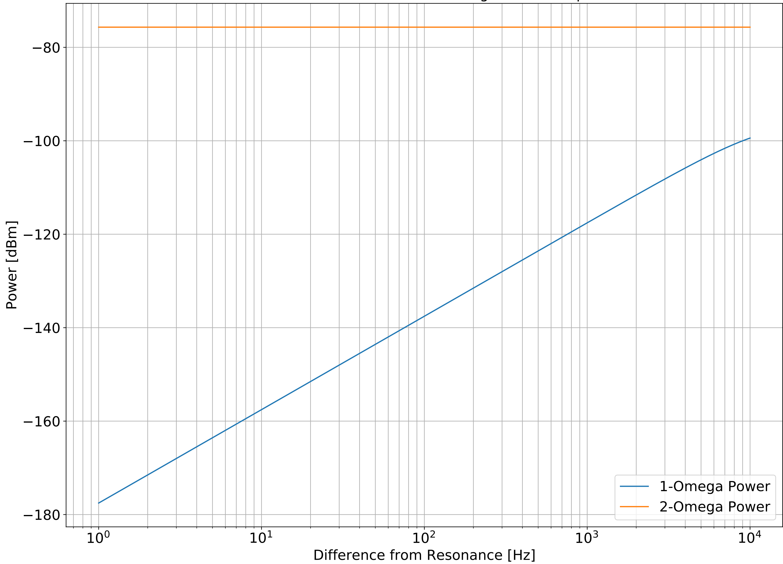
NFSS RFPD SN009 Power reaching MAX4107 input
