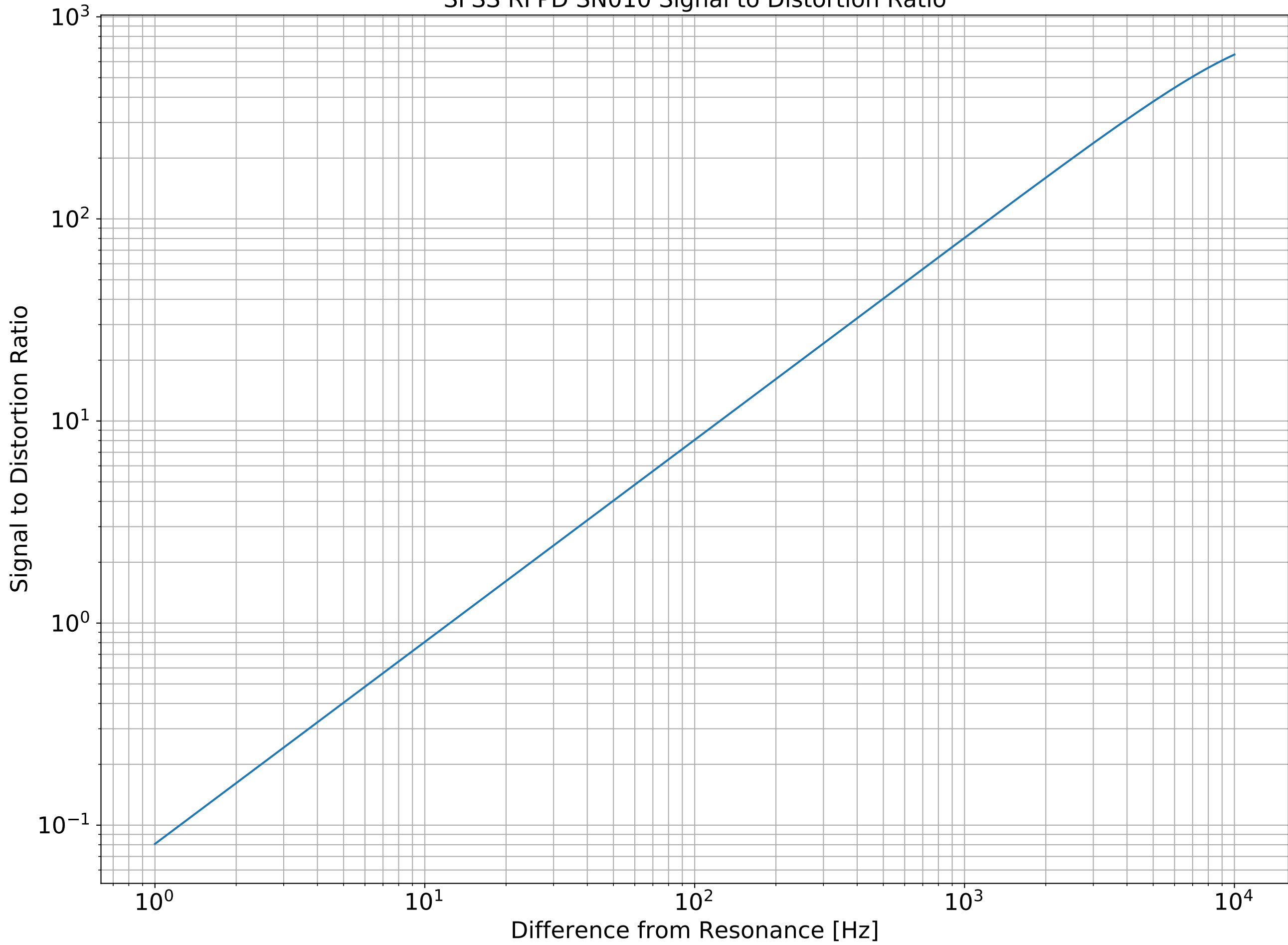
SFSS RFPD SN010 Signal to Distortion Ratio
