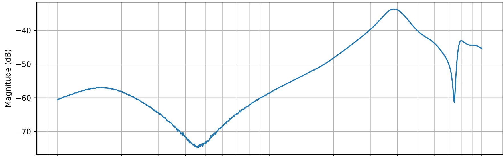
SFSS RFPD SN010 TF Measurement - Nov 11 2019 - 20:34:18
