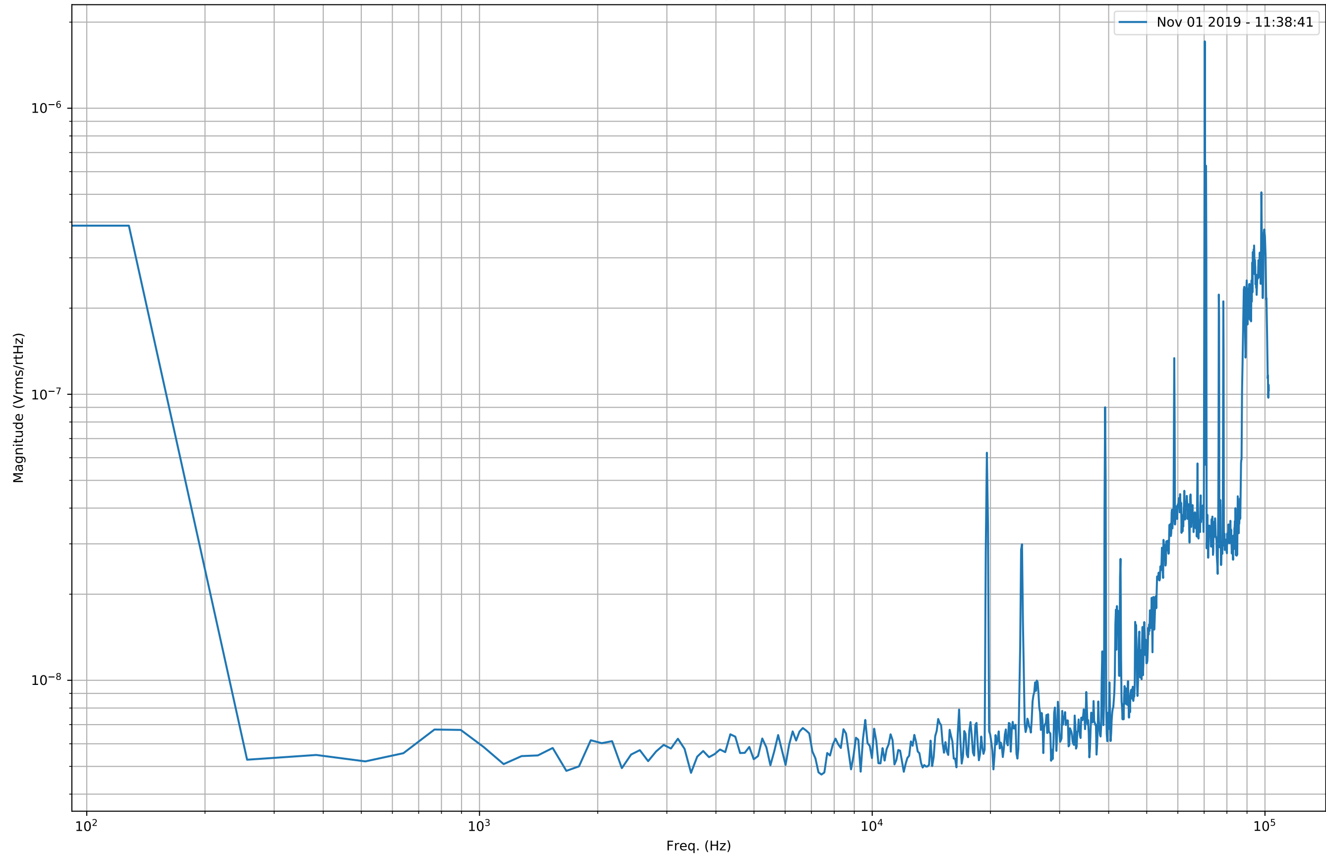
SFSS RFPD SN009 RF OUT 20dB Coupled - Nov 01 2019 - 11:39:06
