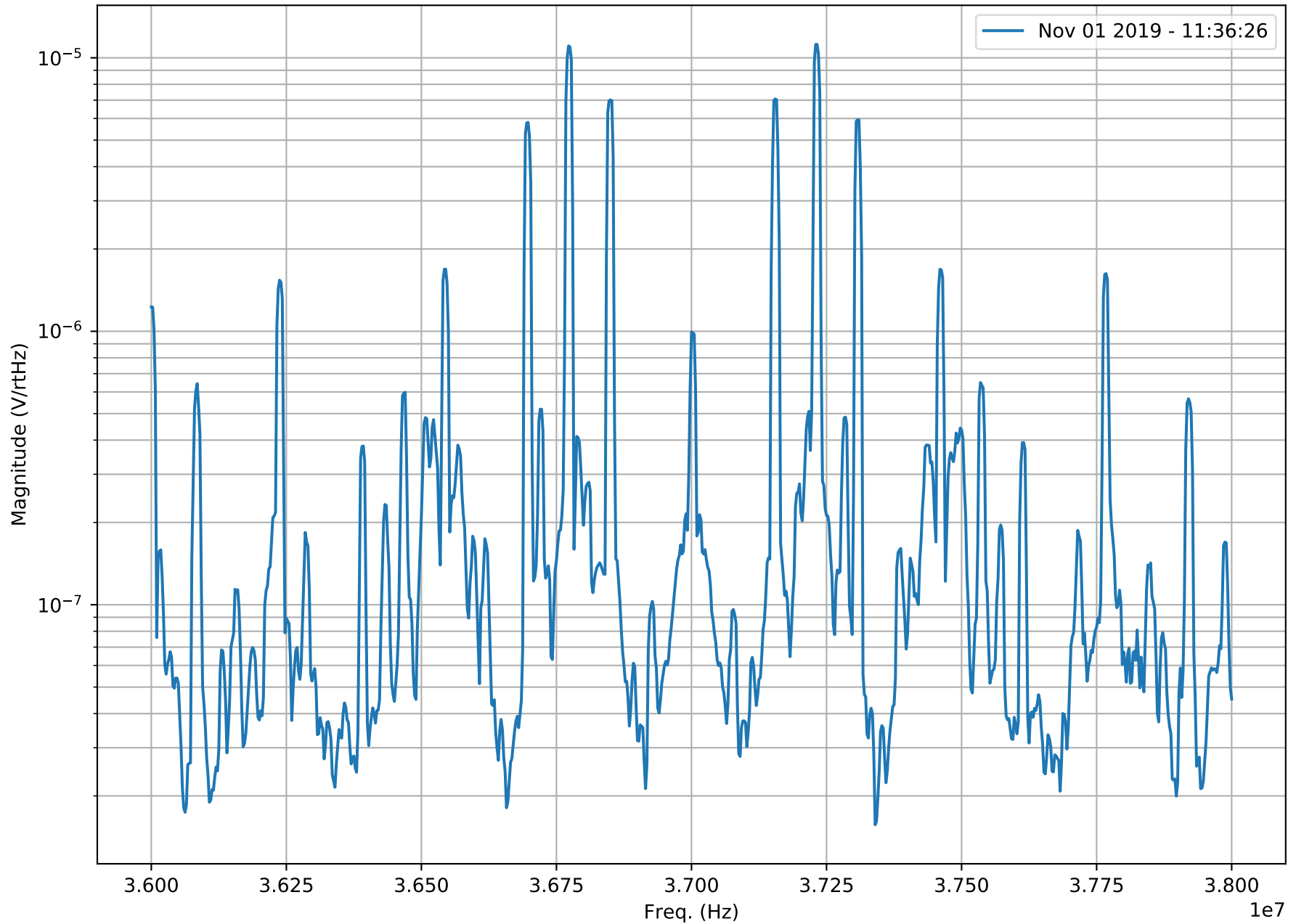
SFSS RFPD SN009 RF OUT 20dB Coupled - Nov 01 2019 - 11:37:13
