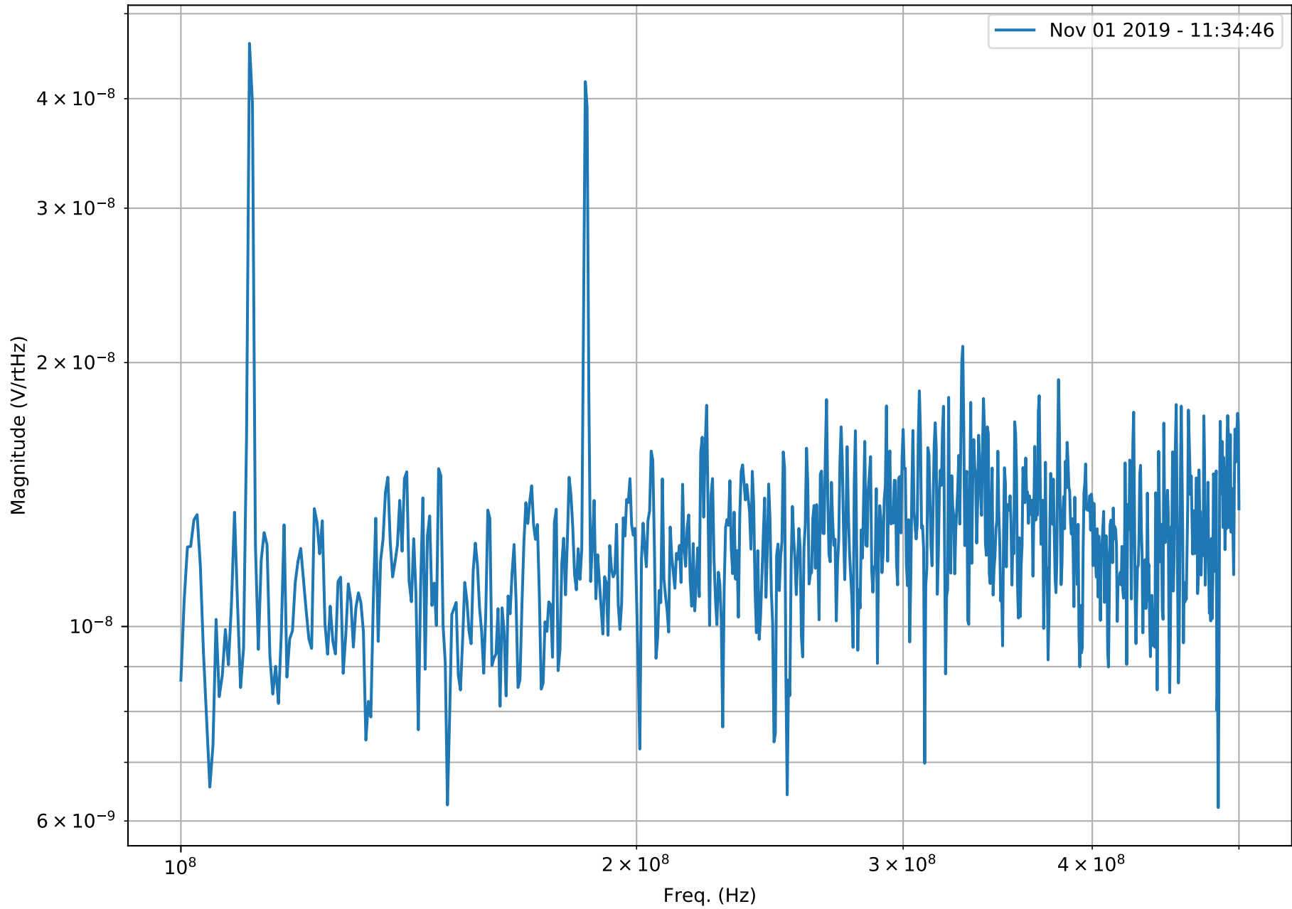
SFSS RFPD SN009 RF OUT 20dB Coupled - Nov 01 2019 - 11:35:33
