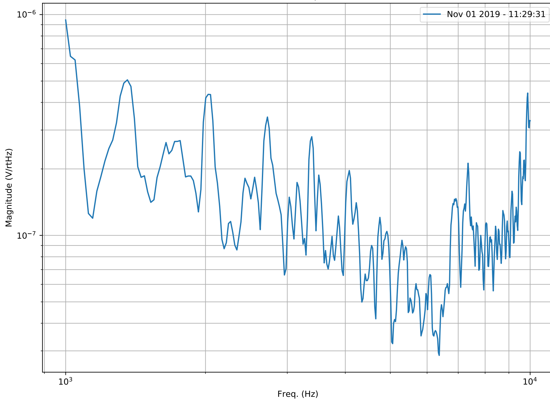
SFSS RFPD SN009 RF OUT 20dB Coupled - Nov 01 2019 - 11:30:11
