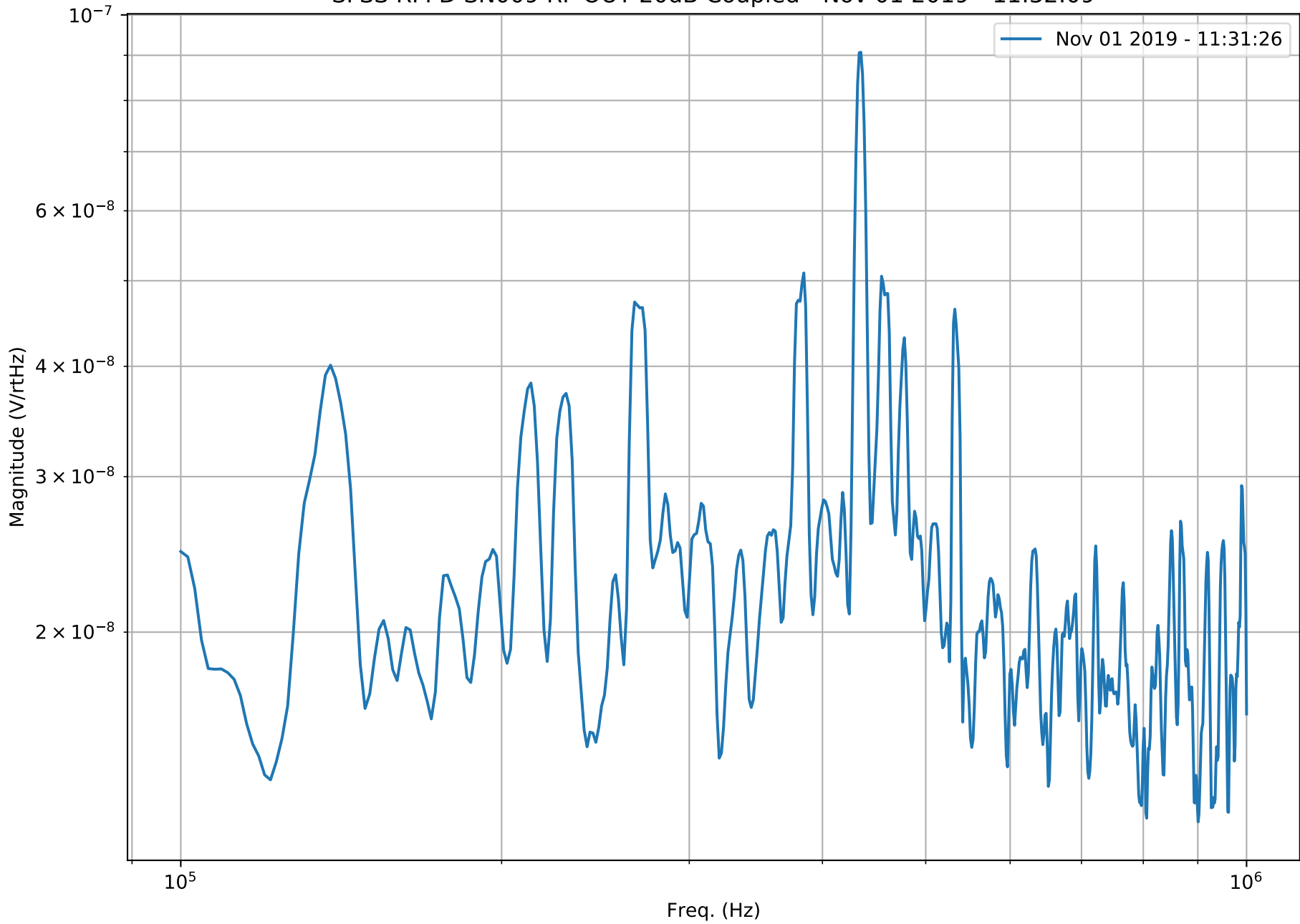
SFSS RFPD SN009 RF OUT 20dB Coupled - Nov 01 2019 - 11:32:09
