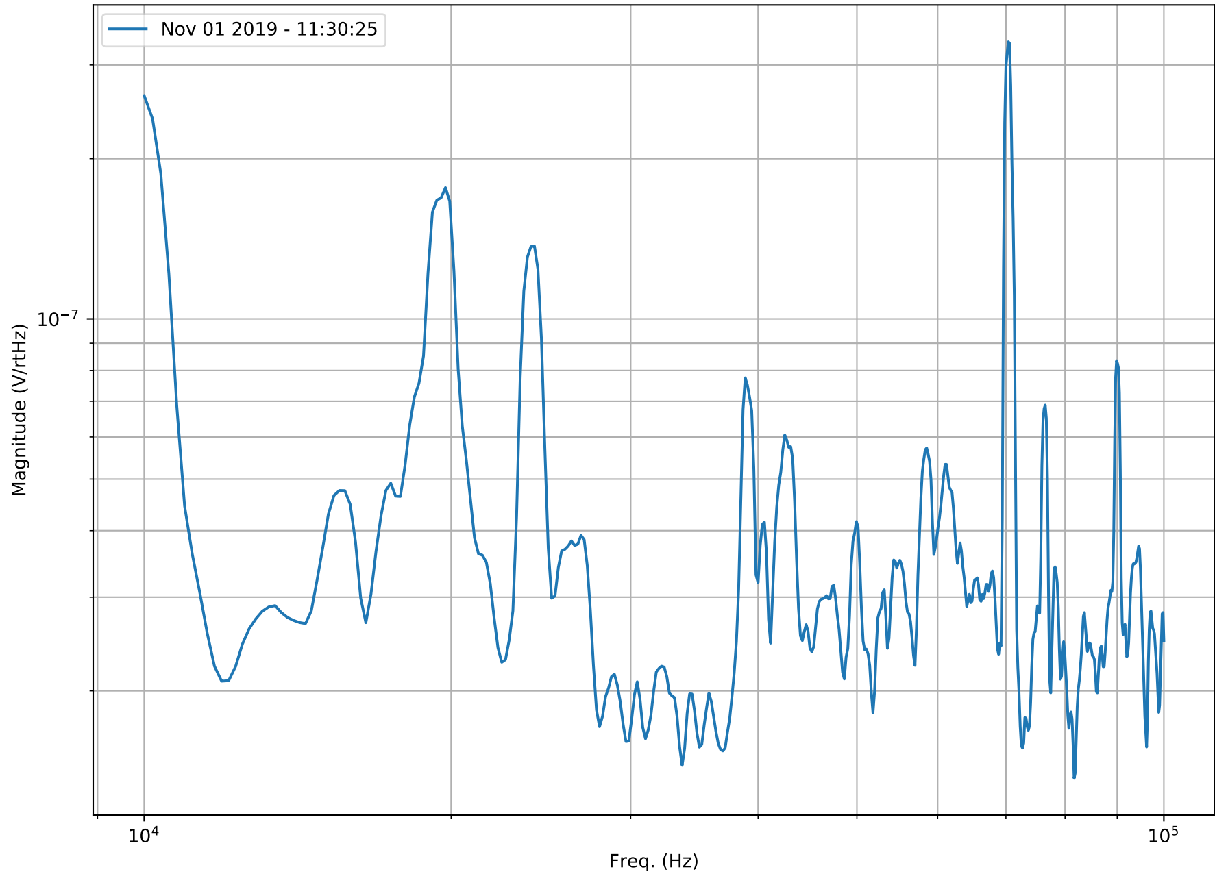
SFSS RFPD SN009 RF OUT 20dB Coupled - Nov 01 2019 - 11:31:07
