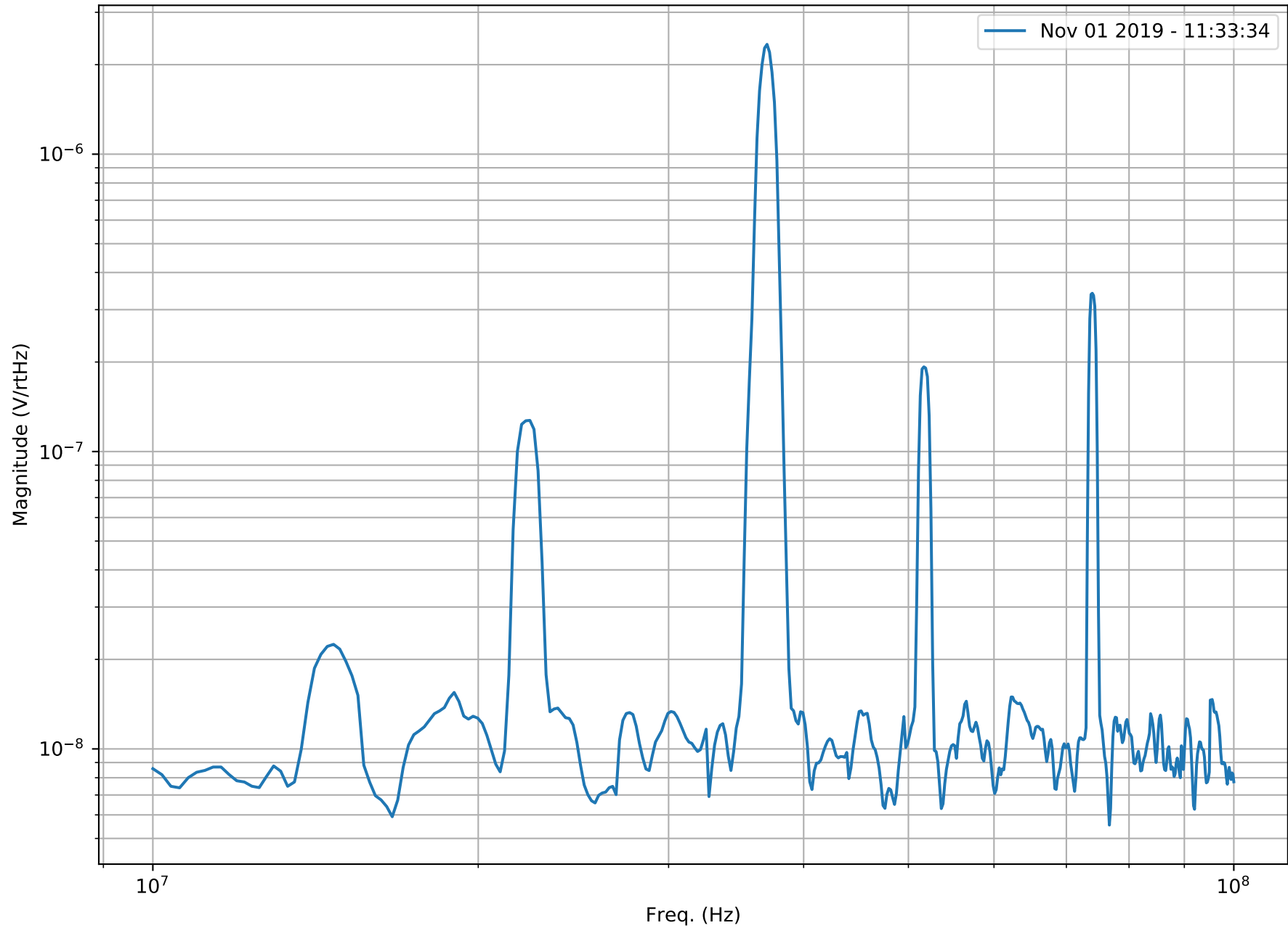
SFSS RFPD SN009 RF OUT 20dB Coupled - Nov 01 2019 - 11:34:15
