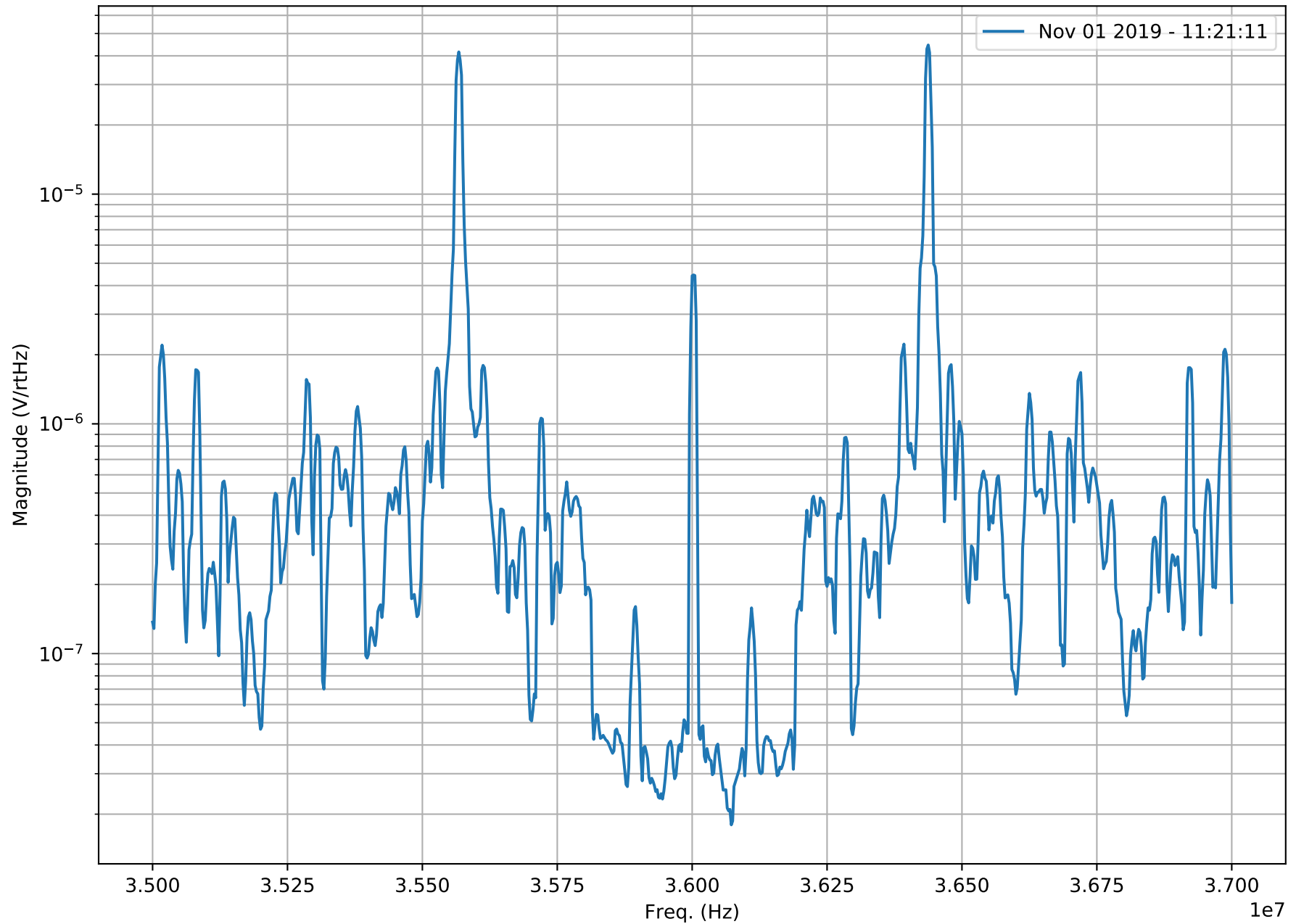
NFSS RFPD SN009 RF OUT 20dB Coupled - Nov 01 2019 - 11:21:58
