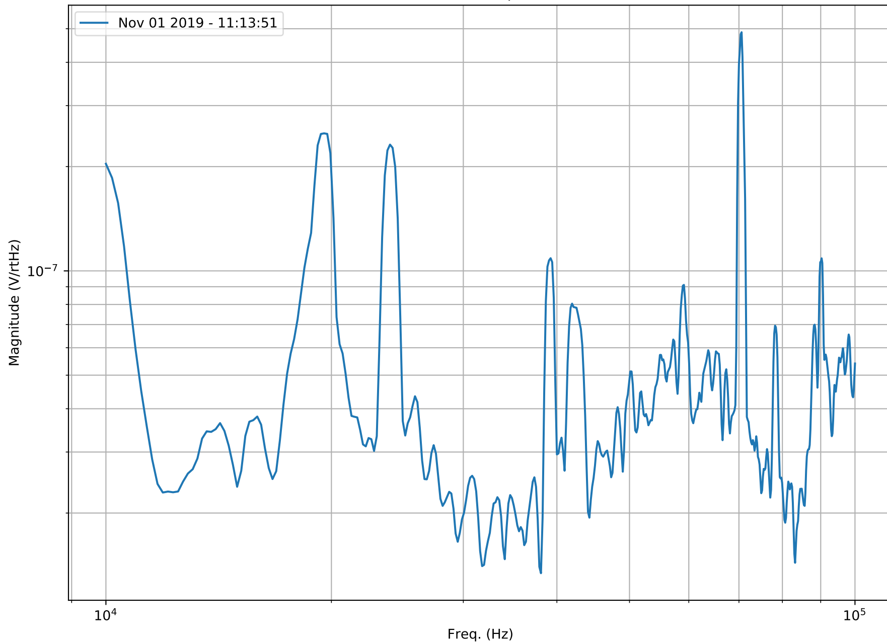
NFSS RFPD SN009 RF OUT 20dB Coupled - Nov 01 2019 - 11:14:33
