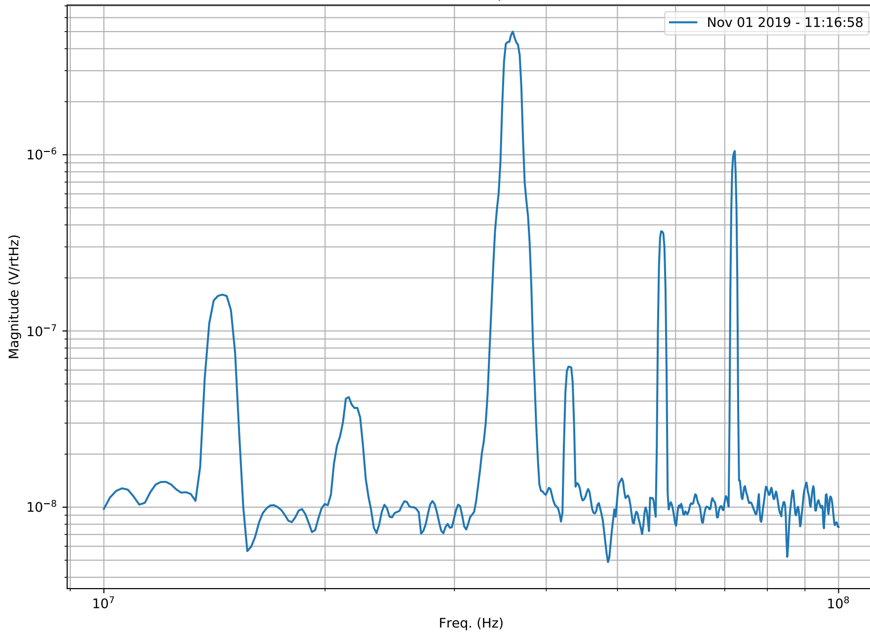
NFSS RFPD SN009 RF OUT 20dB Coupled - Nov 01 2019 - 11:17:38
