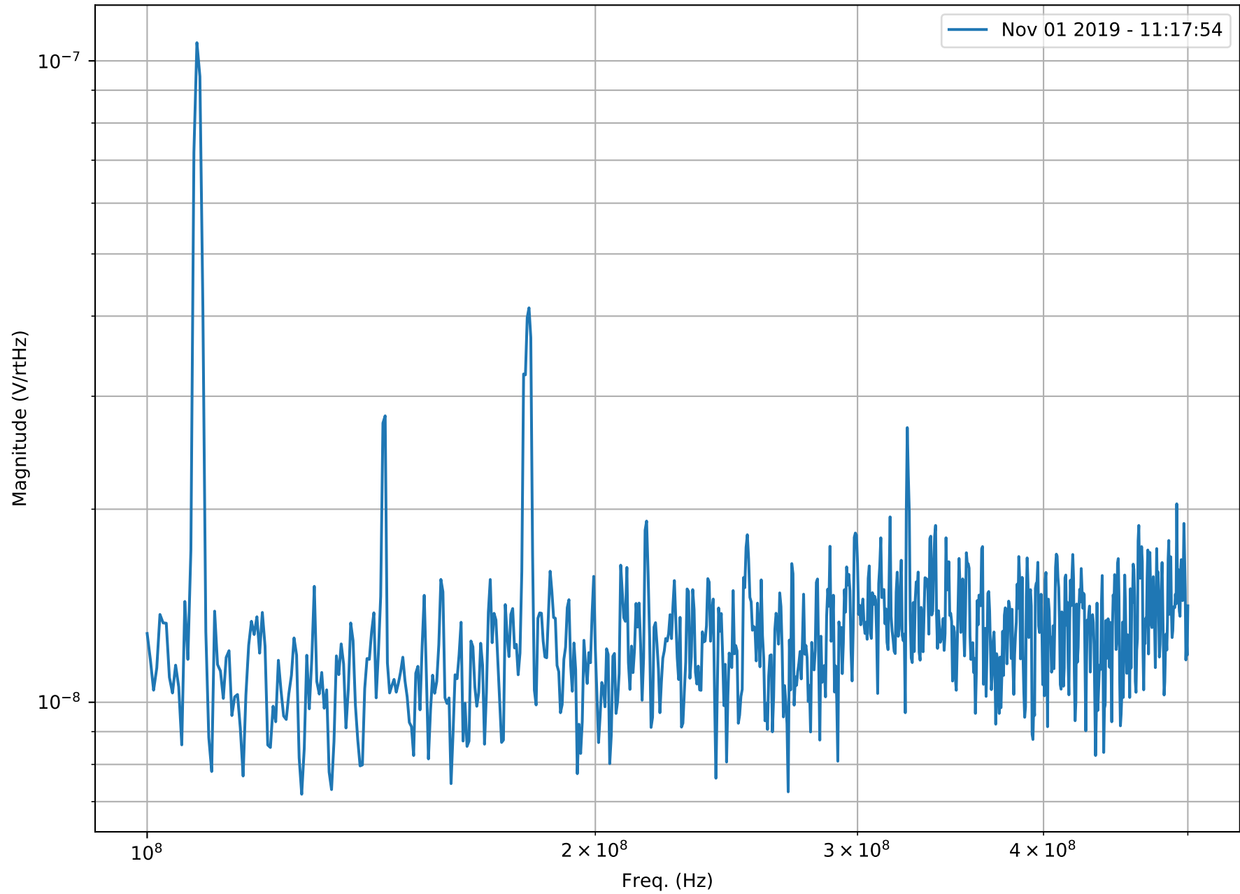
NFSS RFPD SN009 RF OUT 20dB Coupled - Nov 01 2019 - 11:18:41
