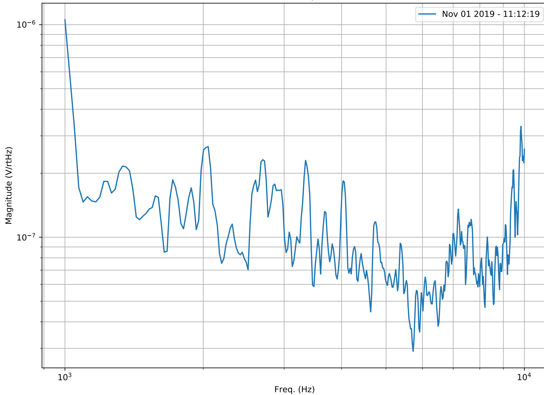
NFSS RFPD SN009 RF OUT 20dB Coupled - Nov 01 2019 - 11:12:59
