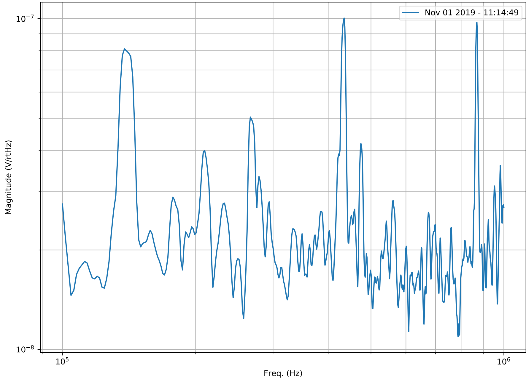
NFSS RFPD SN009 RF OUT 20dB Coupled - Nov 01 2019 - 11:15:32
