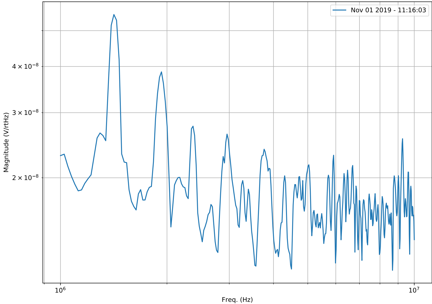
NFSS RFPD SN009 RF OUT 20dB Coupled - Nov 01 2019 - 11:16:42
