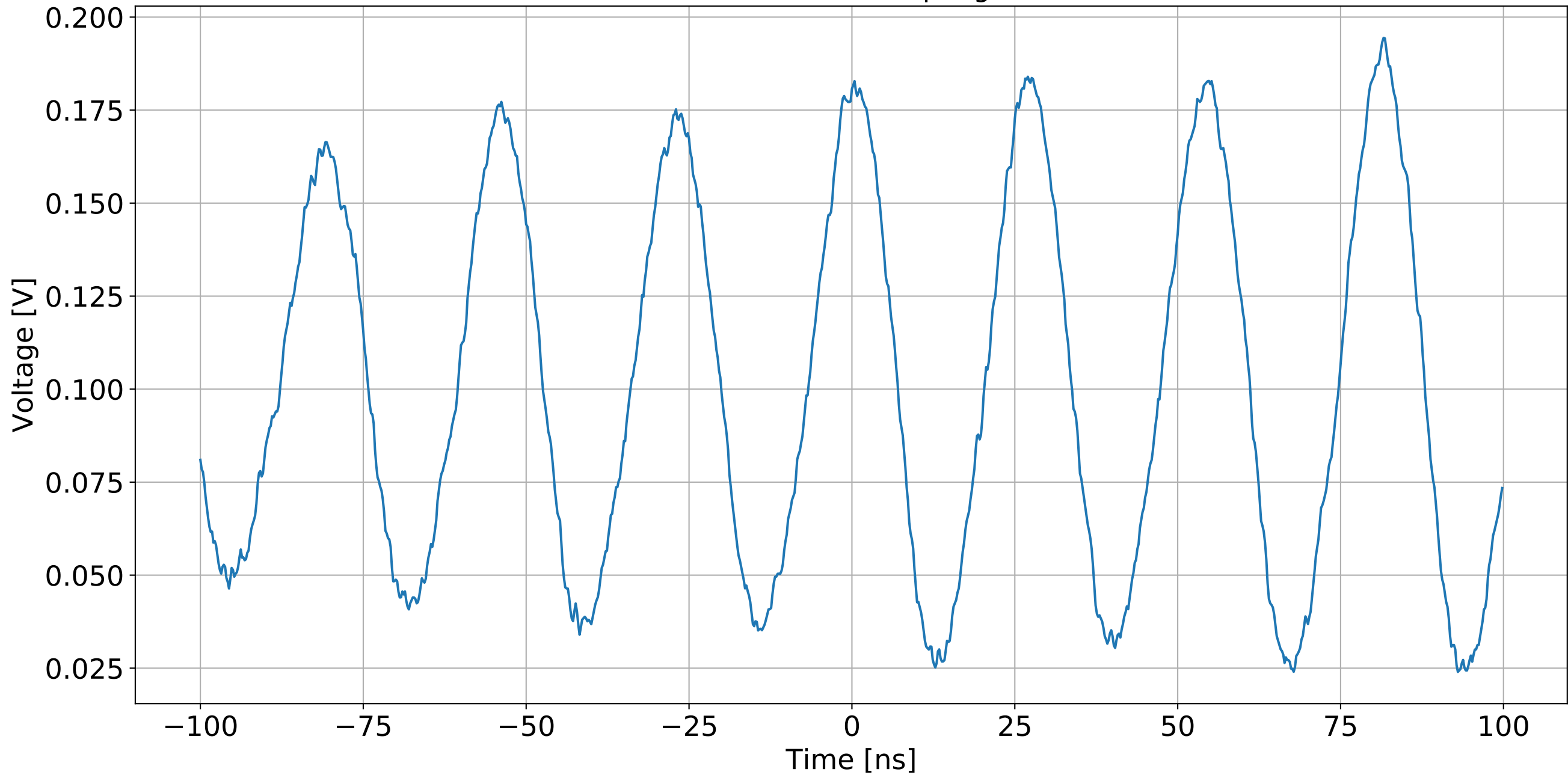
SFSS RFPD SN010 RF Out, Sampling Rate 5.0 GSa/s
