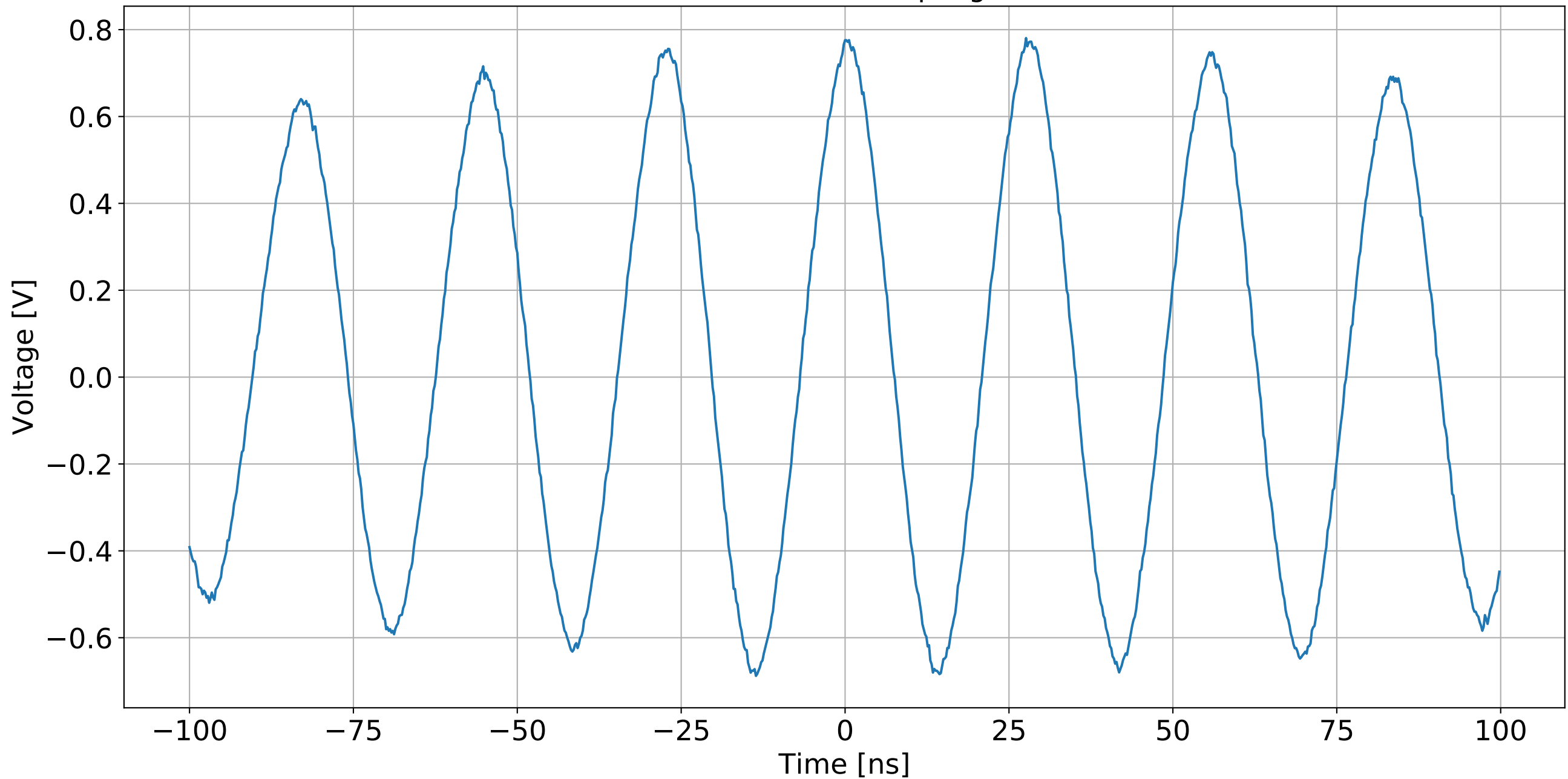
NFSS RFPD SN009 RF Out, Sampling Rate 5.0 GSa/s
