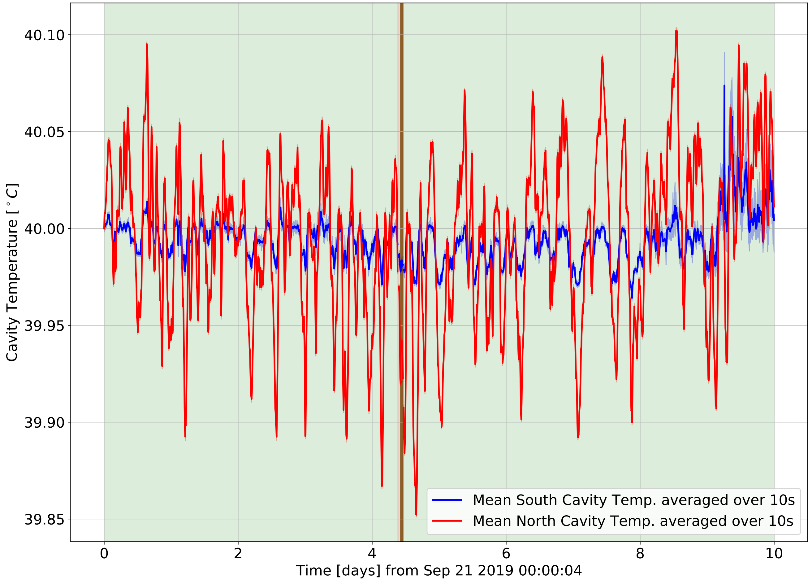
Cavity Temperatures from Sep 21 2019 00:00:04 to Sep 30 2019 23:59:44 Offset Adjusted to start at 40 ° C
