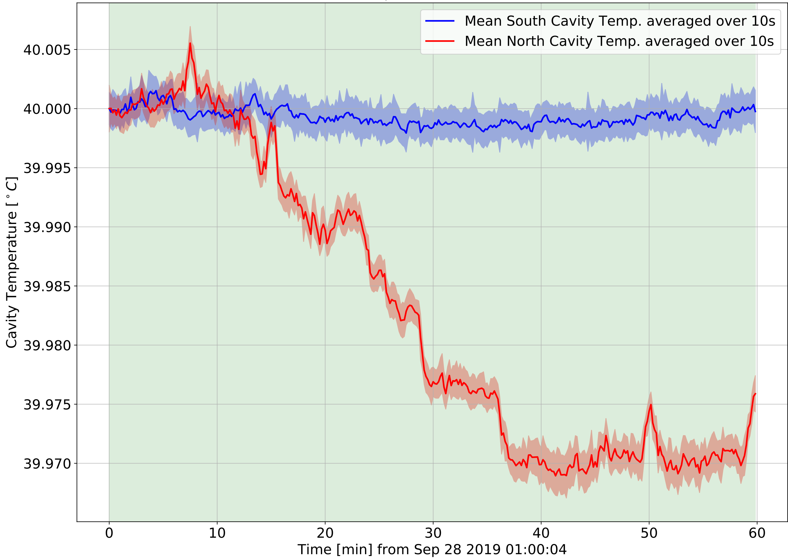
Cavity Temperatures from Sep 28 2019 01:00:04 to Sep 28 2019 01:59:54 Offset Adjusted to start at 40 °C
