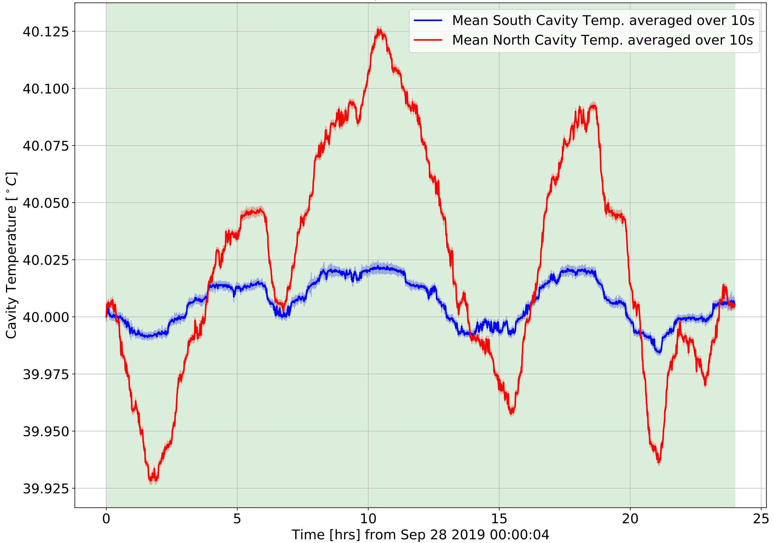
Cavity Temperatures from Sep 28 2019 00:00:04 to Sep 28 2019 23:59:54 Offset Adjusted to start at 40 ° C
