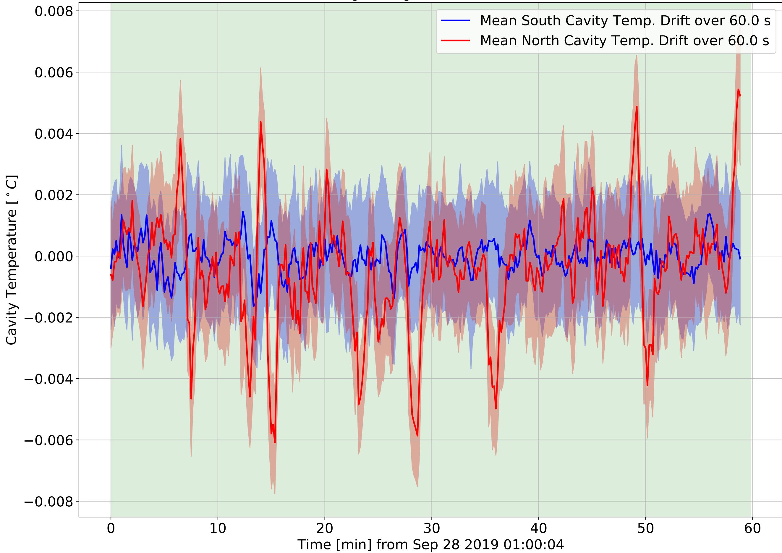
Cavity Temp Drift from Sep 28 2019 01:00:04 to Sep 28 2019 01:59:54 (Using averaged values over 10s)
