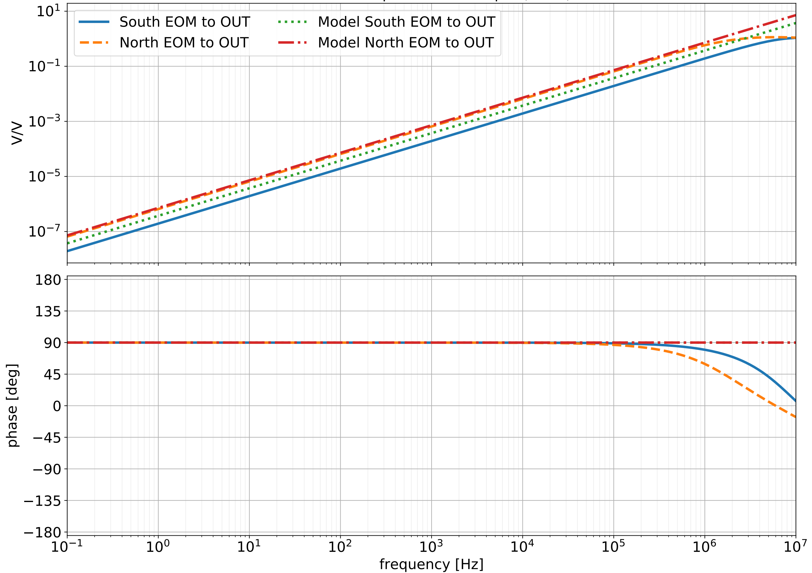
Ideal Model Transfer function vs Circuit Transfer Function for FSS Plant From EOM input to Plant Output (to PD)
