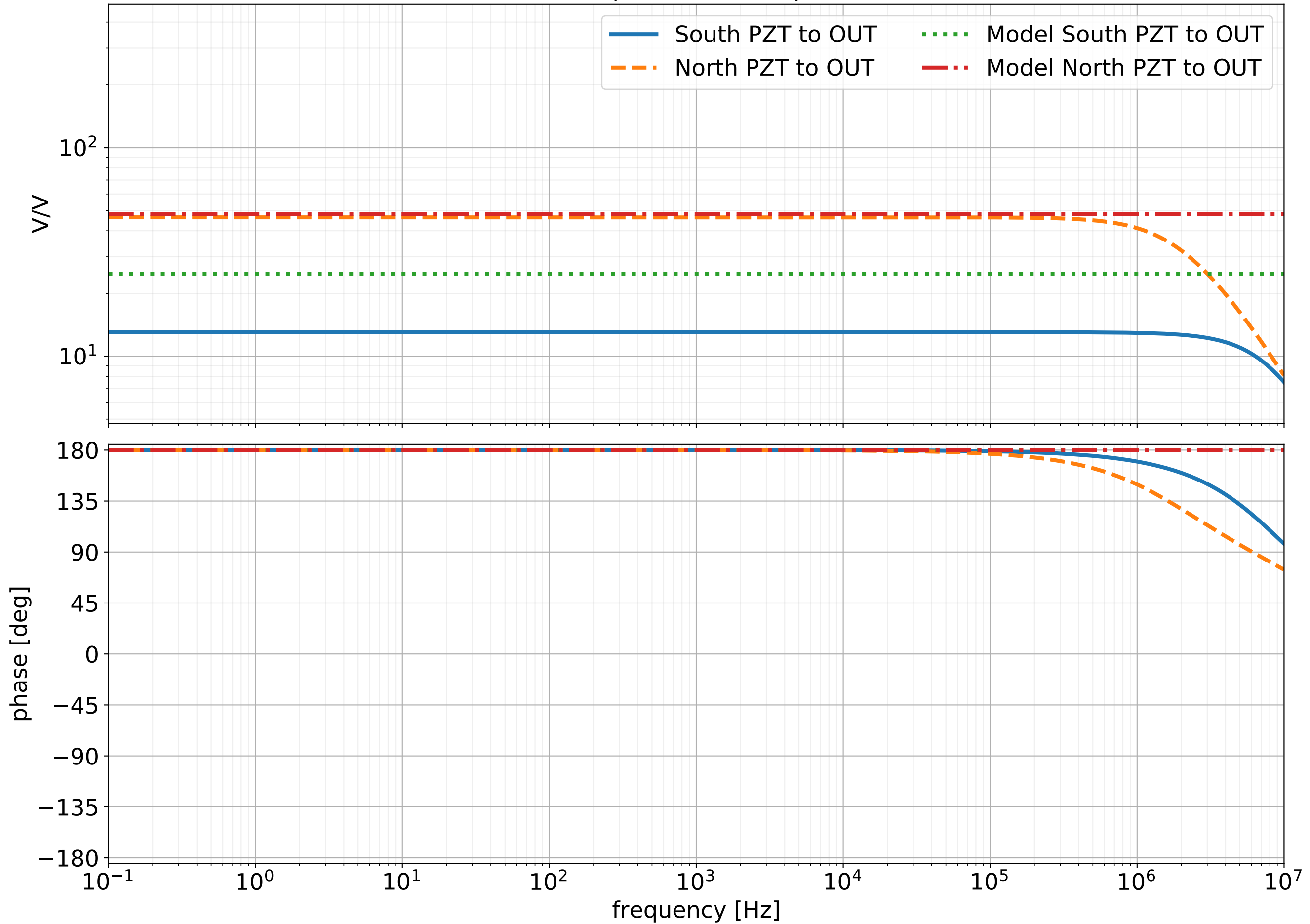
Ideal Model Transfer function vs Circuit Transfer Function for FSS Plant From PZT input to Plant Output (to PD)
