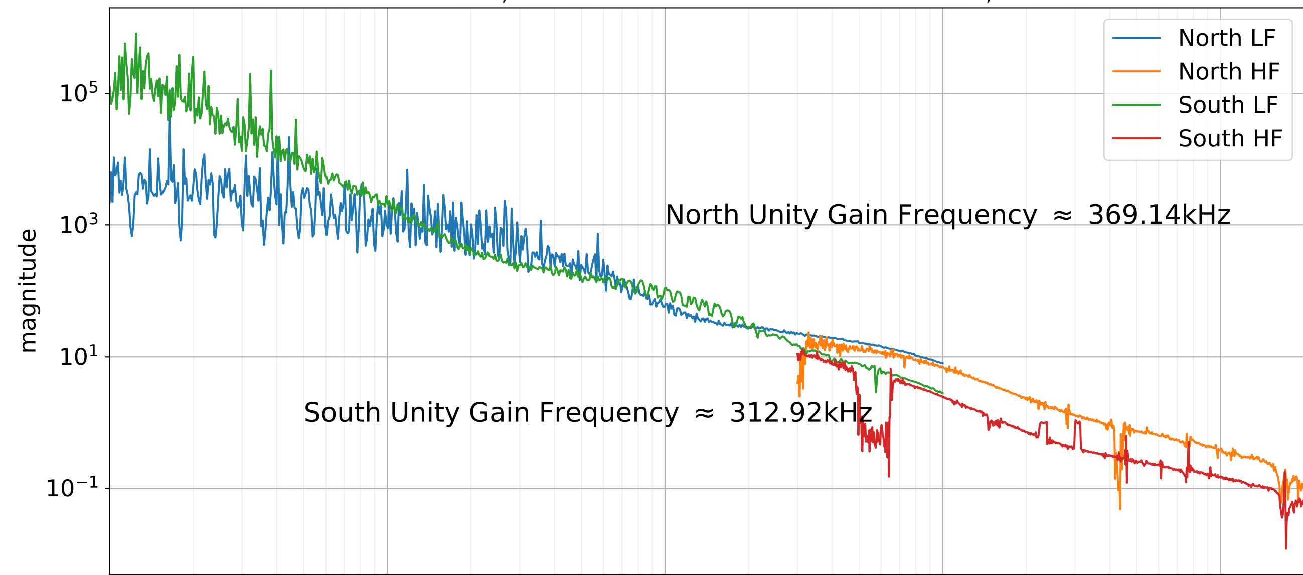
FSS Open Loop Gains - Boost On South: COMGain=10dB, FastGain=14dB North:COMGain=10dB, FASTGain=10dB
