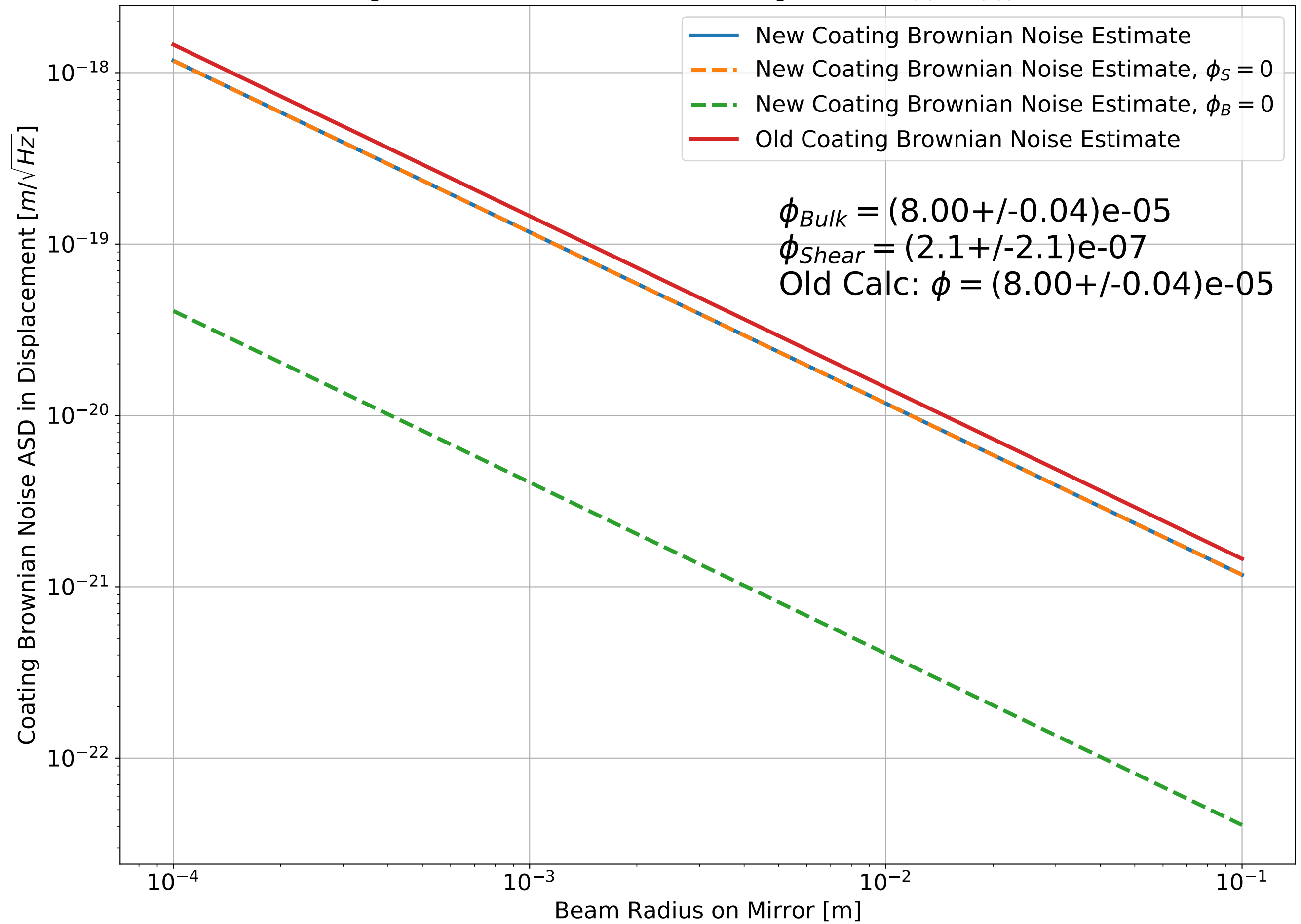
Coating Brownian Noise Estimate for a single GaAs, Al_{0.92}Ga_{0.08}As mirror
