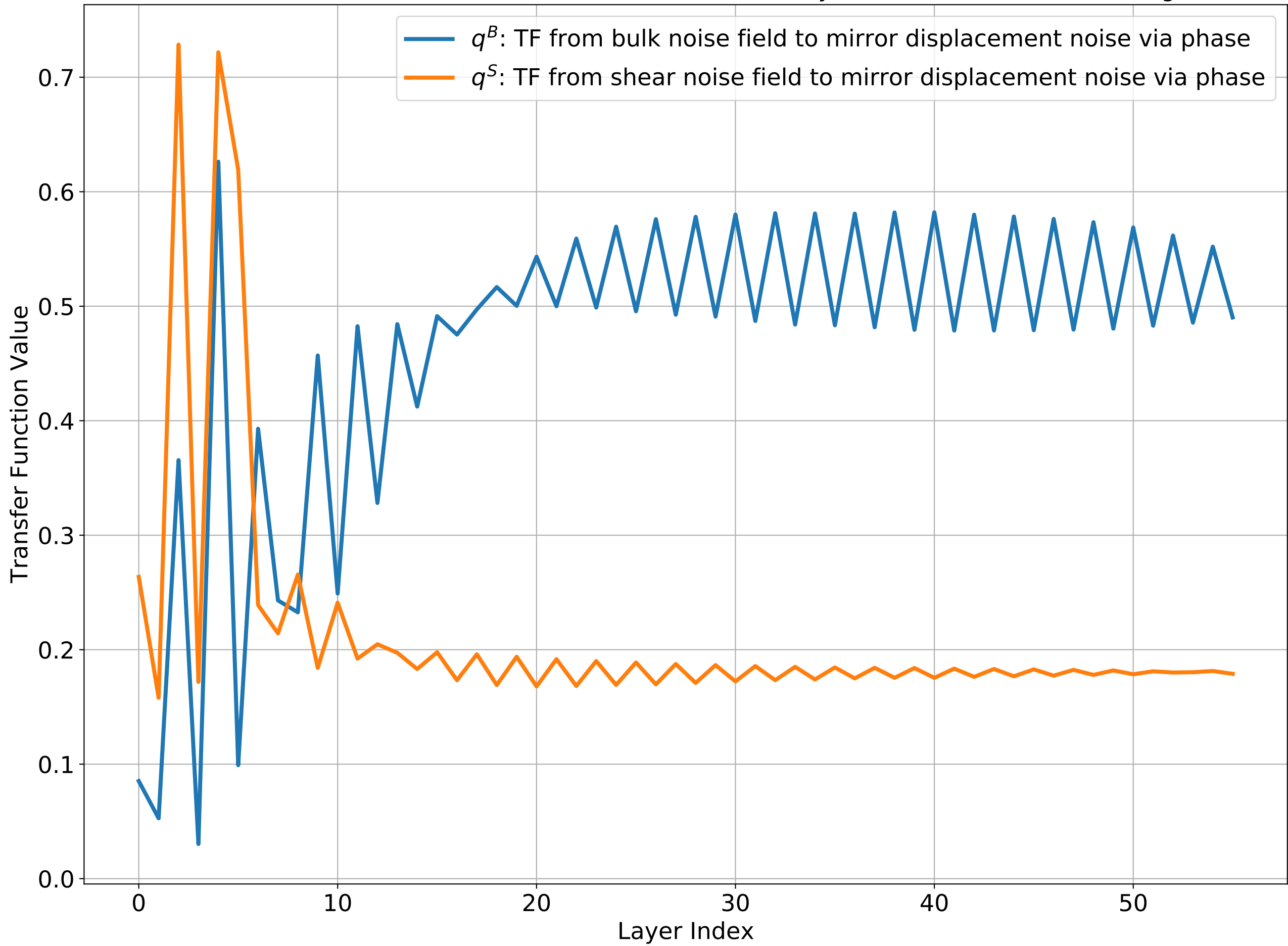
Transfer functions from bulk and shear noise fieldsto layer thickness and surface height
