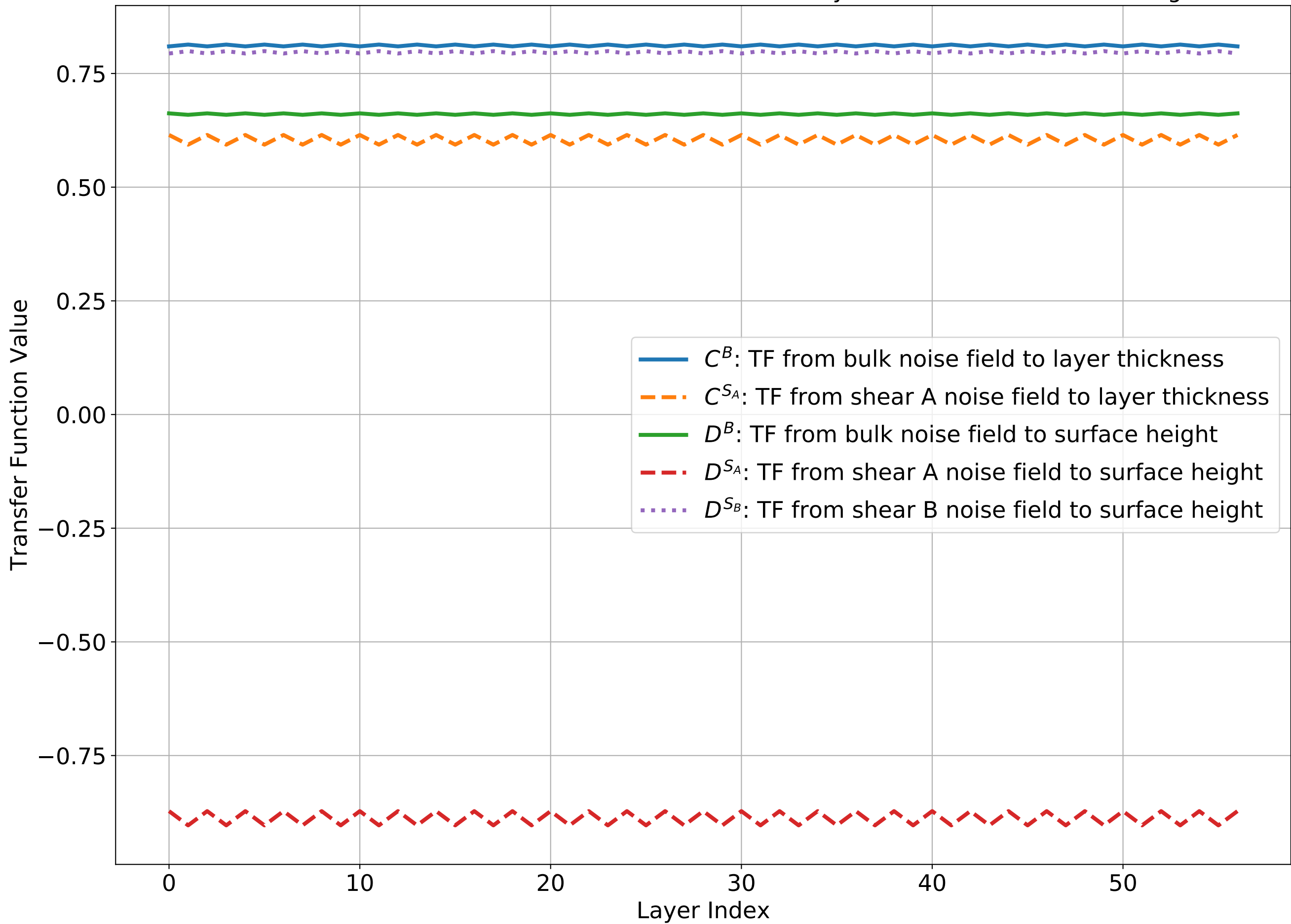
Transfer functions from bulk and shear noise fieldsto layer thickness and surface height
