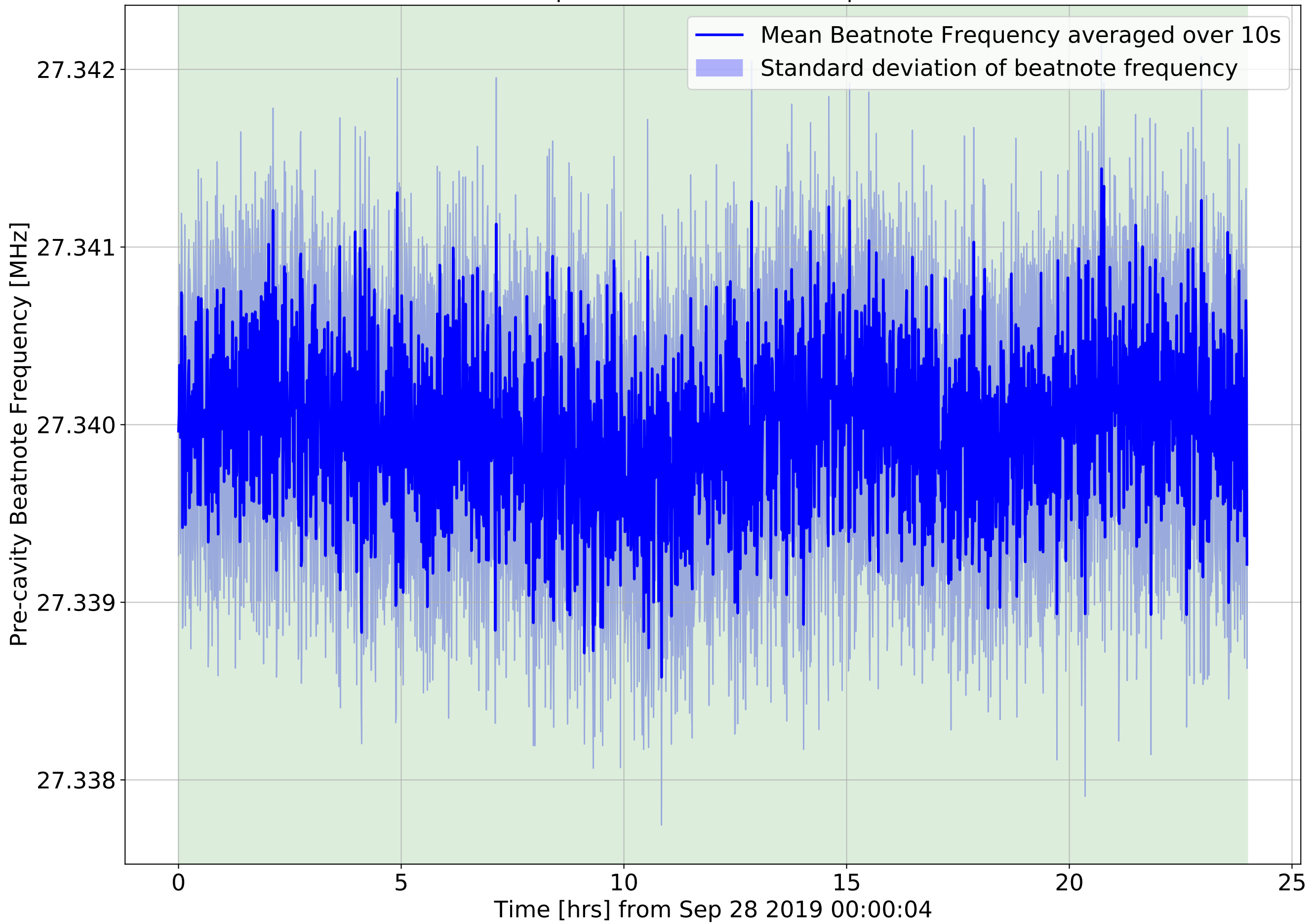
Beatnote from Sep 28 2019 00:00:04 to Sep 28 2019 23:59:54
