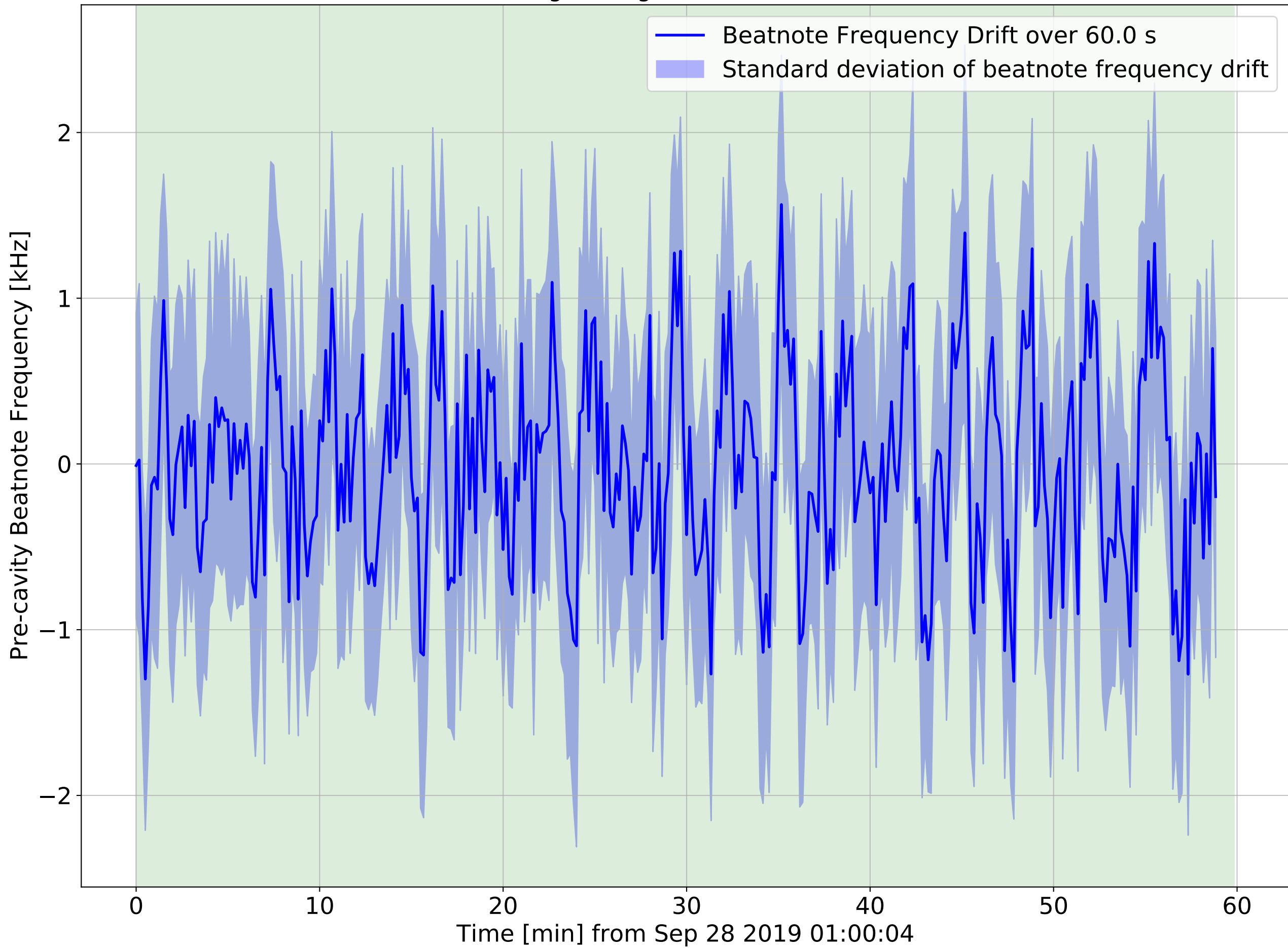
Beatnote Drift from Sep 28 2019 01:00:04 to Sep 28 2019 01:59:54 (Using averaged values over 10s)
