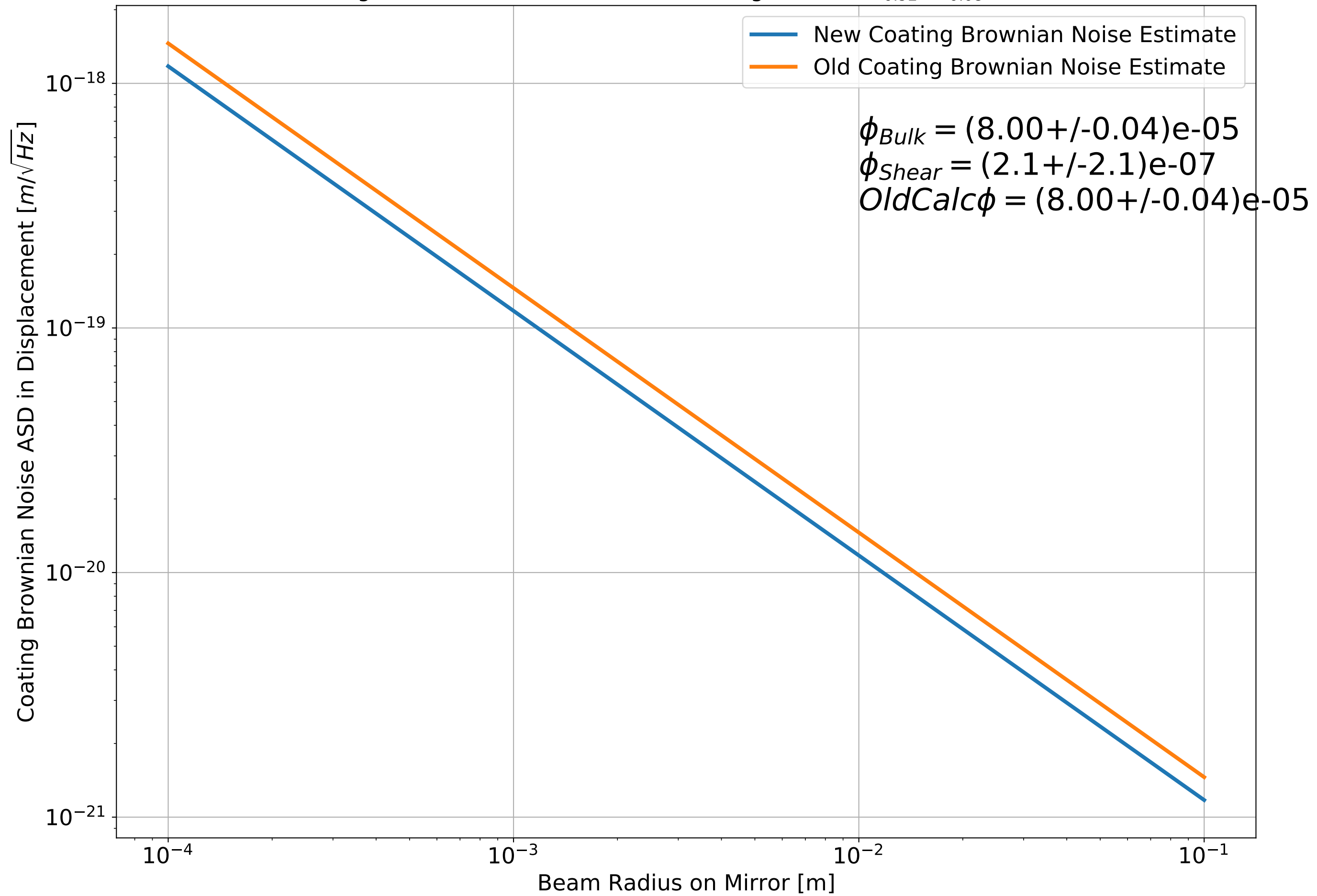
Coating Brownian Noise Estimate for a single GaAs, Al_{0.92}Ga_{0.08}As mirror
