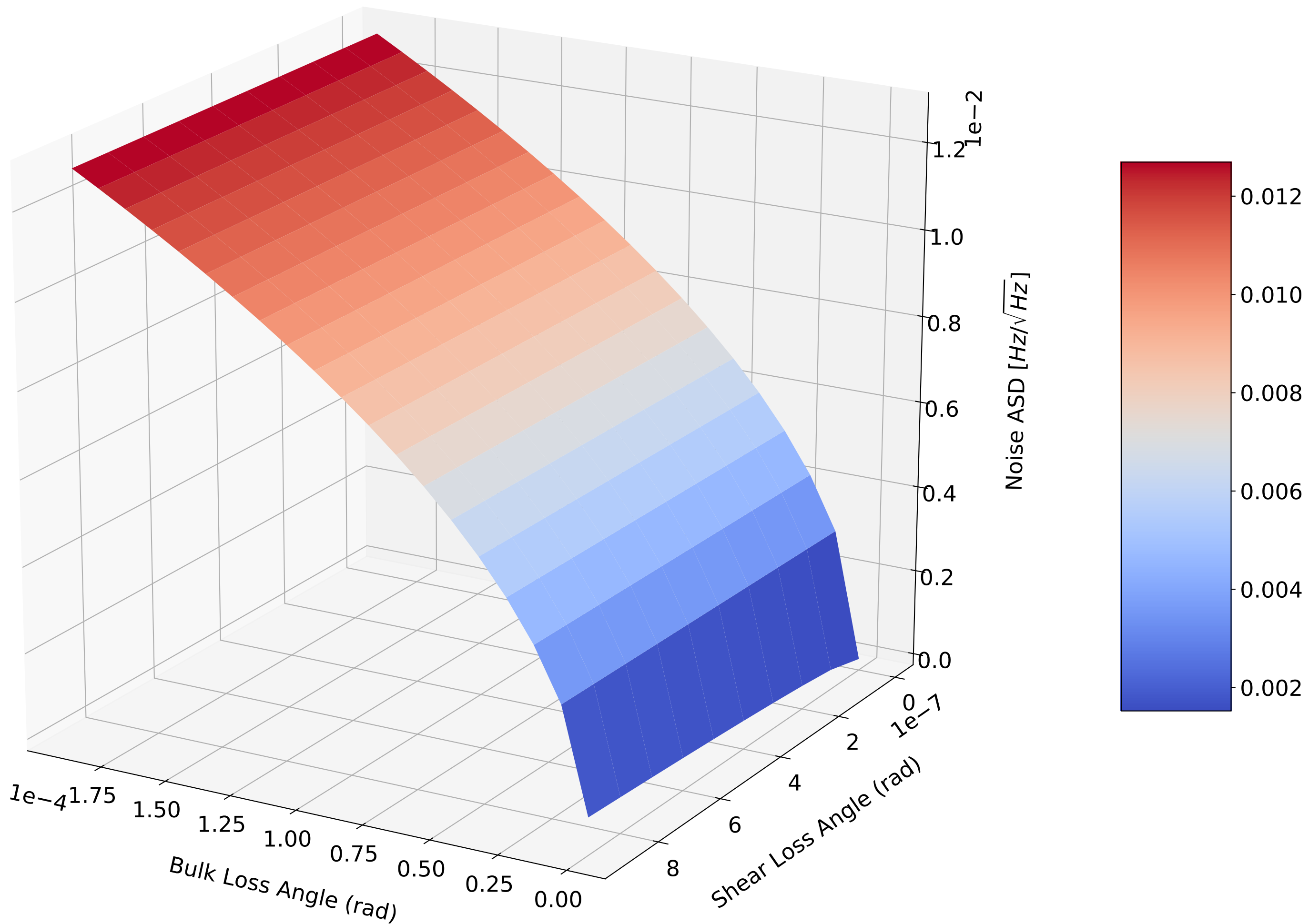
Expected Coating Brownian Noise ASD at 300 Hz For different Bulk and Shear Loss Angles
