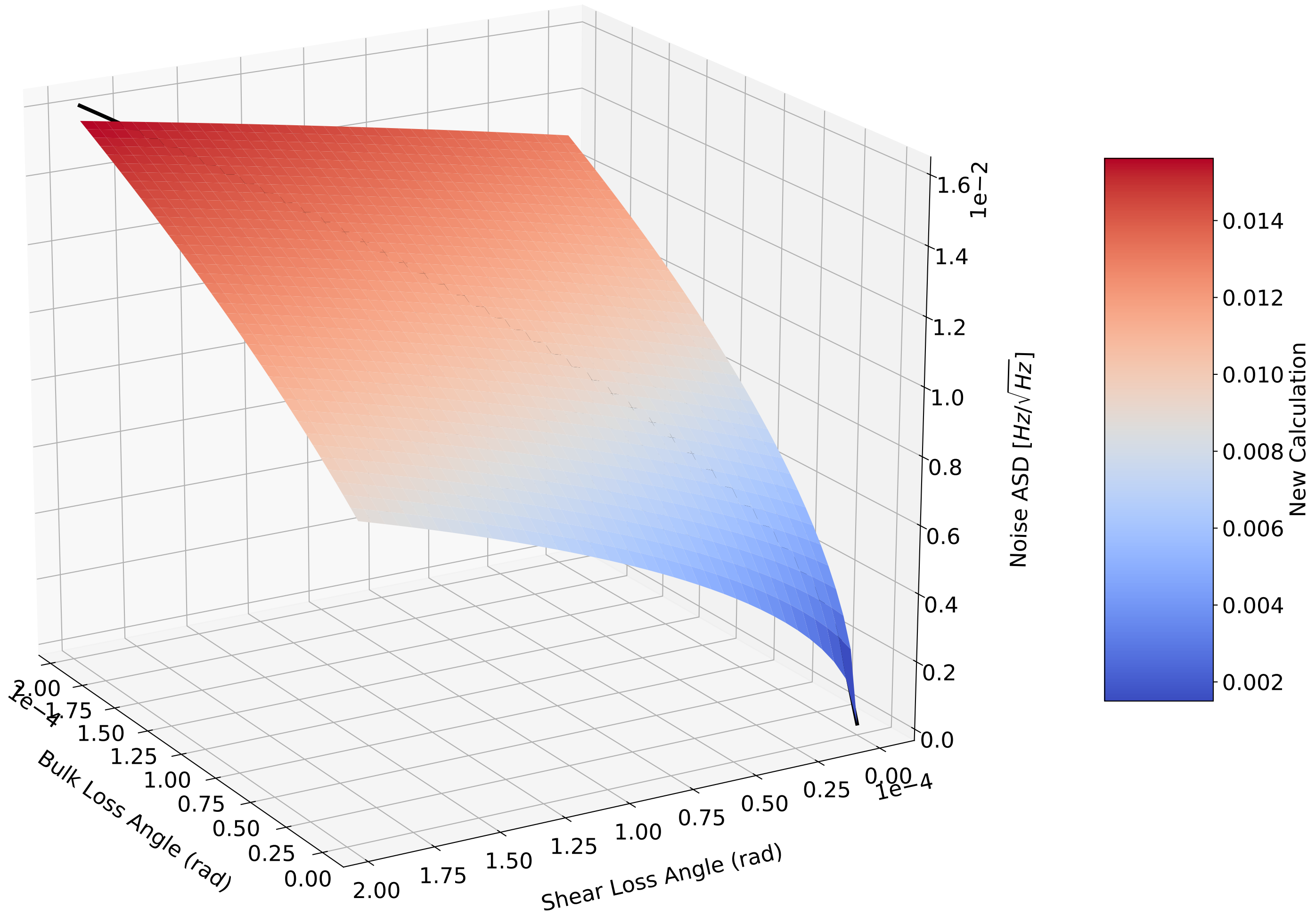
Expected Coating Brownian Noise ASD at 300 Hz For different Bulk and Shear Loss Angles Compared with old calculation
