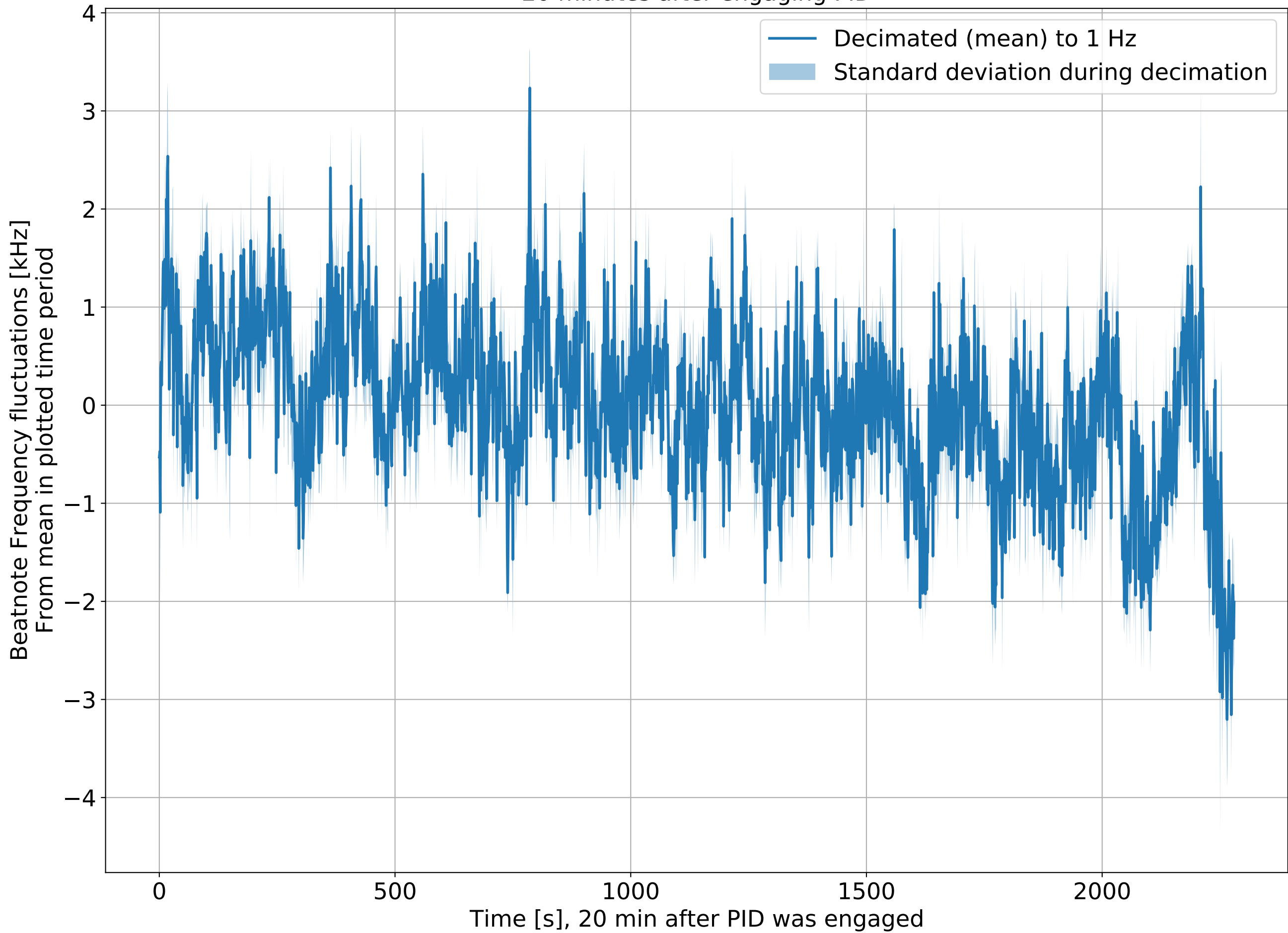
CTN Beatnote frequency stabilization 20 minutes after engaging PID
