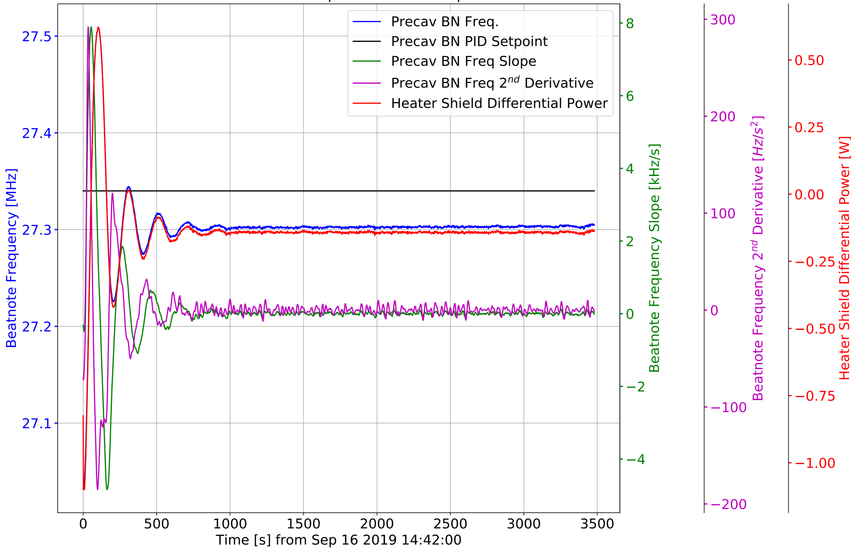
CTN beatnote PID control performance on Sep 16 2019
