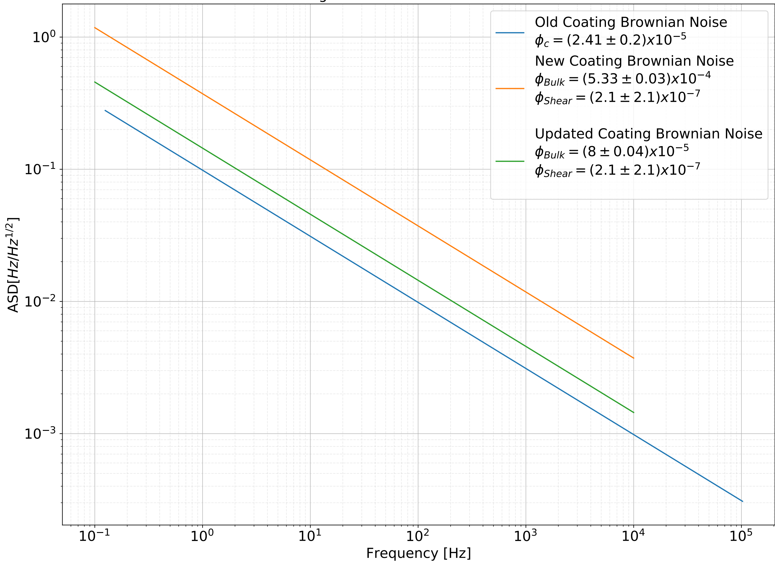
Coating Brownian Noise in CTN at Caltech
