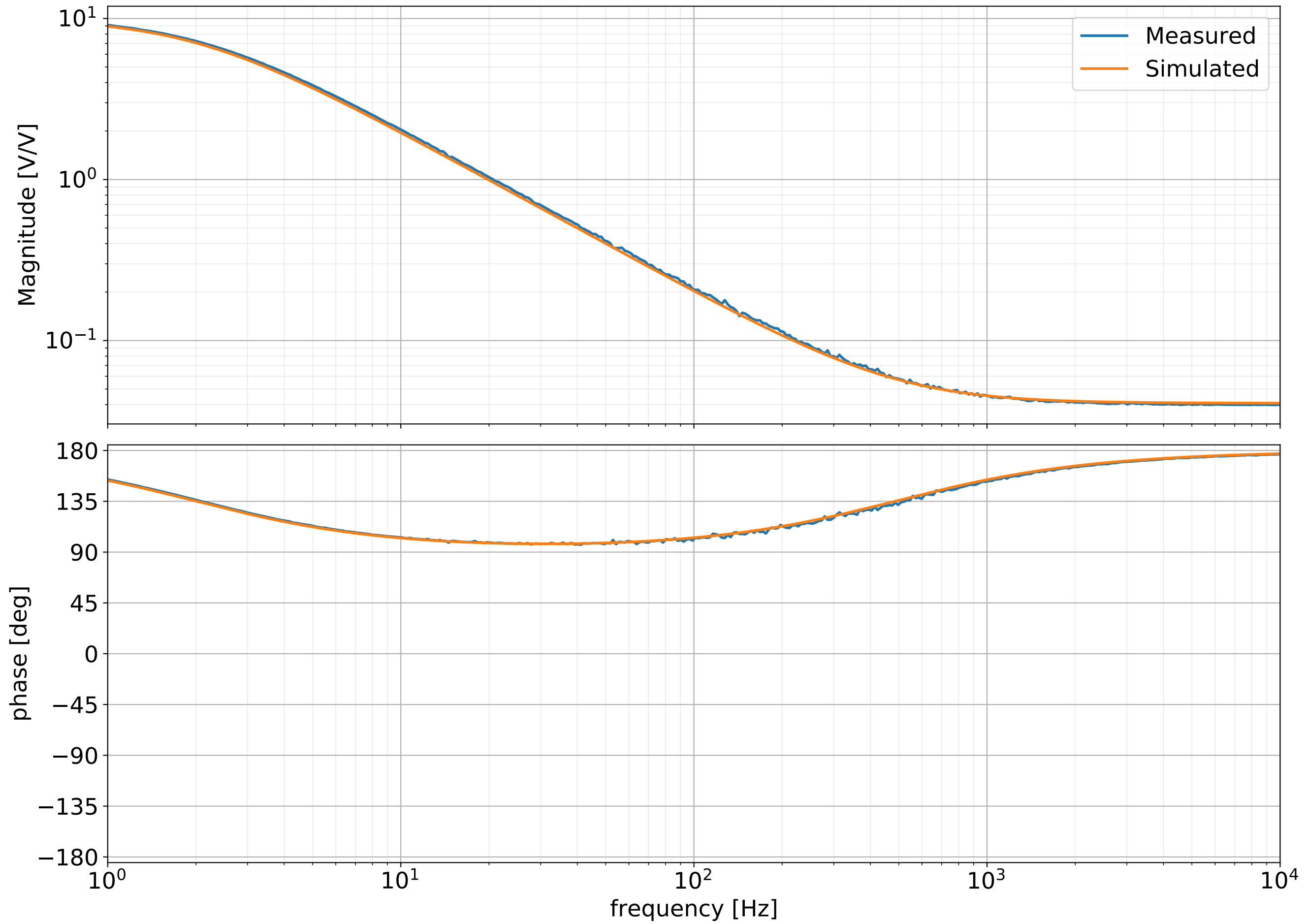
Transfer function from TP2 to TP4 in North PMC box
