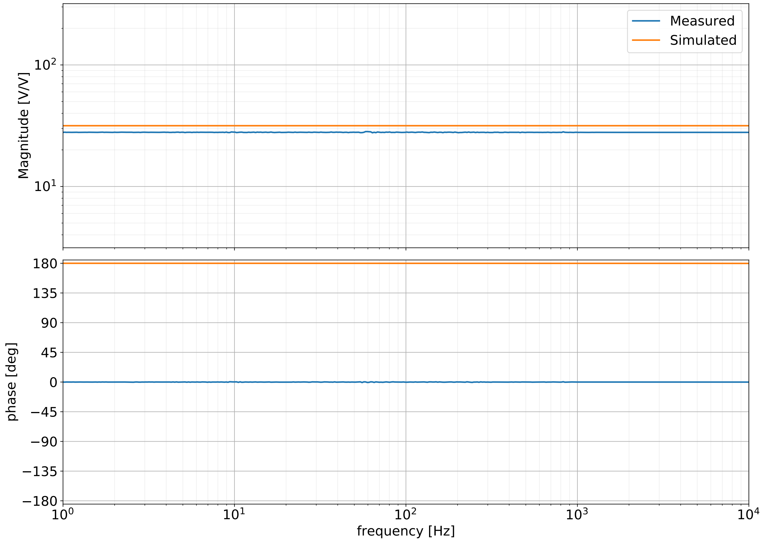
Transfer function from TP1 to TP2 in North PMC box
