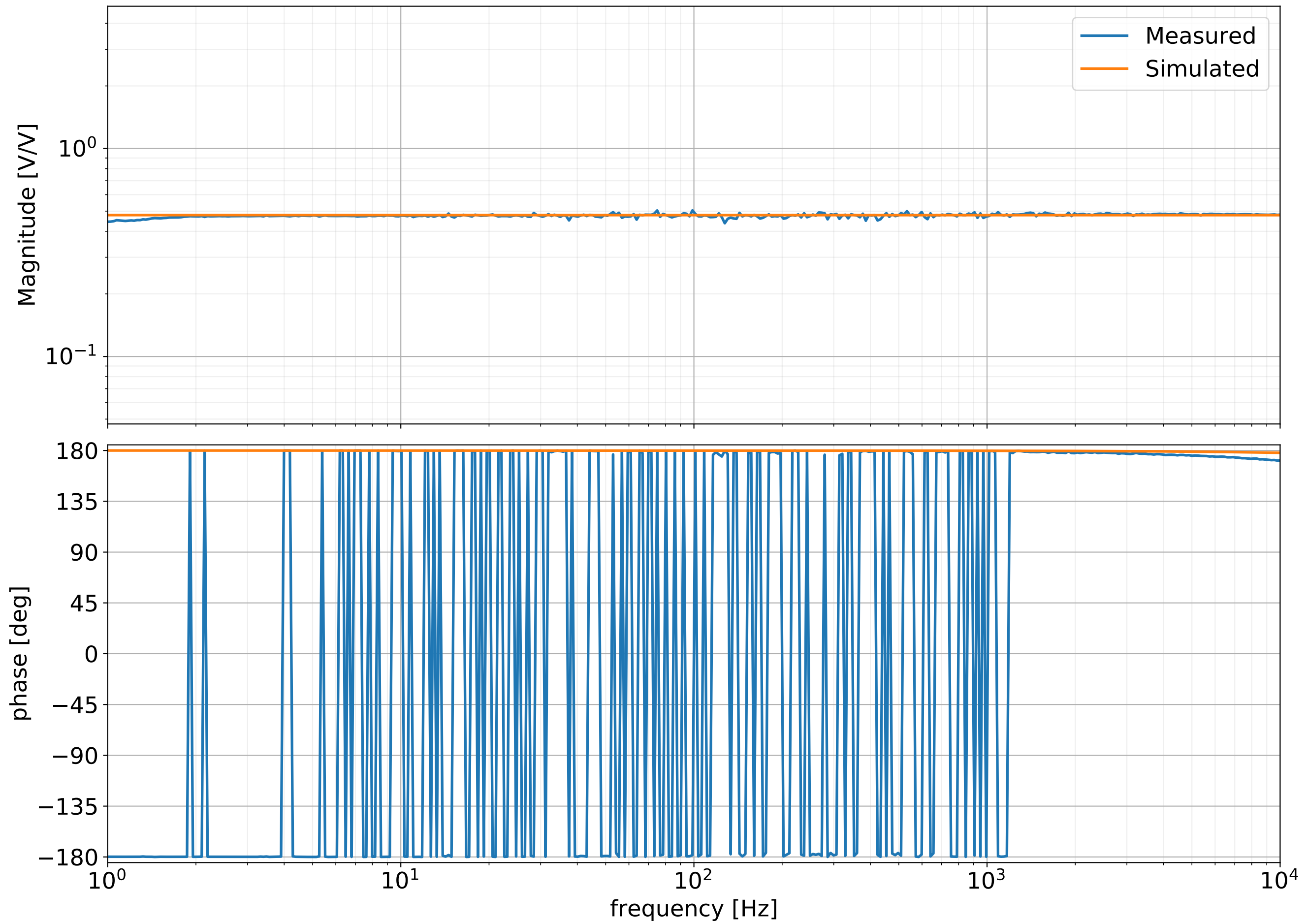
Transfer function from TP4 to TP3 in North PMC box
