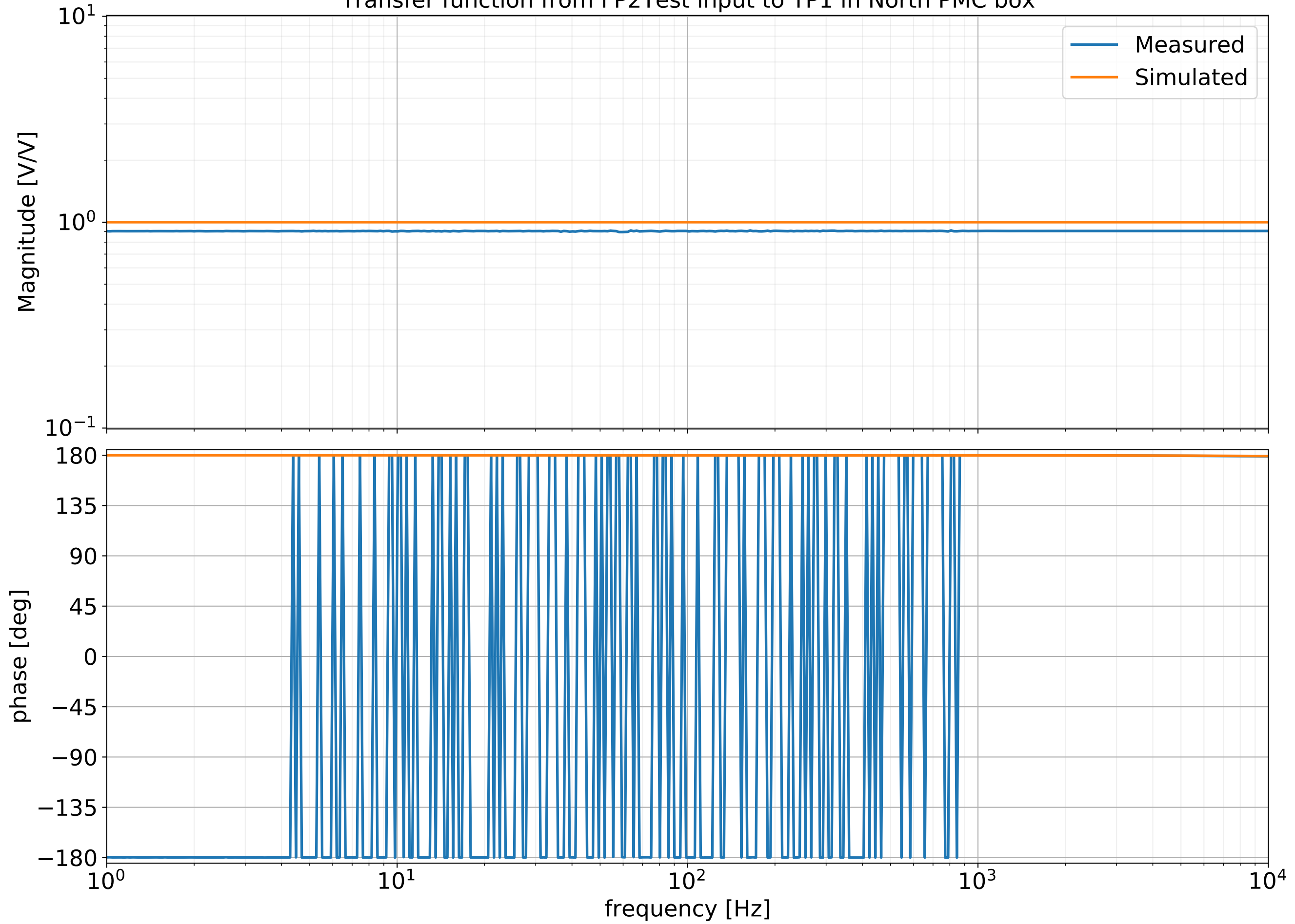
Transfer function from FP2Test input to TP1 in North PMC box
