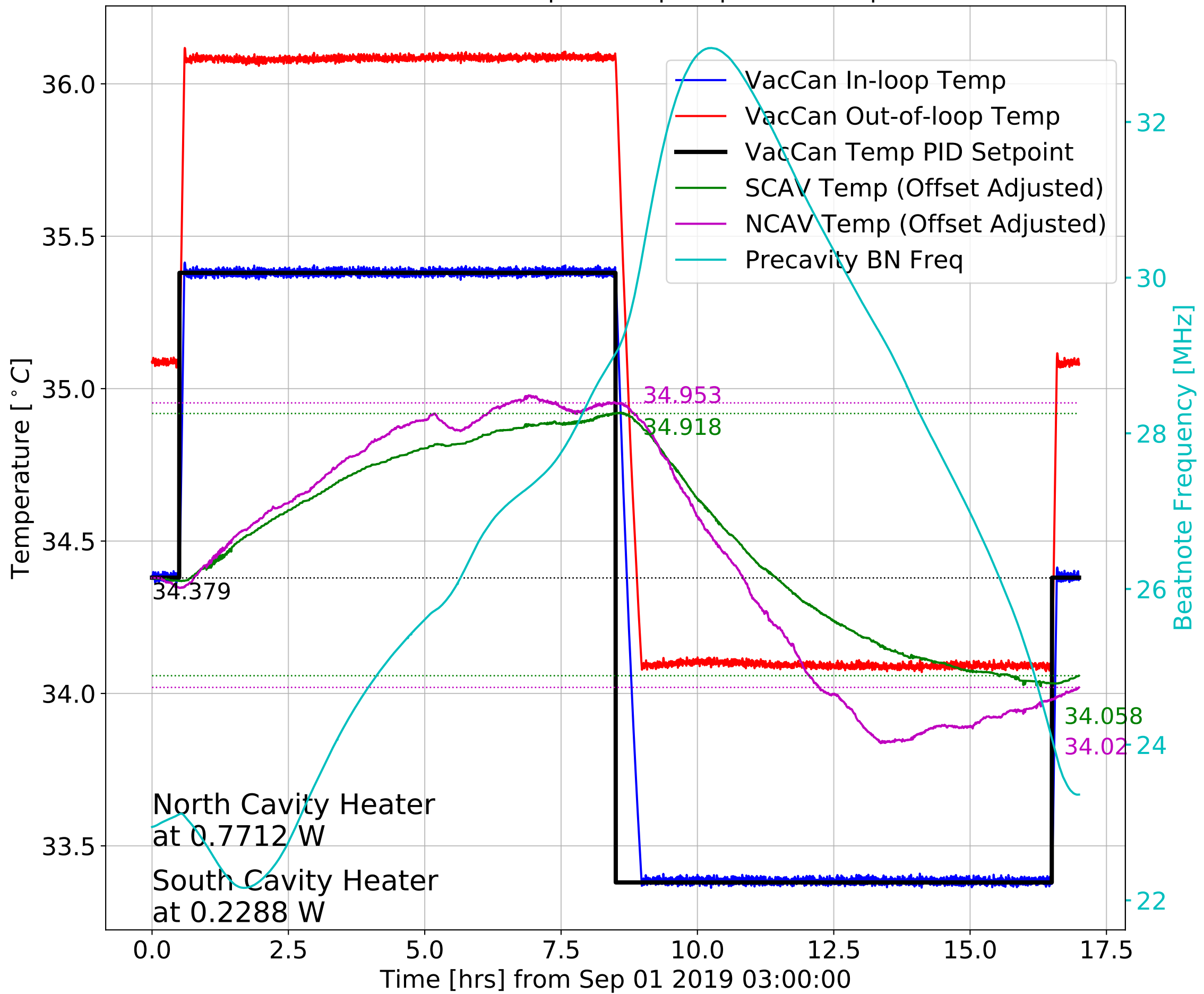
CTN Vacuum Can PID Setpoint Step response on Sep 01 2019
