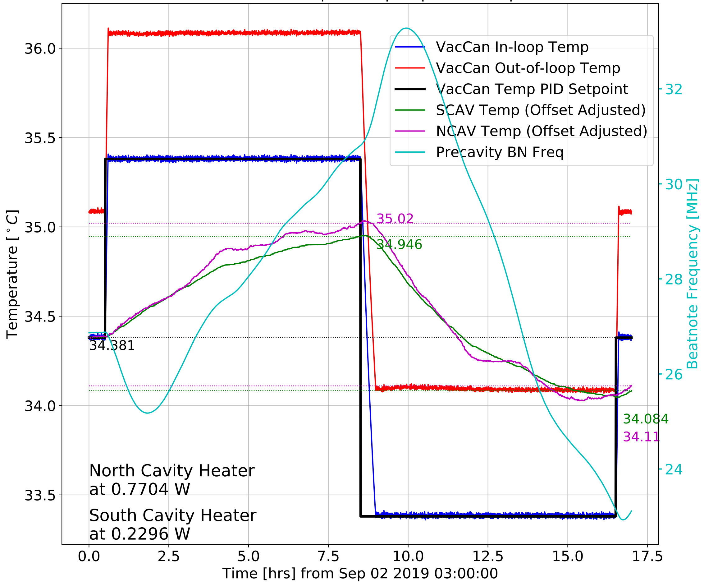
CTN Vacuum Can PID Setpoint Step response on Sep 02 2019
