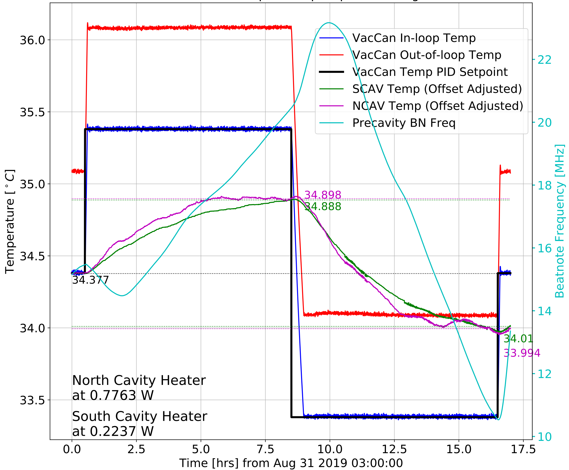
CTN Vacuum Can PID Setpoint Step response on Aug 31 2019
