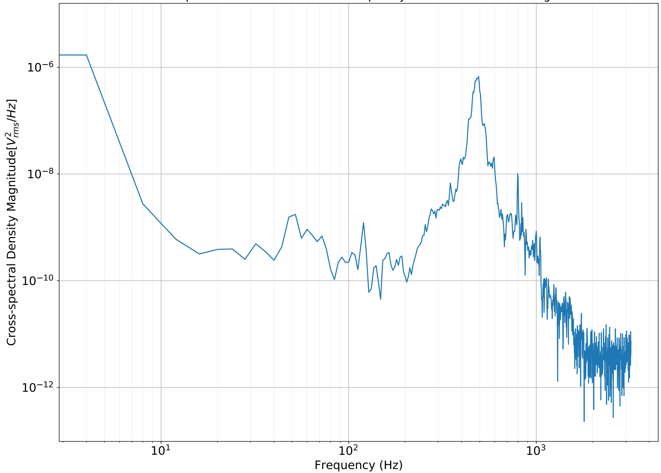
Cross-spectrum between beatnote frequency and North PMC Error Signal
