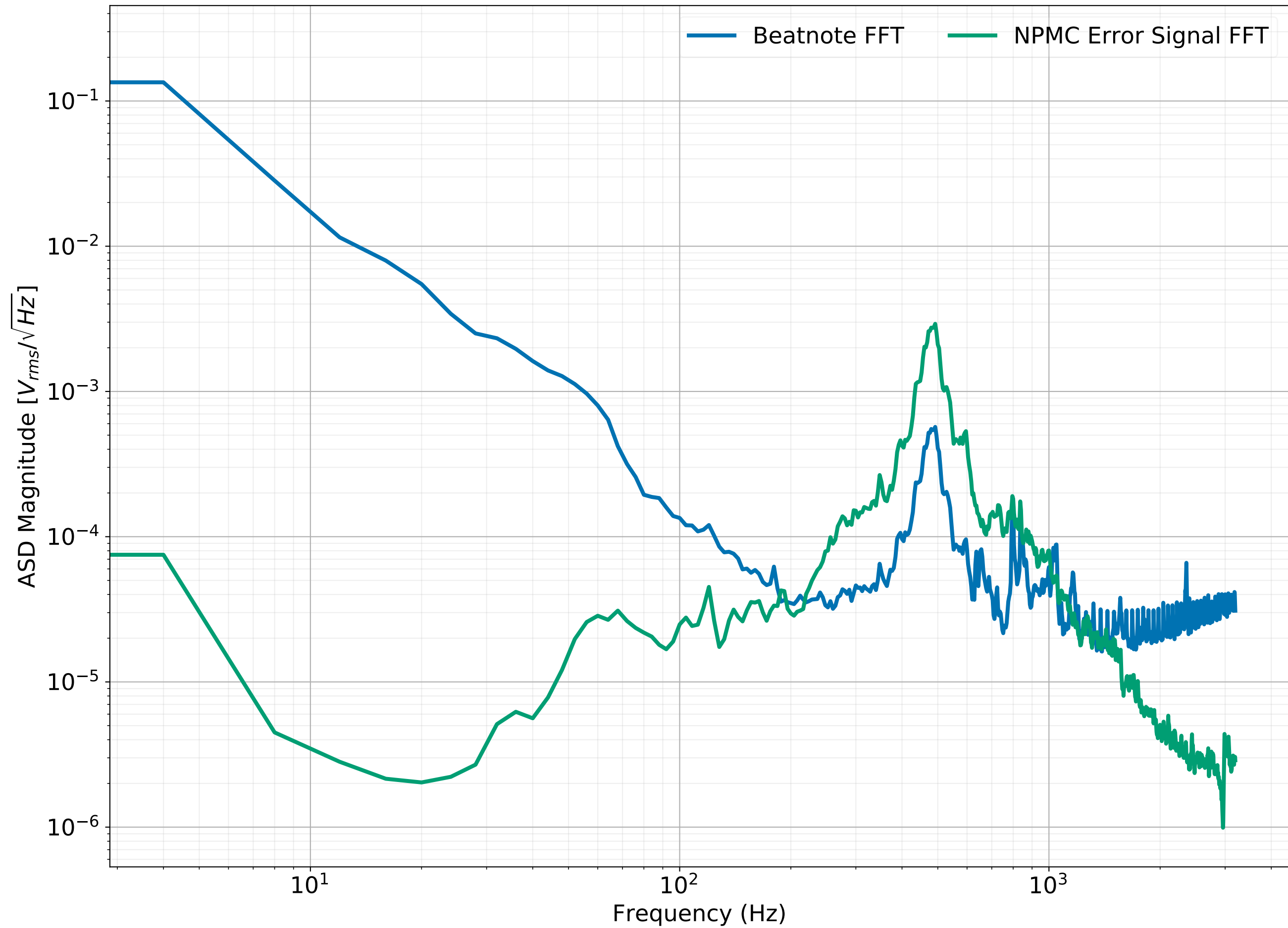
FFT of Beatnote and NPMC Error
