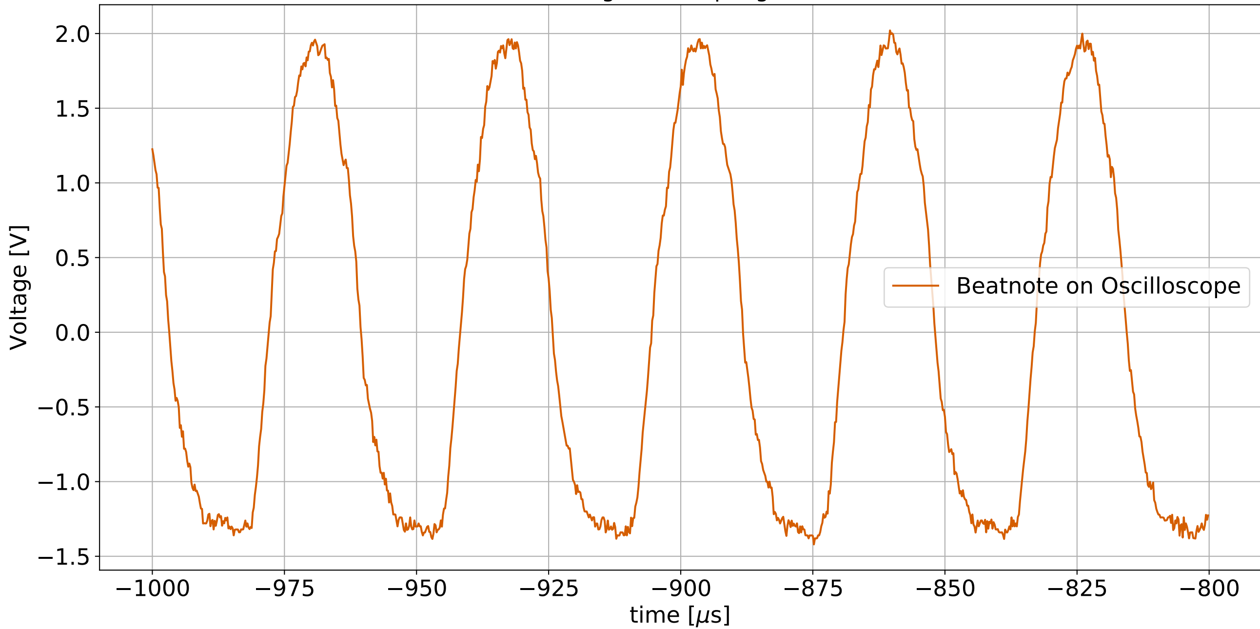
CTN Beatnote Signal, Sampling Rate 5.0 GSa/s
