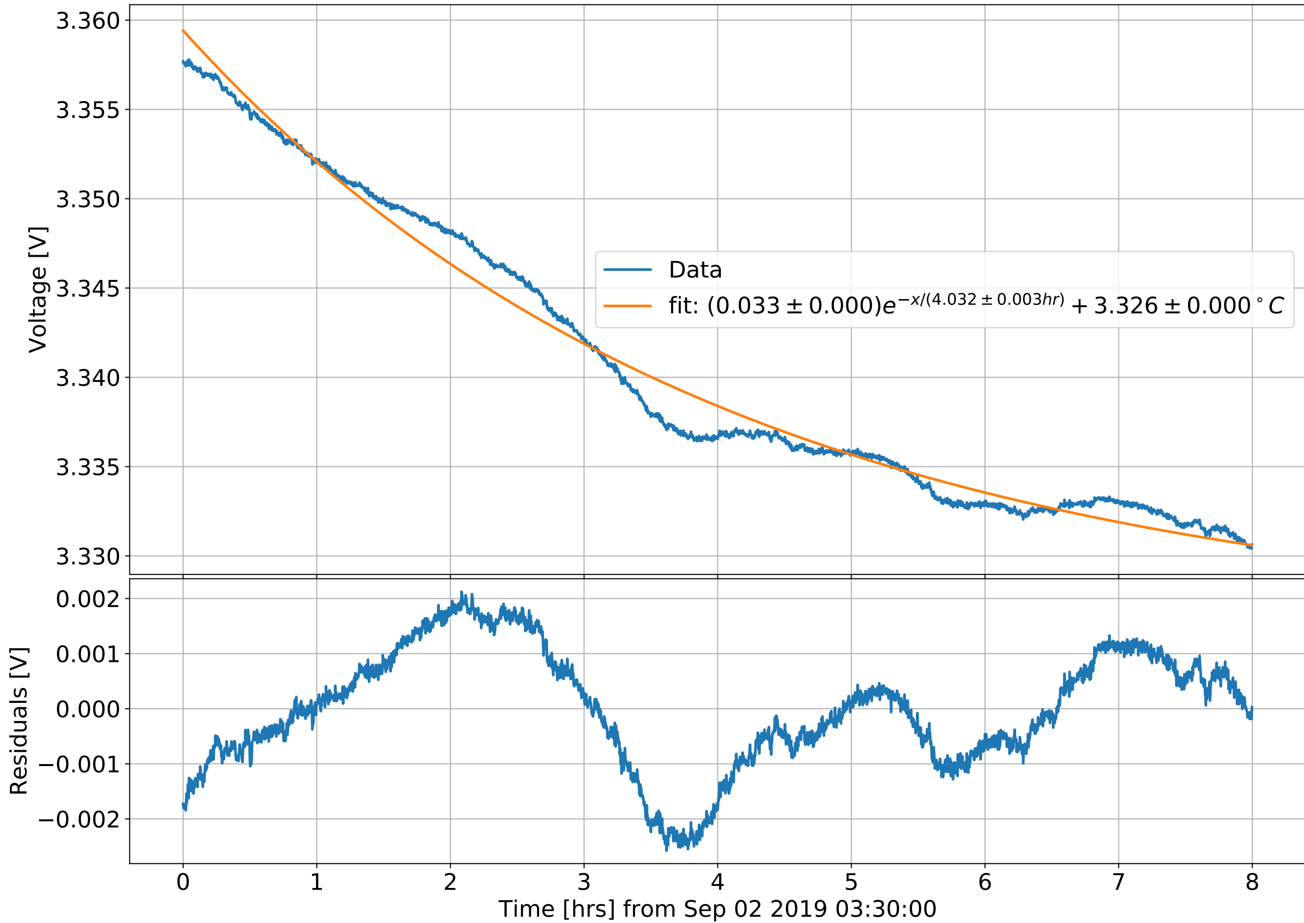
CTN Vacuum Can PID Setpoint Step response on Sep 02 2019 North FSS Slowout Fit
