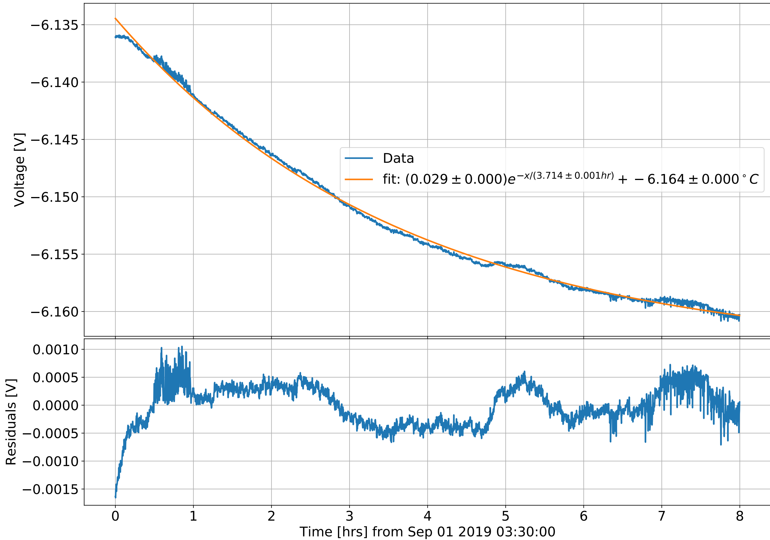
CTN Vacuum Can PID Setpoint Step response on Sep 01 2019 South FSS Slowout Fit
