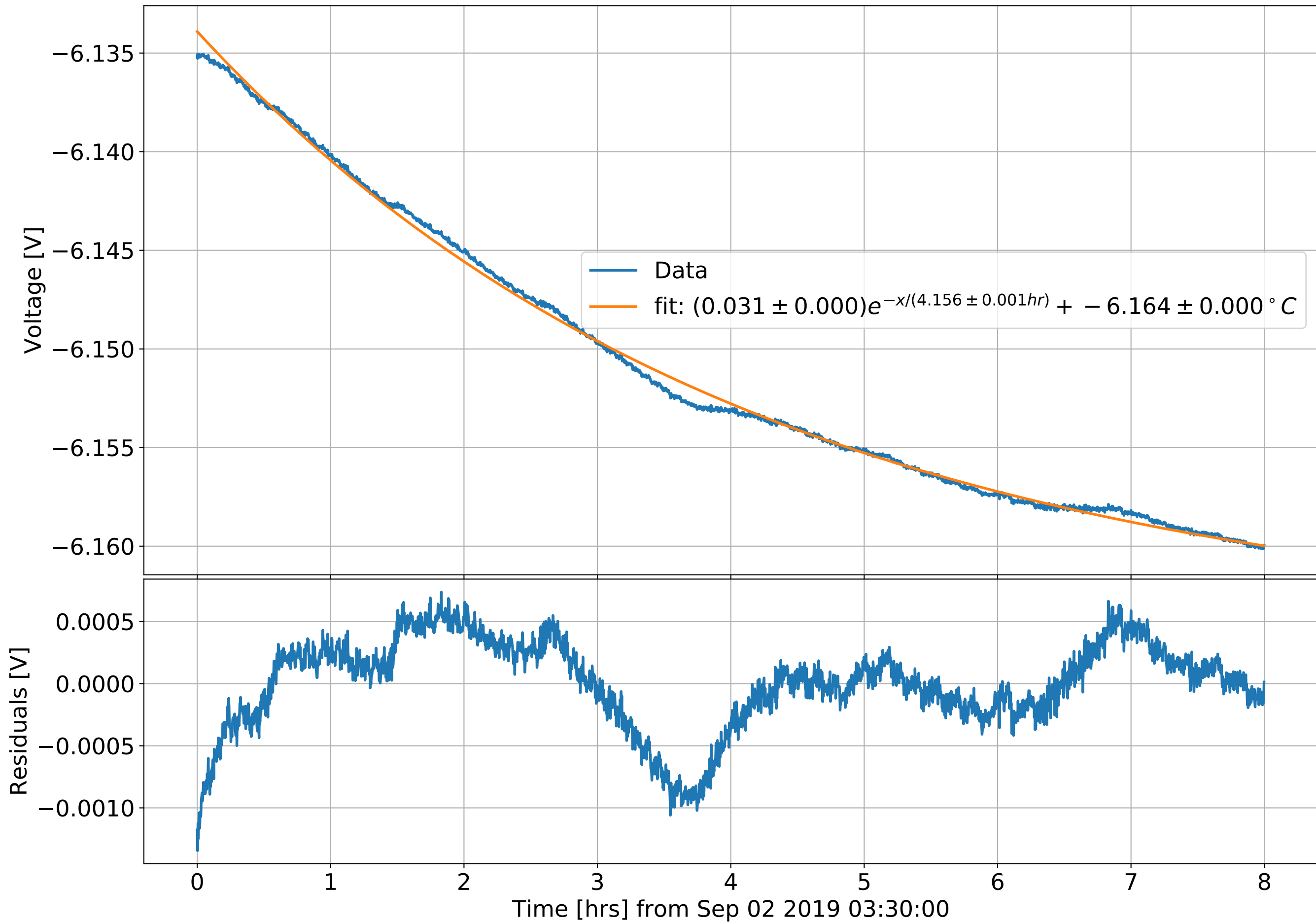
CTN Vacuum Can PID Setpoint Step response on Sep 02 2019 South FSS Slowout Fit
