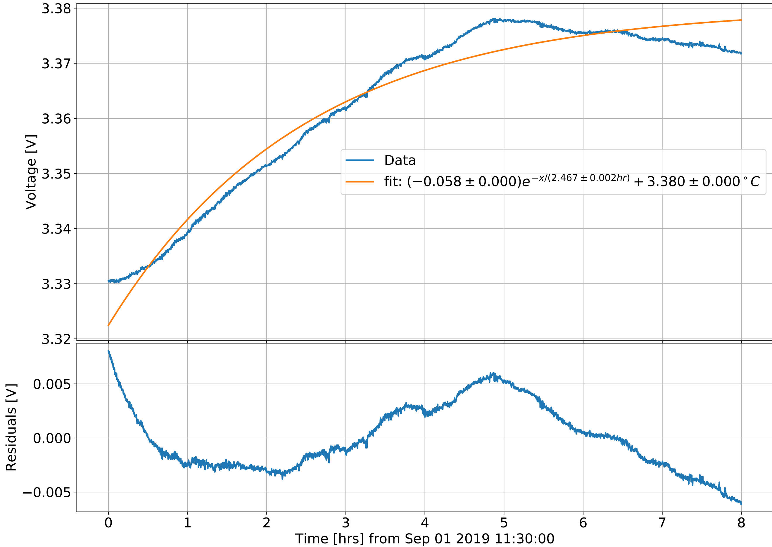
CTN Vacuum Can PID Setpoint Step response on Sep 01 2019 North FSS Slowout Fit
