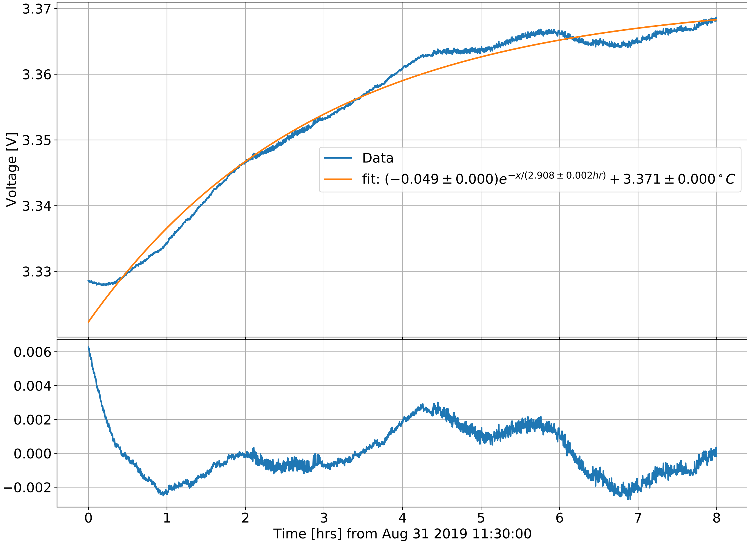
CTN Vacuum Can PID Setpoint Step response on Aug 31 2019 North FSS Slowout Fit
