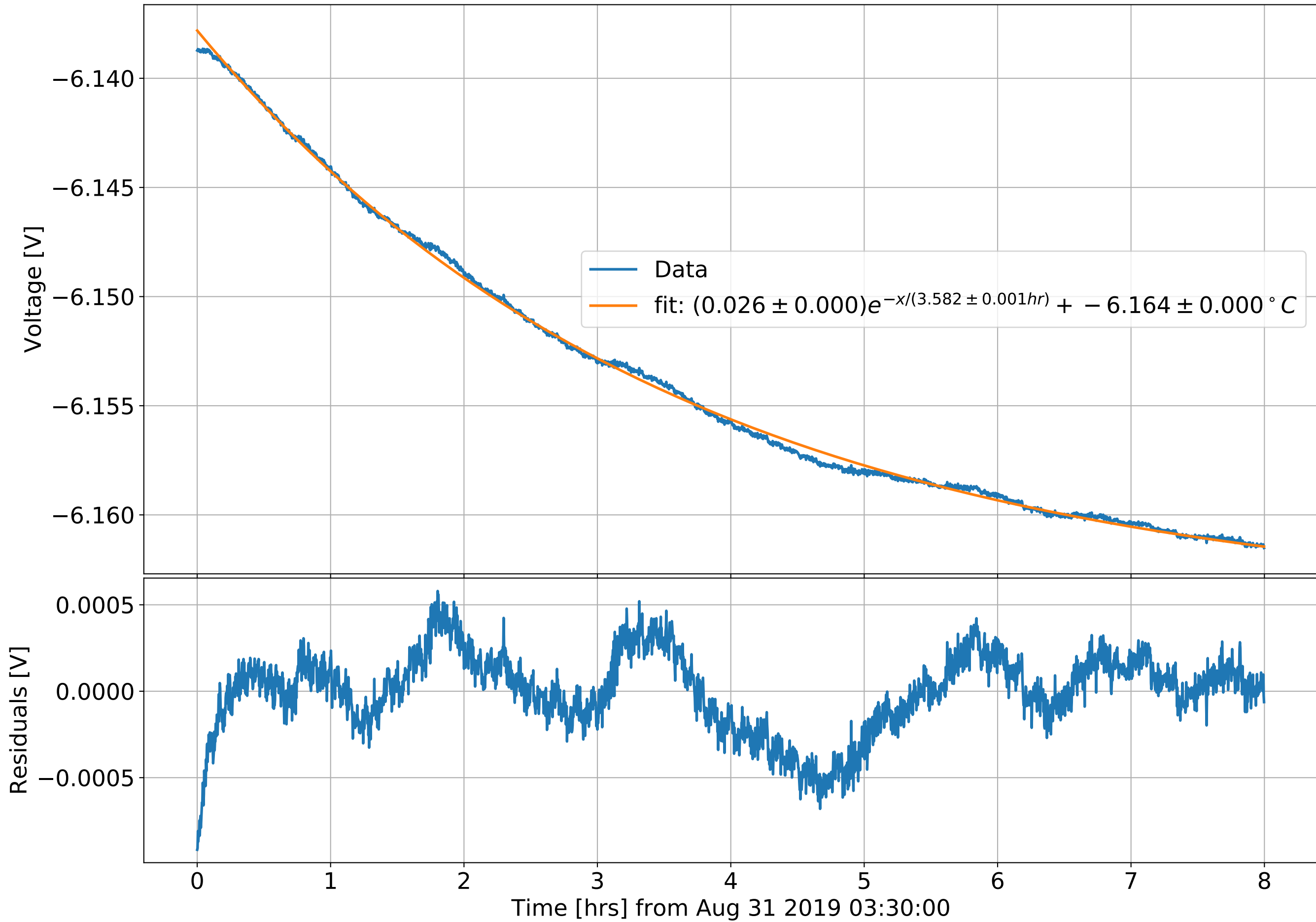
CTN Vacuum Can PID Setpoint Step response on Aug 31 2019 South FSS Slowout Fit
