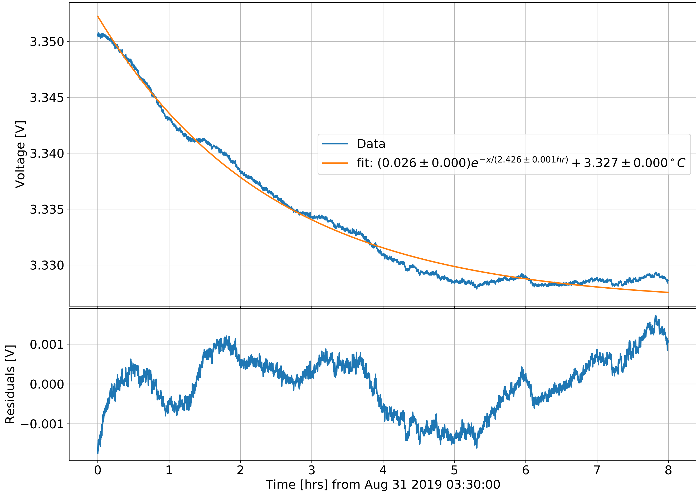
CTN Vacuum Can PID Setpoint Step response on Aug 31 2019 North FSS Slowout Fit
