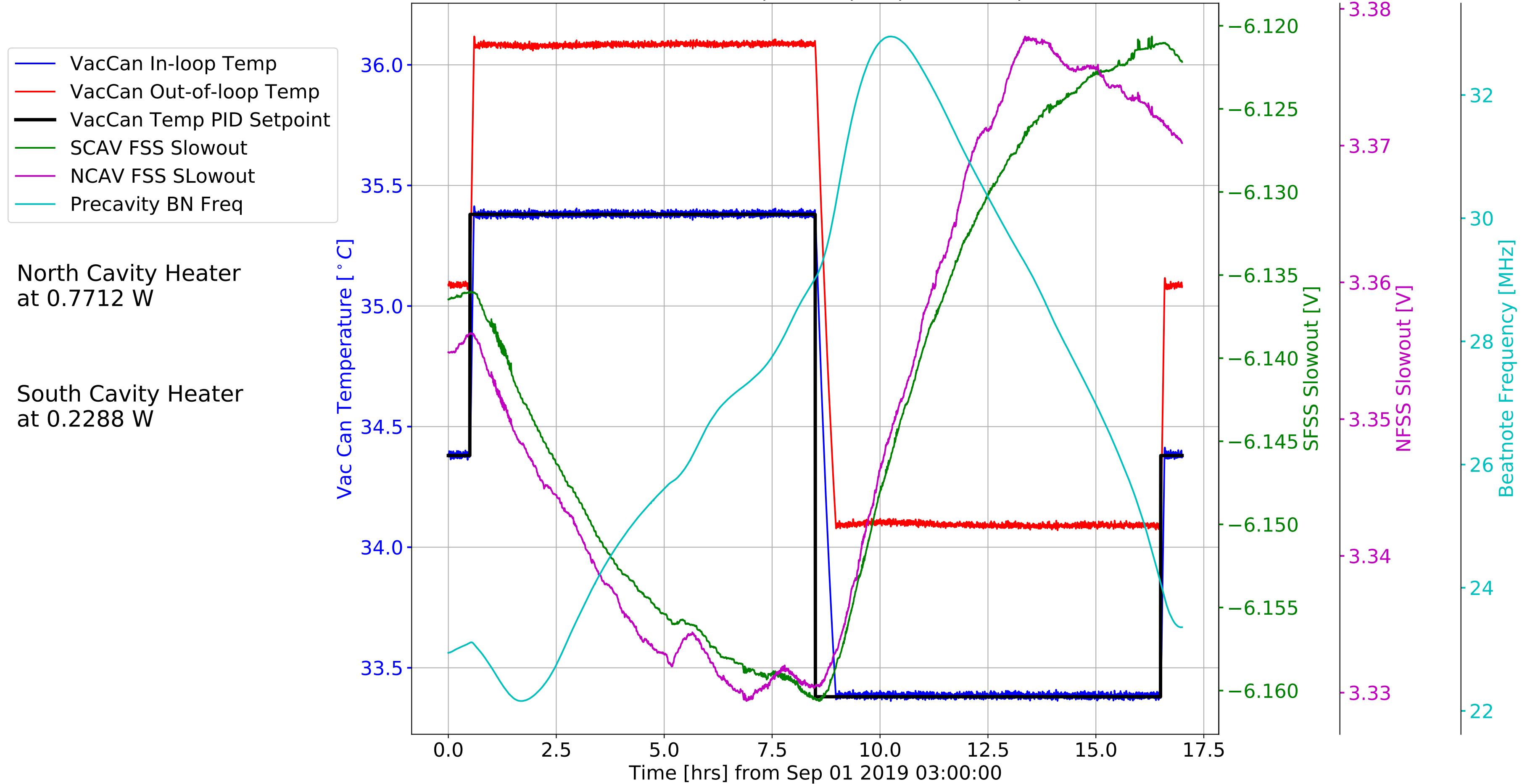
CTN Vacuum Can PID Setpoint Step response on Sep 01 2019
