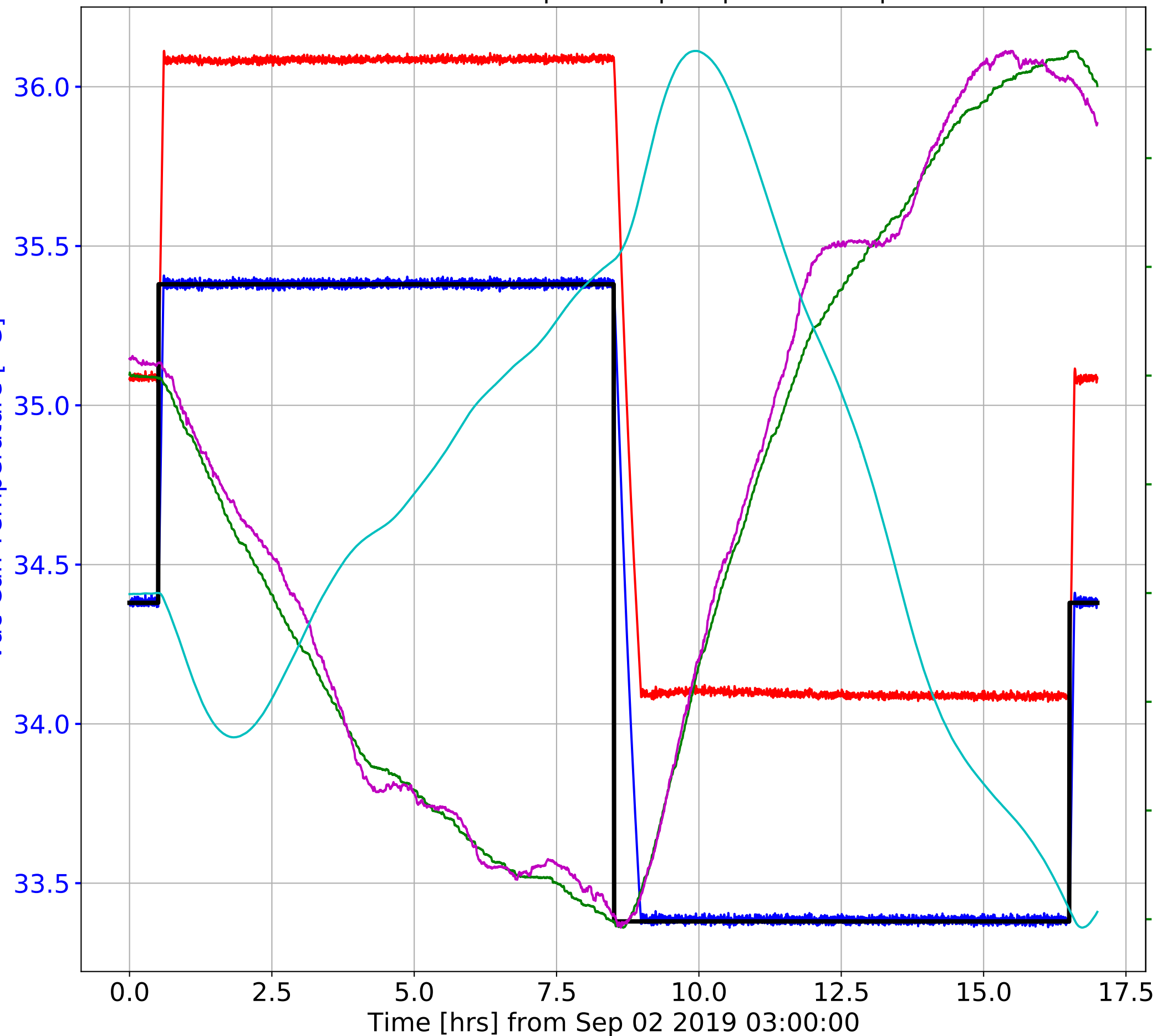
CTN Vacuum Can PID Setpoint Step response on Sep 02 2019
