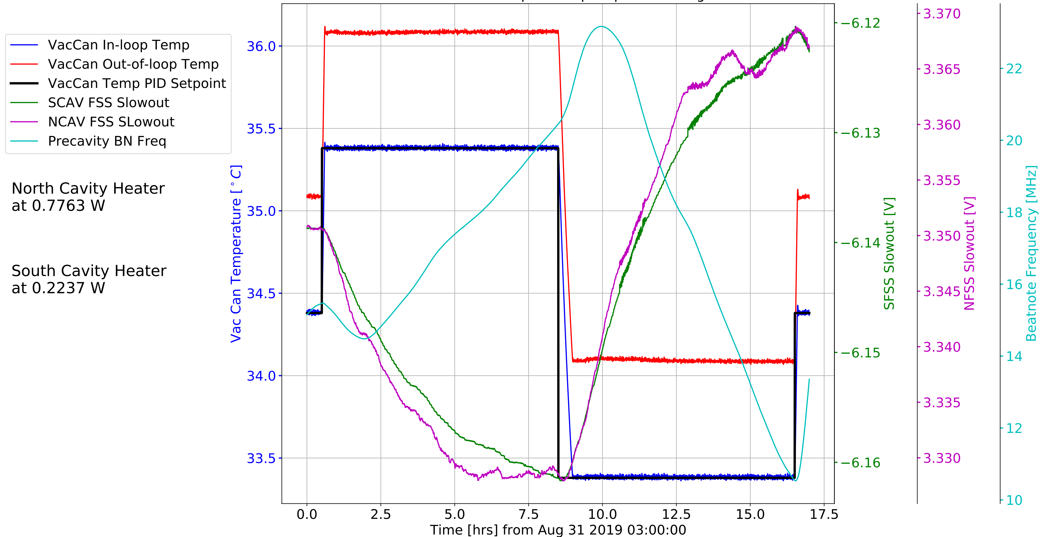
CTN Vacuum Can PID Setpoint Step response on Aug 31 2019
