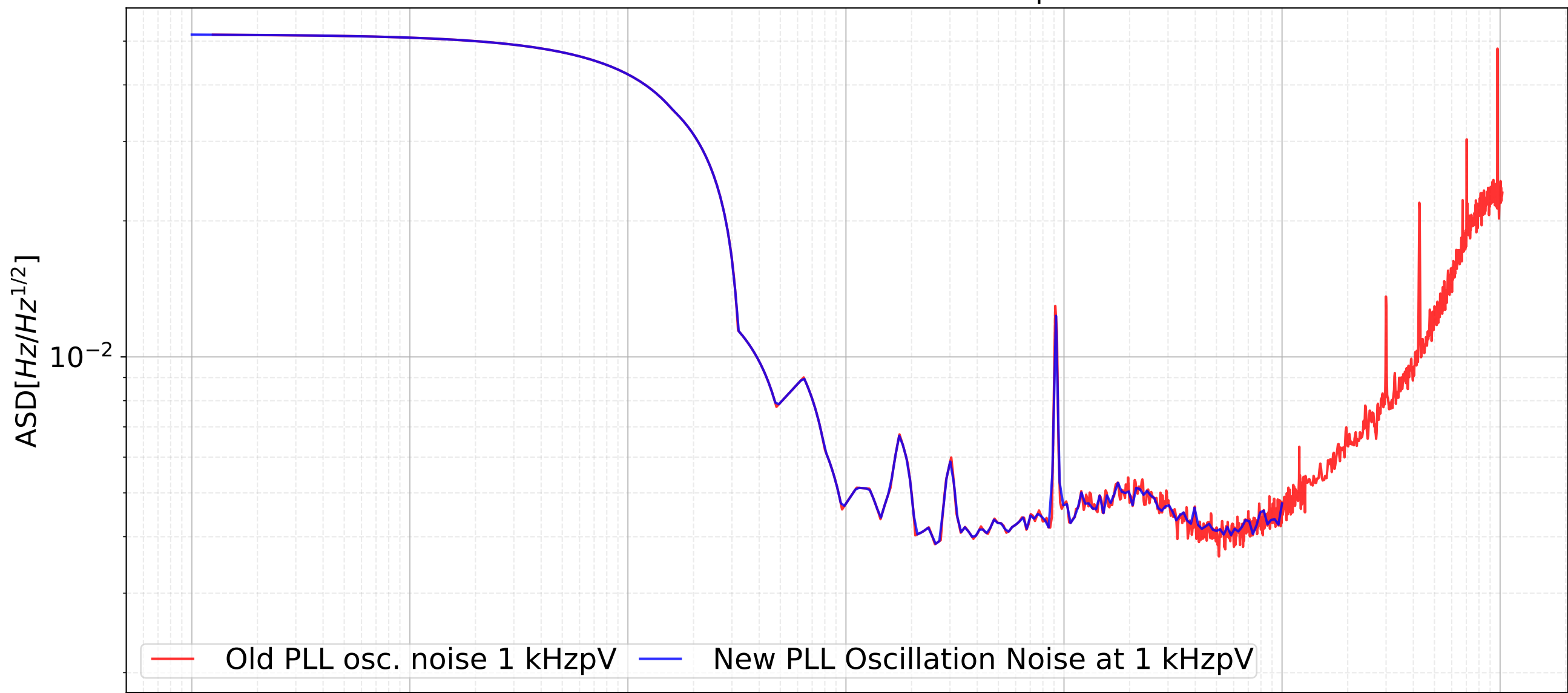
PLL Oscillation Noise at 1 kHzpV
