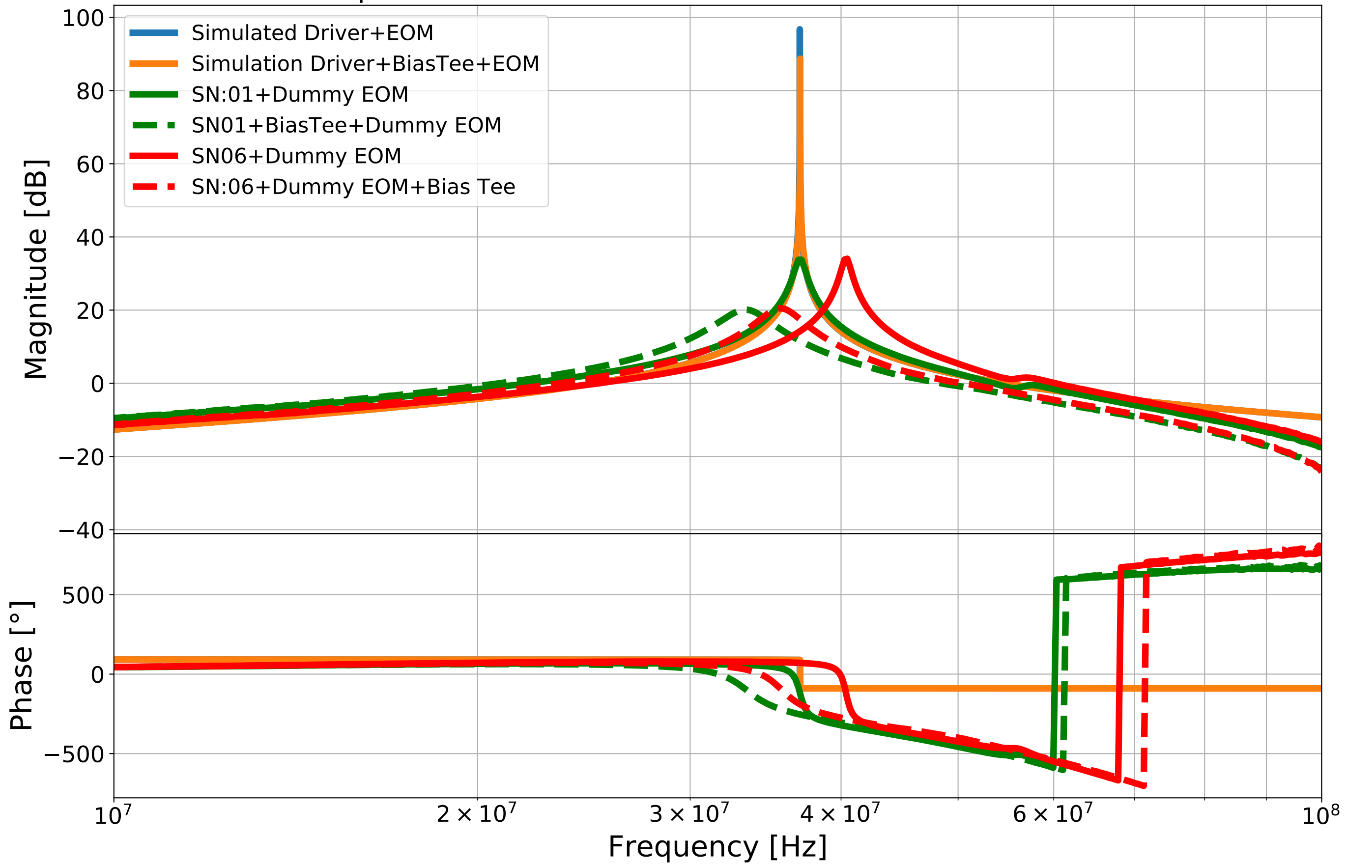
Comparison of Transfer function of EOM Drivers with Simulation
