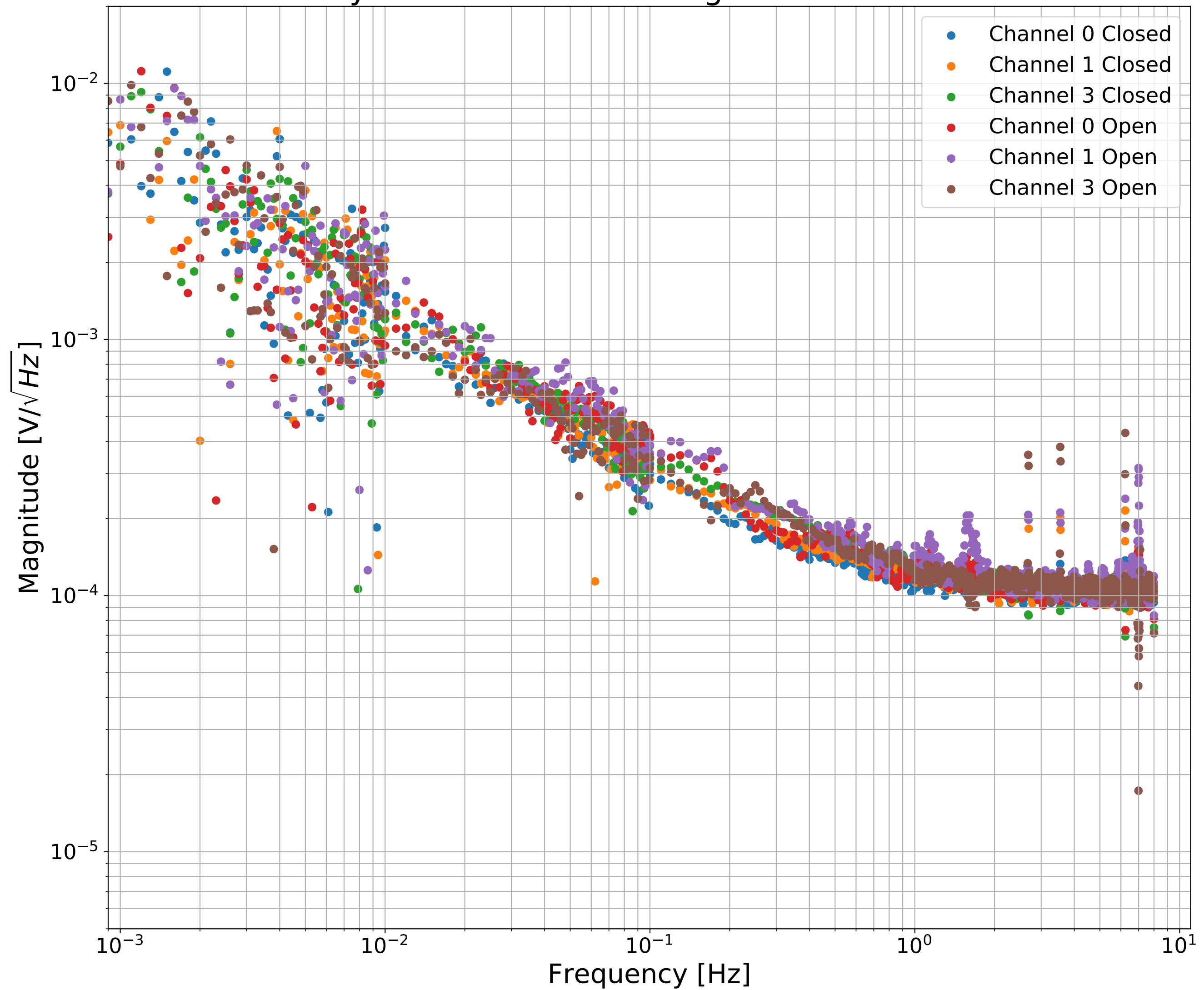
Noise density in each AD590 through Difference Measurement
