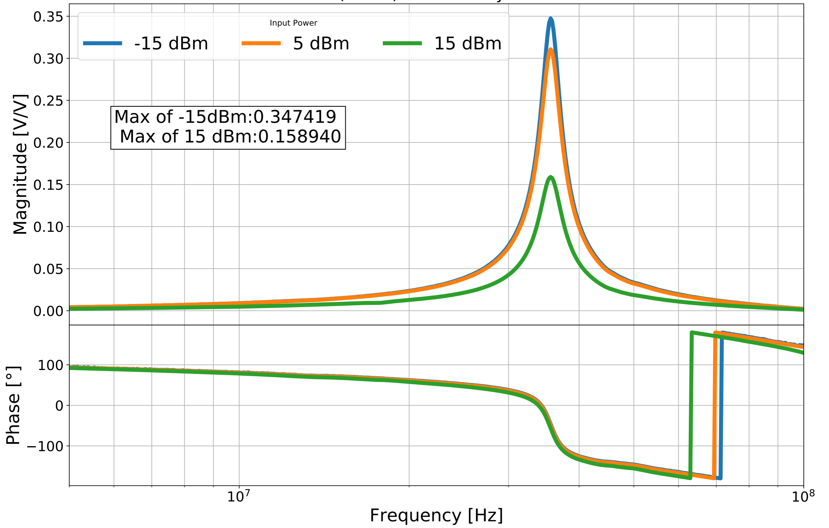
Transfer function of New EOM Driver(SN:06) with Dummy EOM and Bias Tee from RF in to RF Mon
