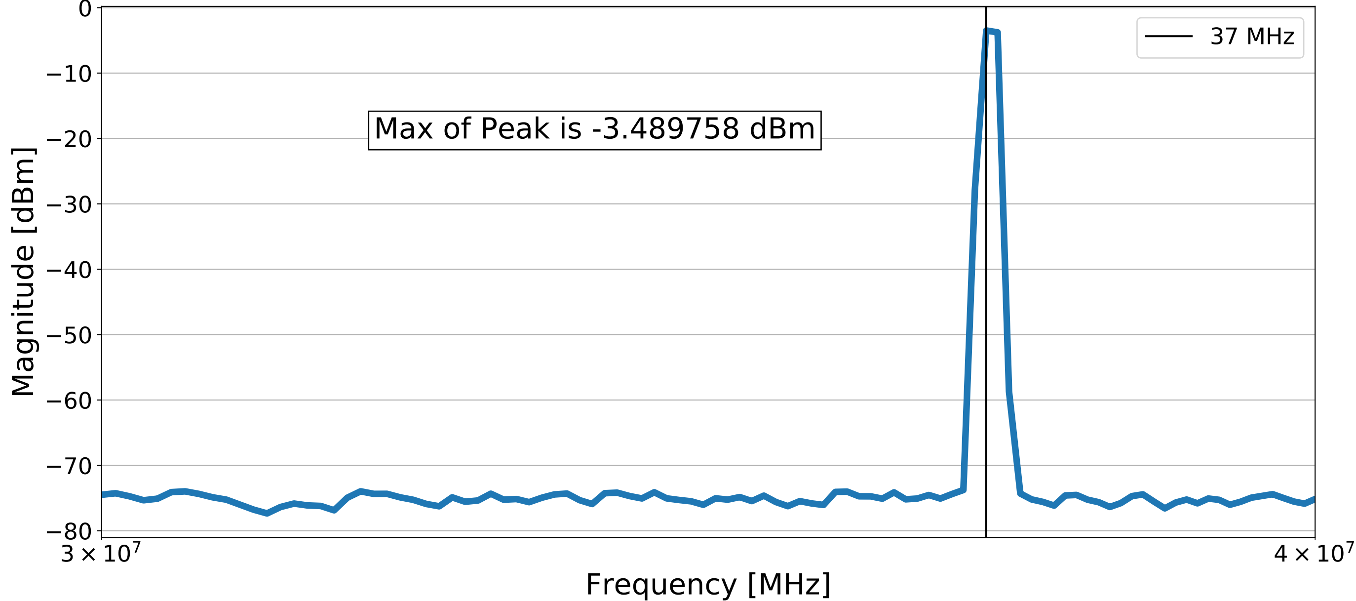
Spectrum of EOM Driver with real EOM and Bias Tee from RF mon with 16.5 dBm input
