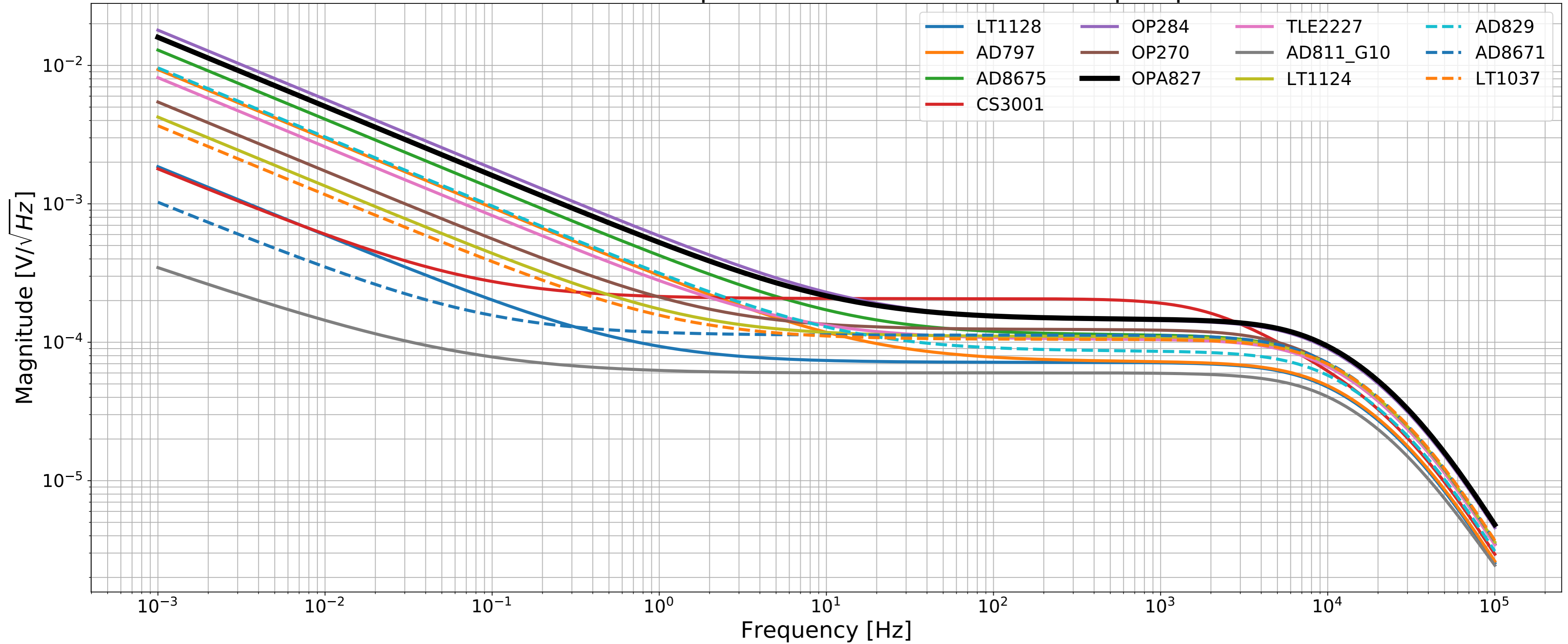
Zero Simulated Output Noise Sum with Different OpAmps
