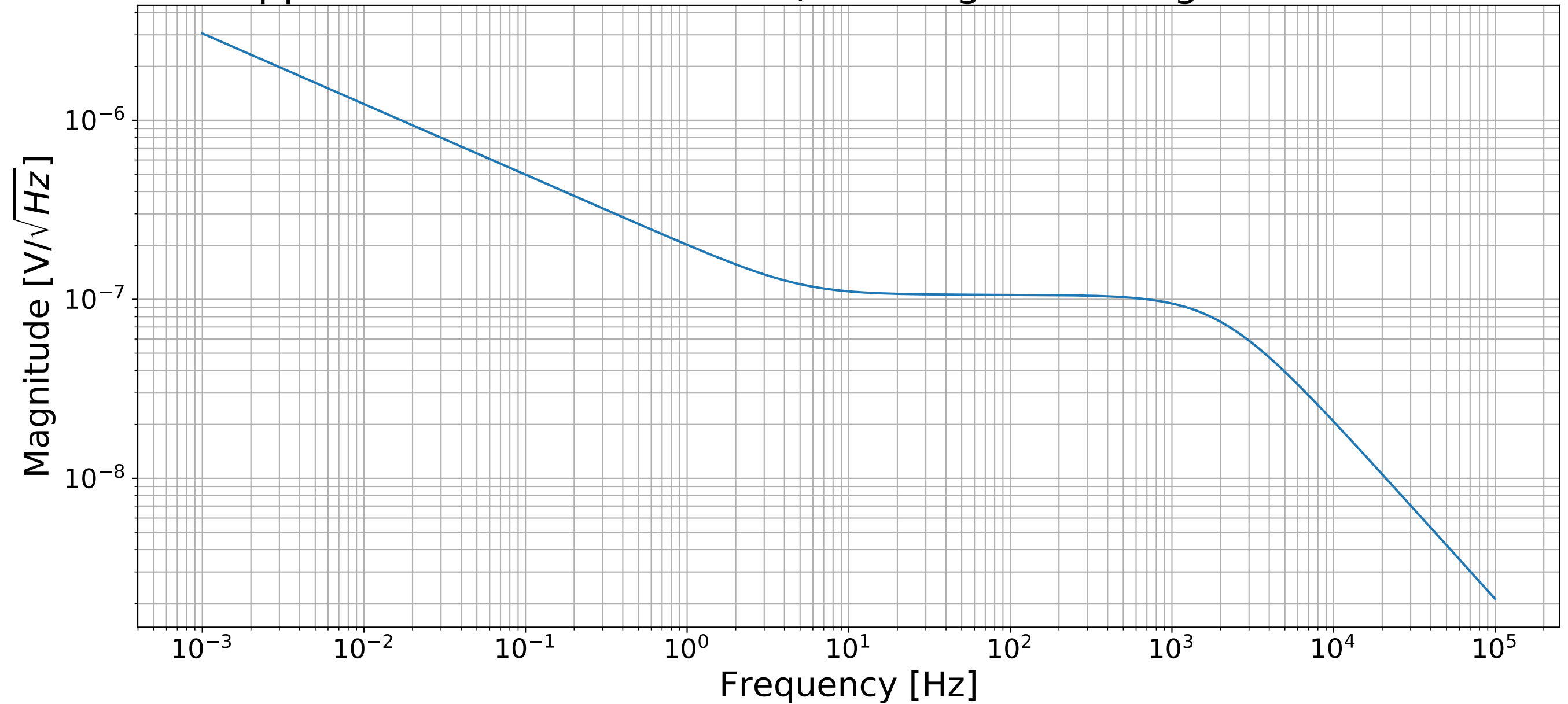
Noise Approximation of ADR4550 (From Figure 78 Page 28 of Data Sheet)
