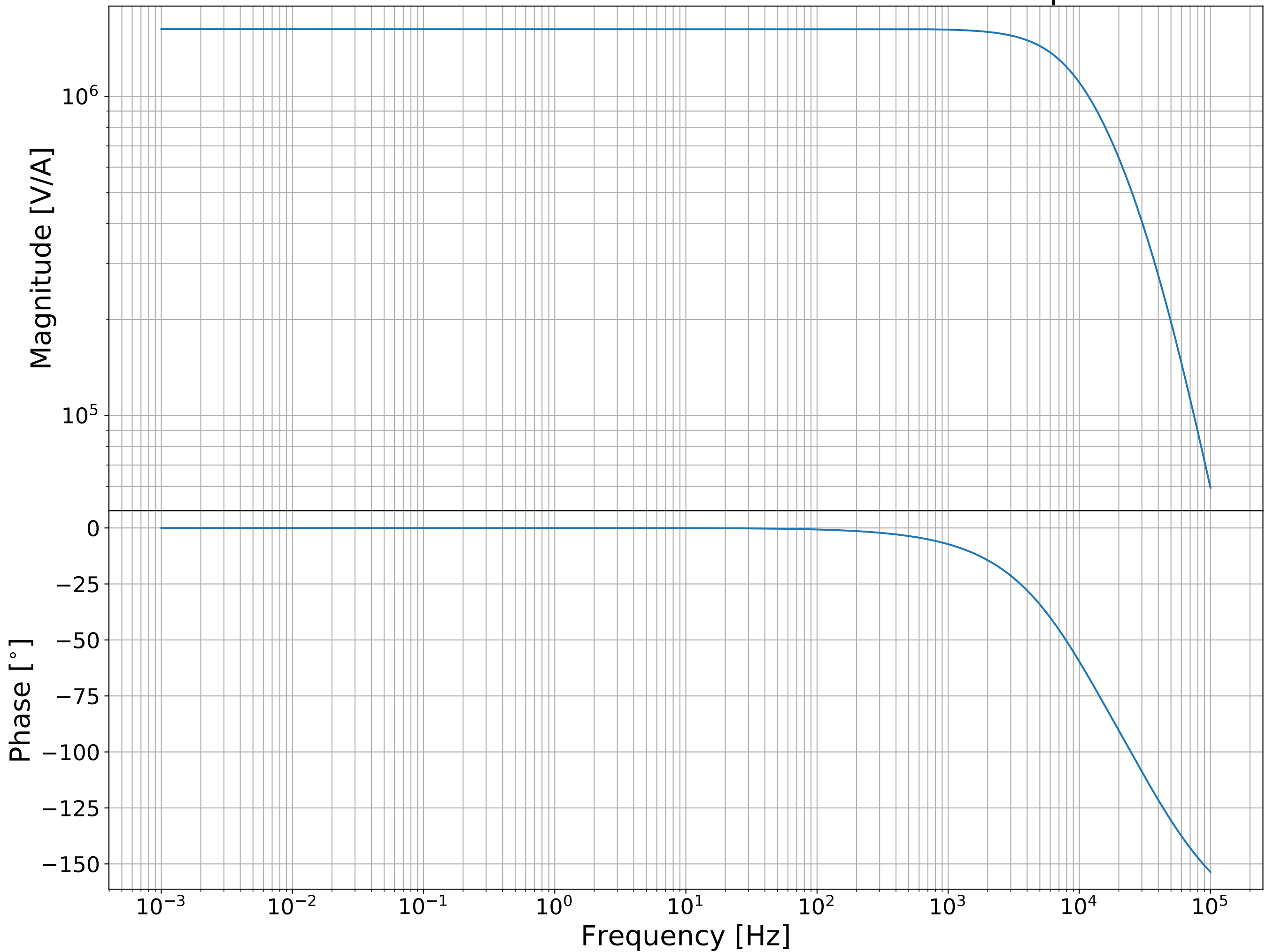
Simulated Transfer Function from AD590 to Output
