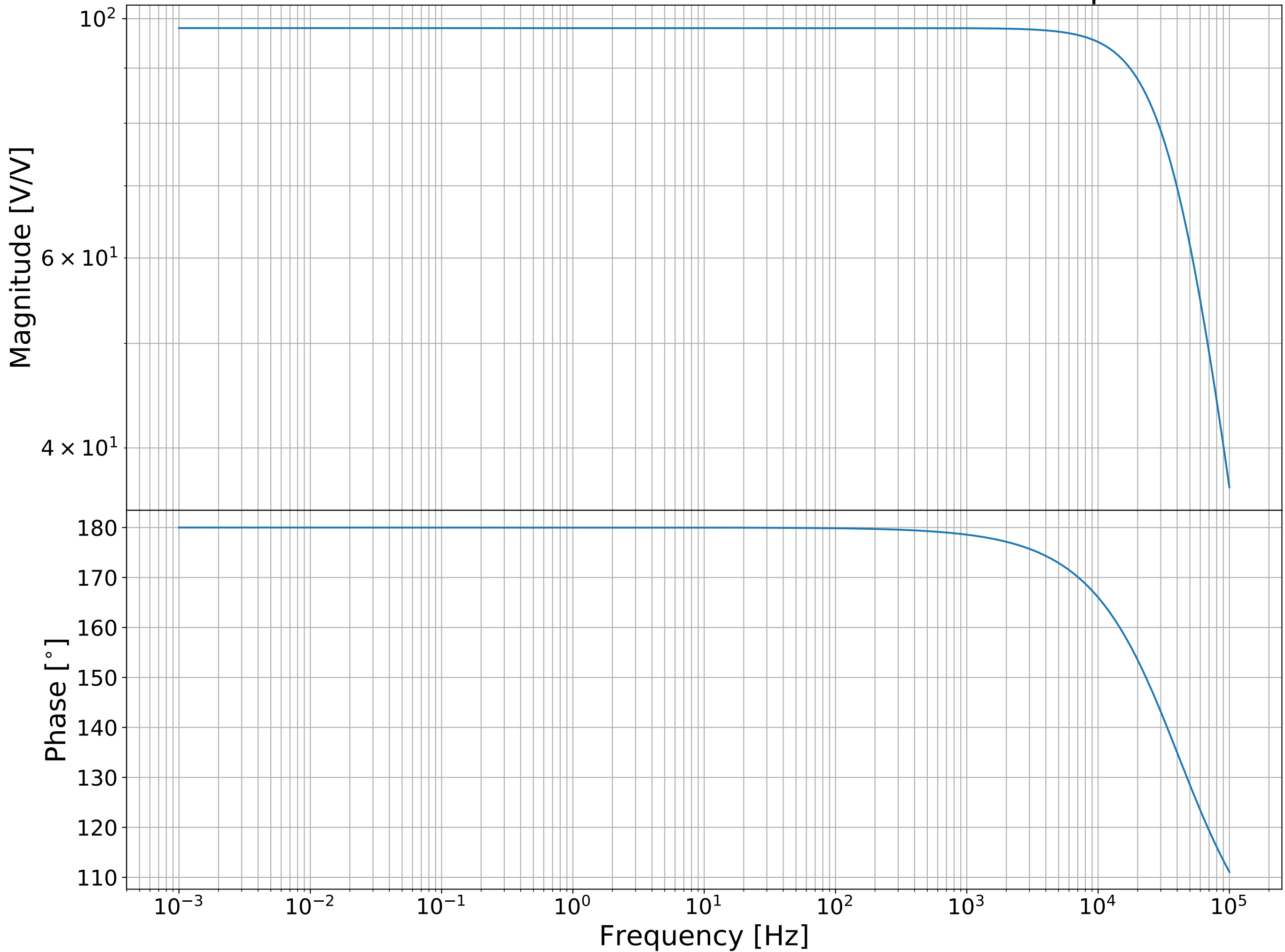
Simulated Transfer Function from ADR4550 to Output
