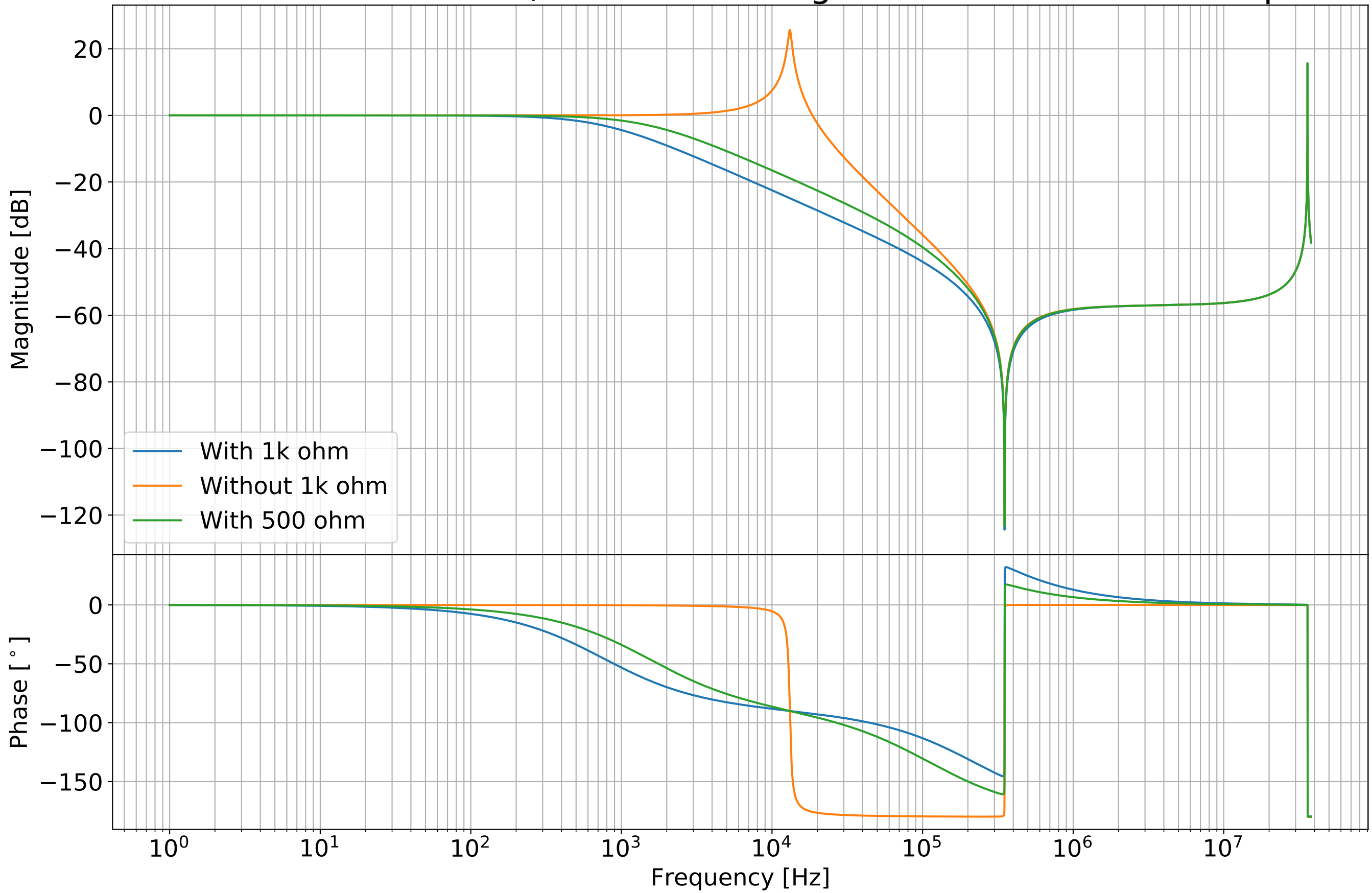
TF from DC to RF+DC, effect of adding series resistance to DC port
