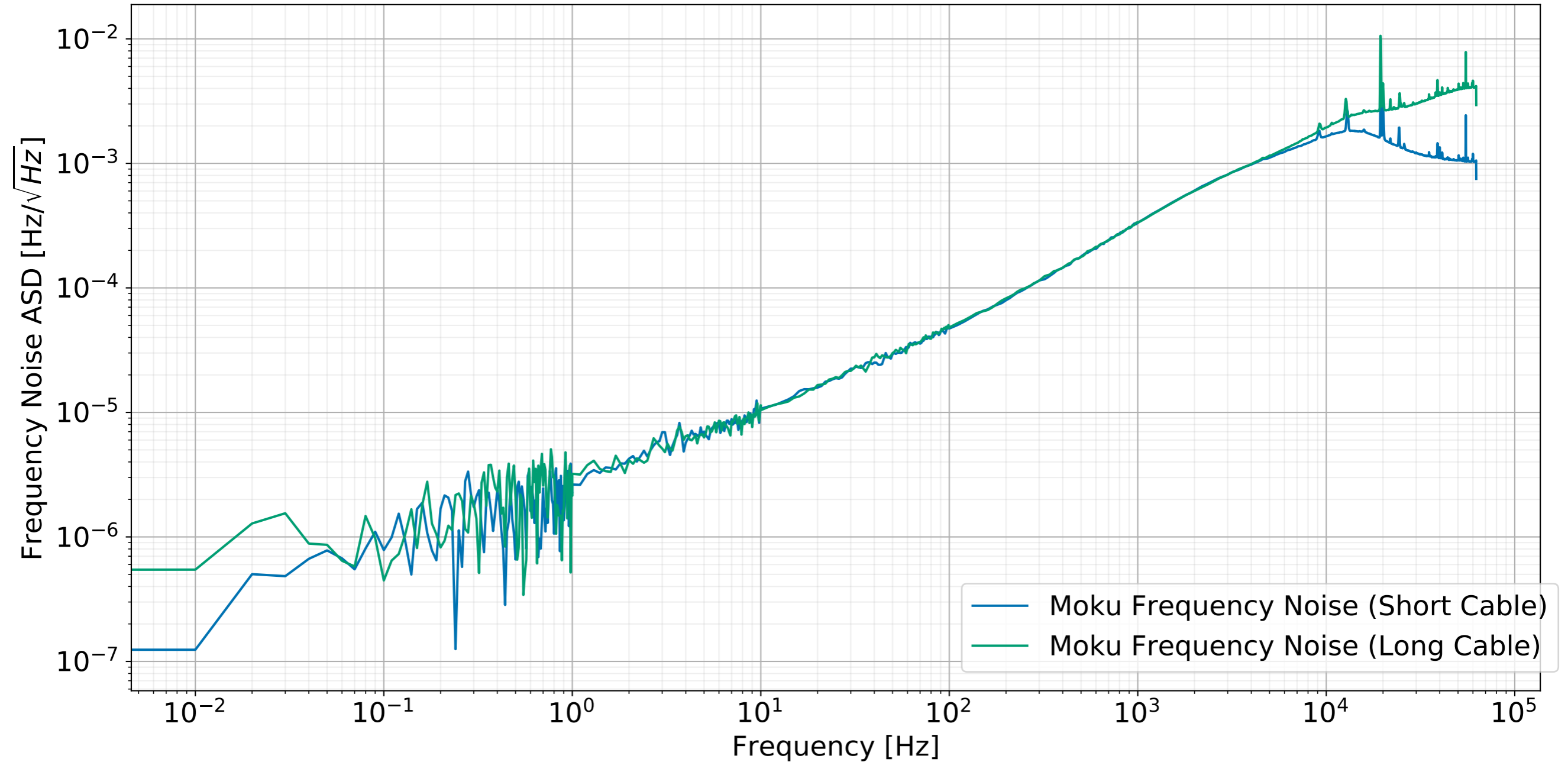
Frequency Noise of Moku output measured by itself At 27.334 MHz
