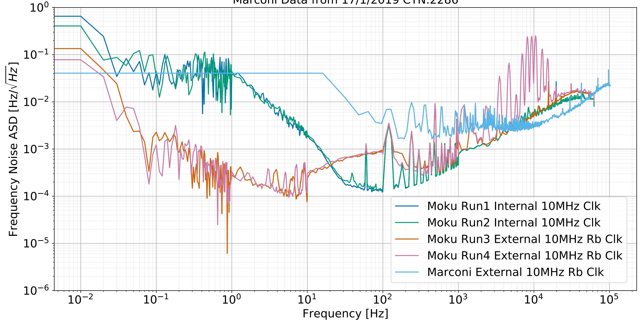
Comparison of frequency noise between Moku and Marconi Marconi Data from 17/1/2019 CTN:2286
