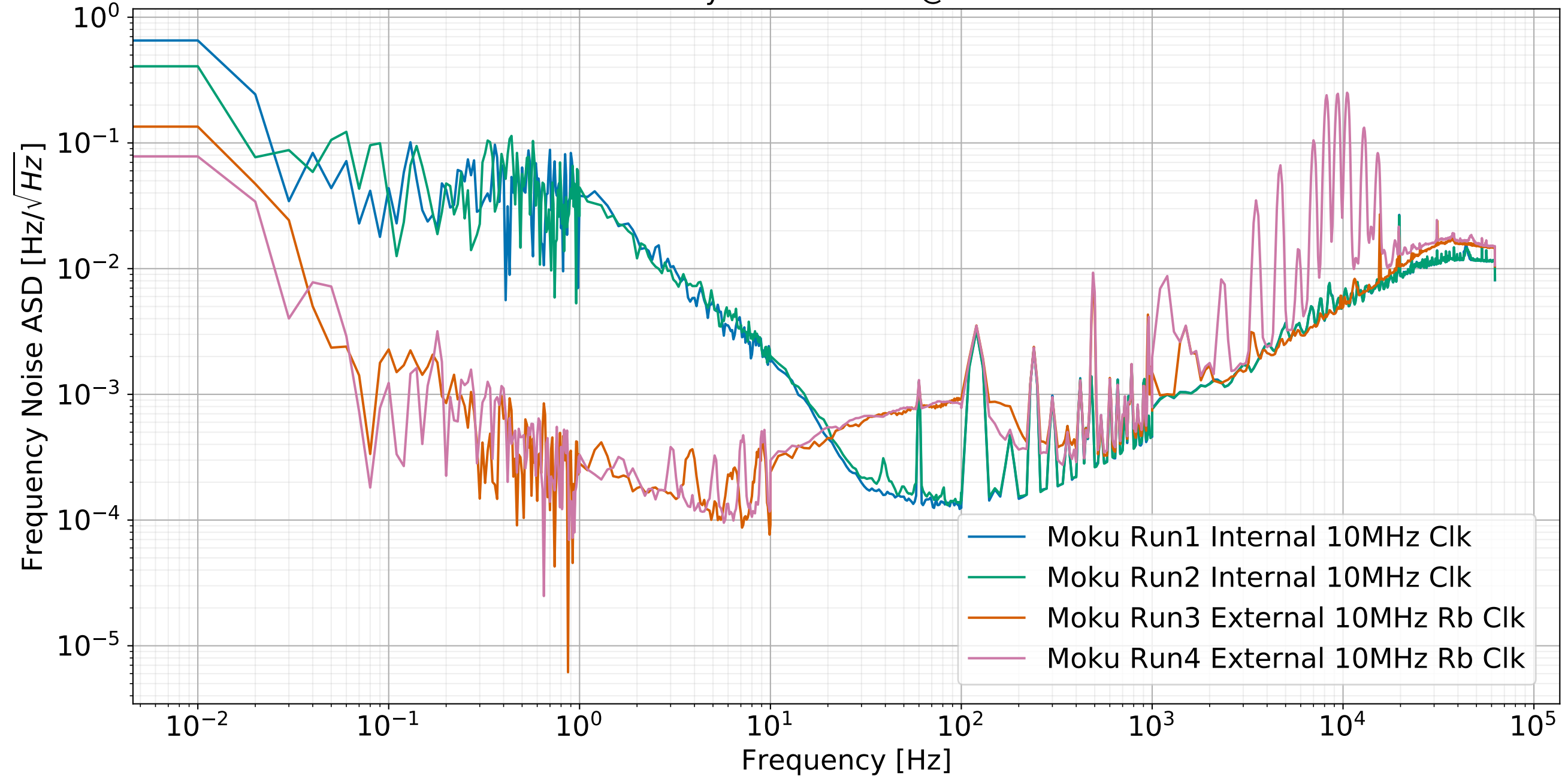
Measured frequency noise from Moku when input was Wenzel Crystal Oscillator @24.4835 MHz
