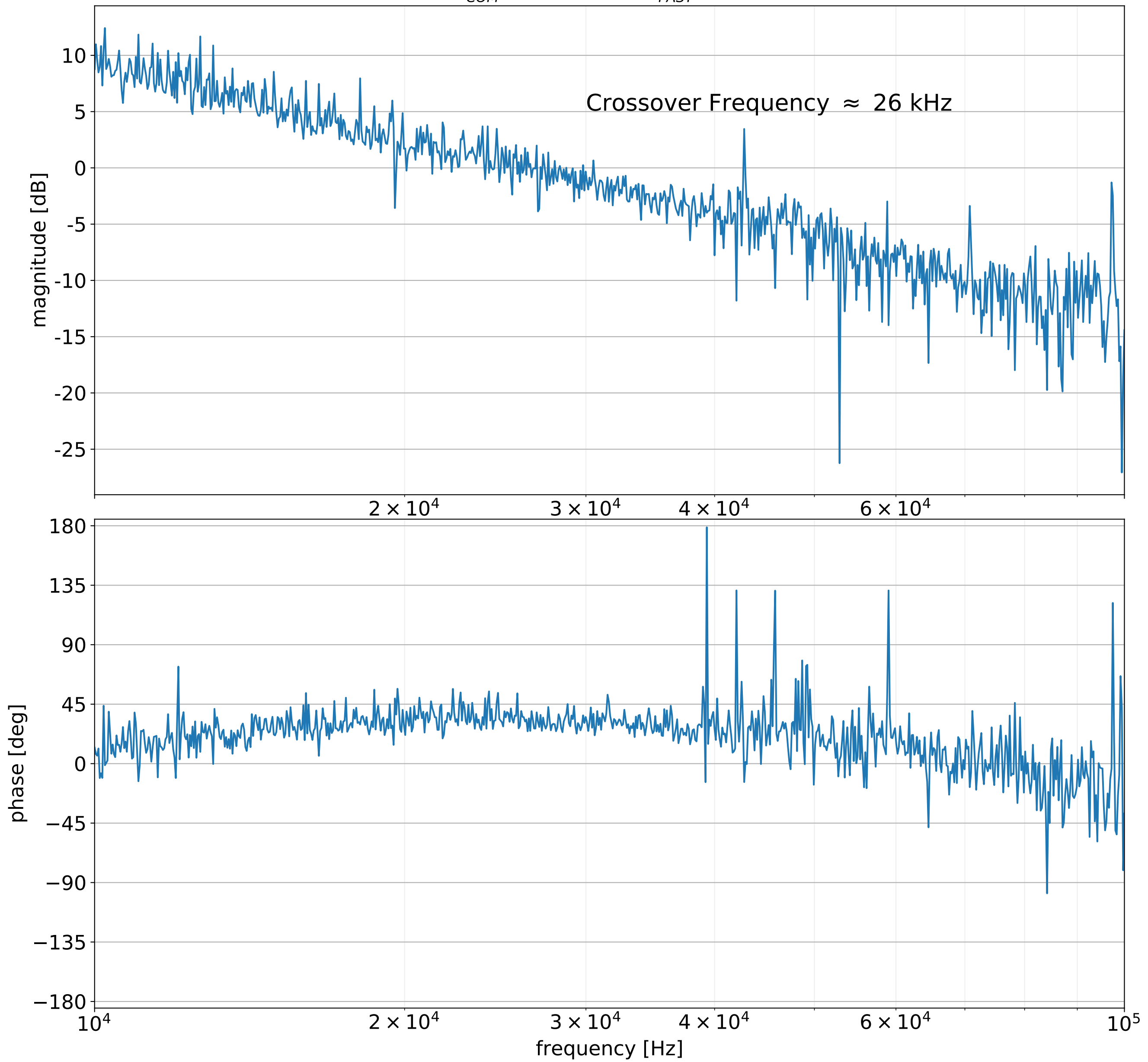
North FSS Crossover Function at G_{COM} = 0.4 dB and G_{FAST} = 46.8 dB
