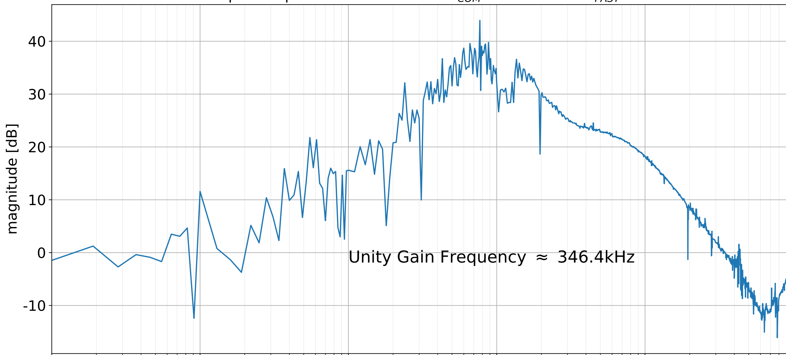
North FSS Open Loop Transfer Function at G_{COM} = 0.4 dB and G_{FAST} = 46.8 dB
