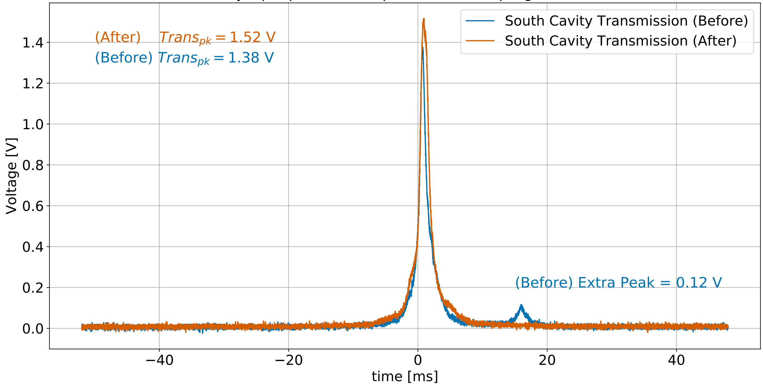
South Cavity input polarization optimization, Sampling Rate 100.0 kSa/s
