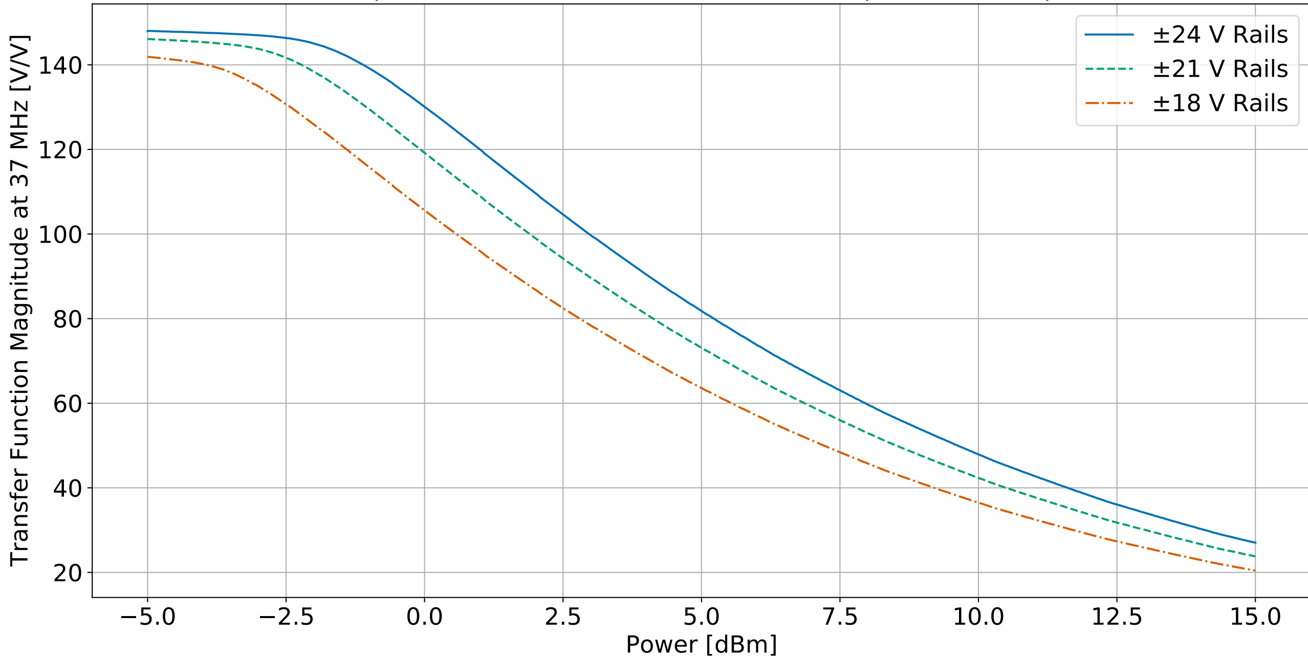
Power Sweep of South EOM Driver at 37 MHz CW Freq with different power rails
