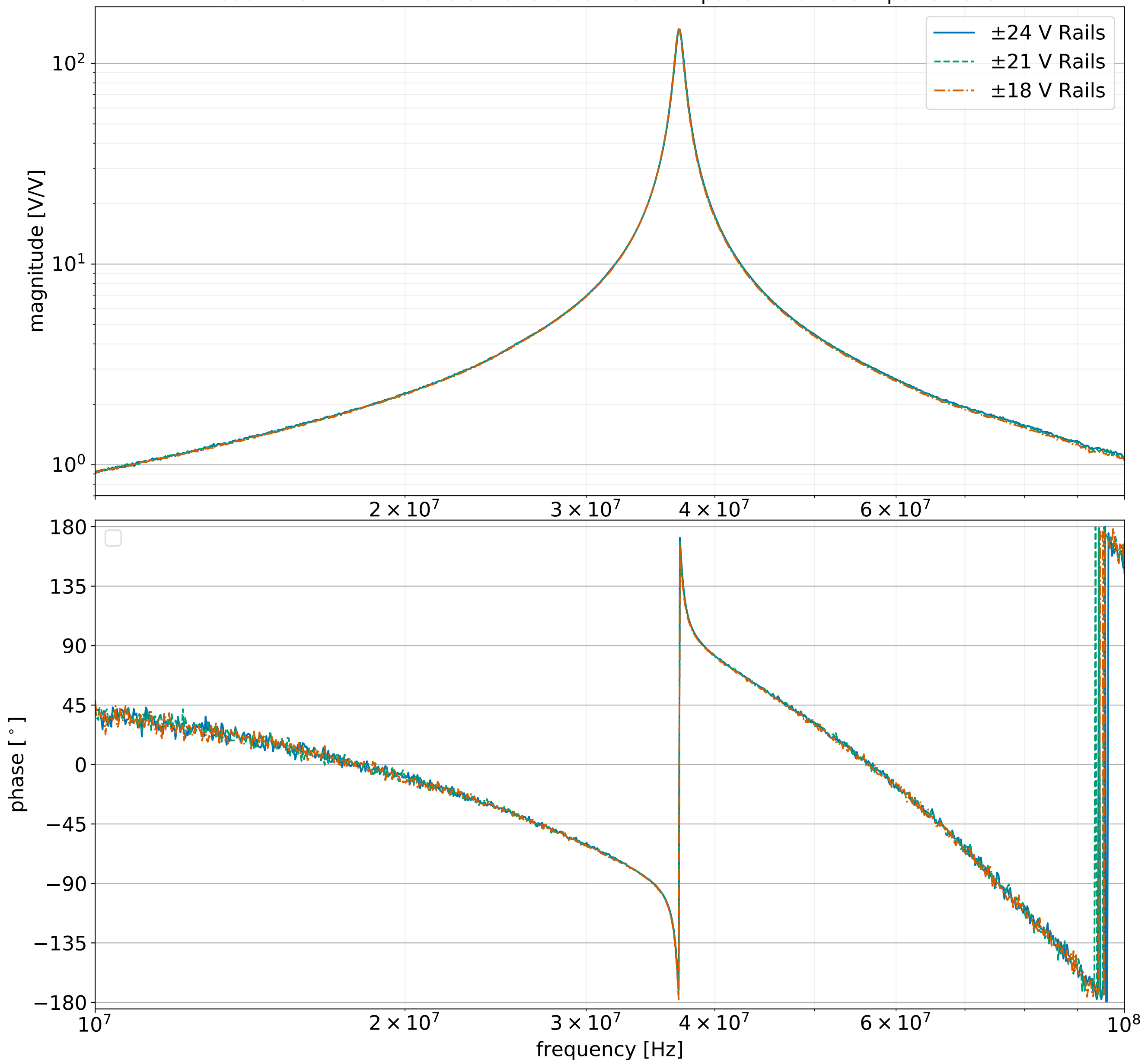
South EOM Driver Transfer Function at -10 dBm power at different power rails.
