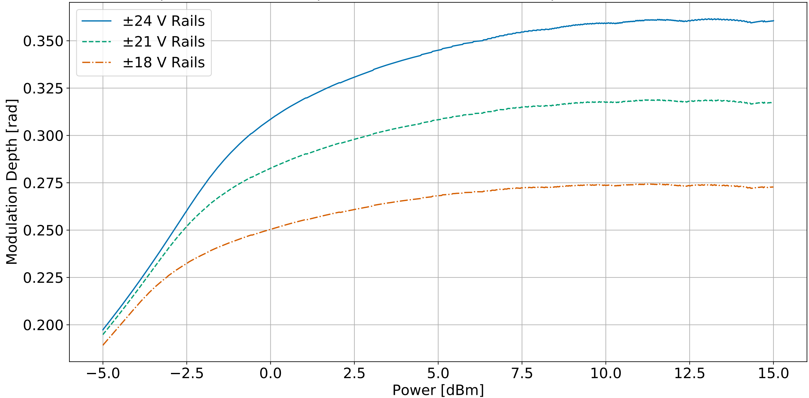
Expected modulation depth on South Path with different power rails on EOM driver
