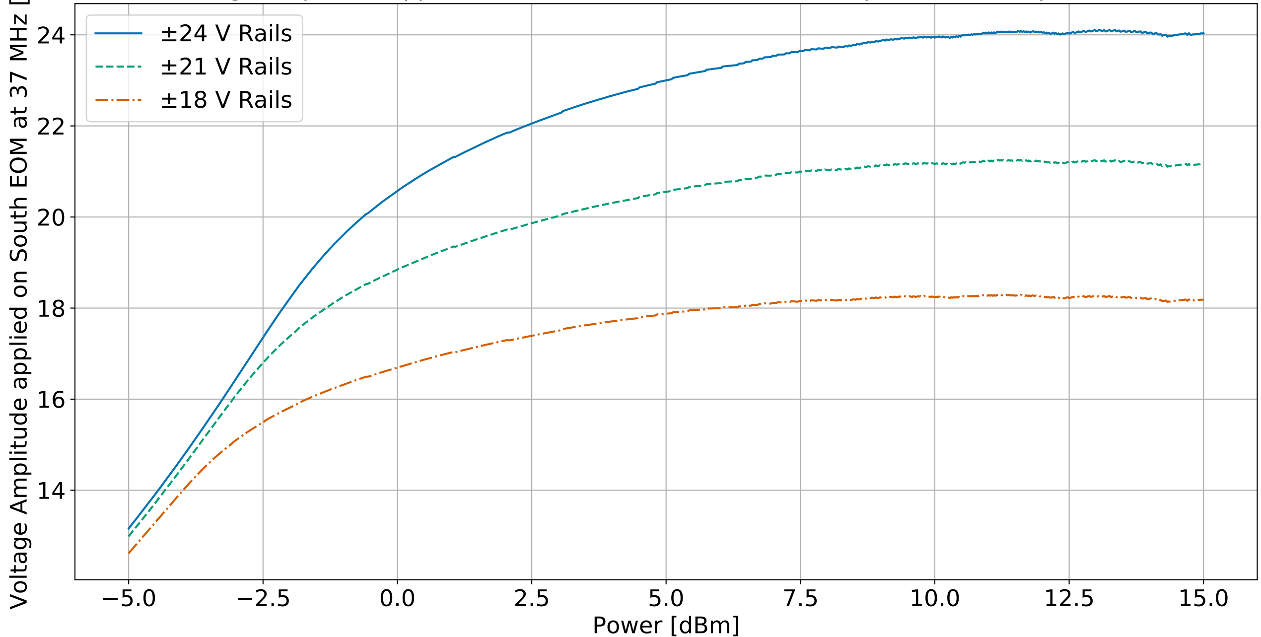
Voltage Amplitude applied on South EOM at 37 MHz CW Freq with different power rails
