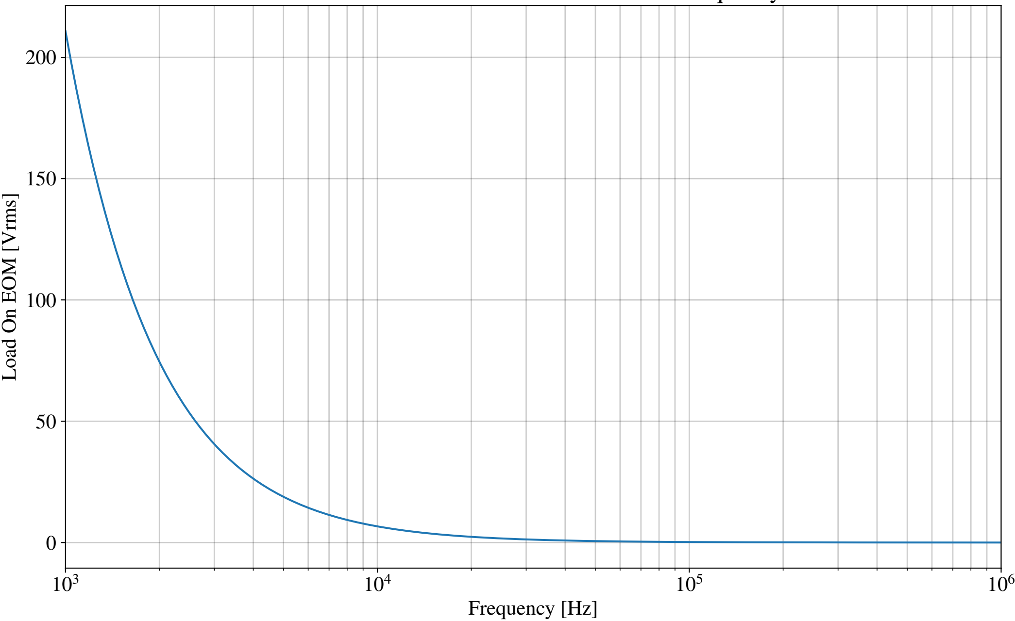
Total Noise Load On EOM As a Function Of Minimum Frequency EOM Drives To
