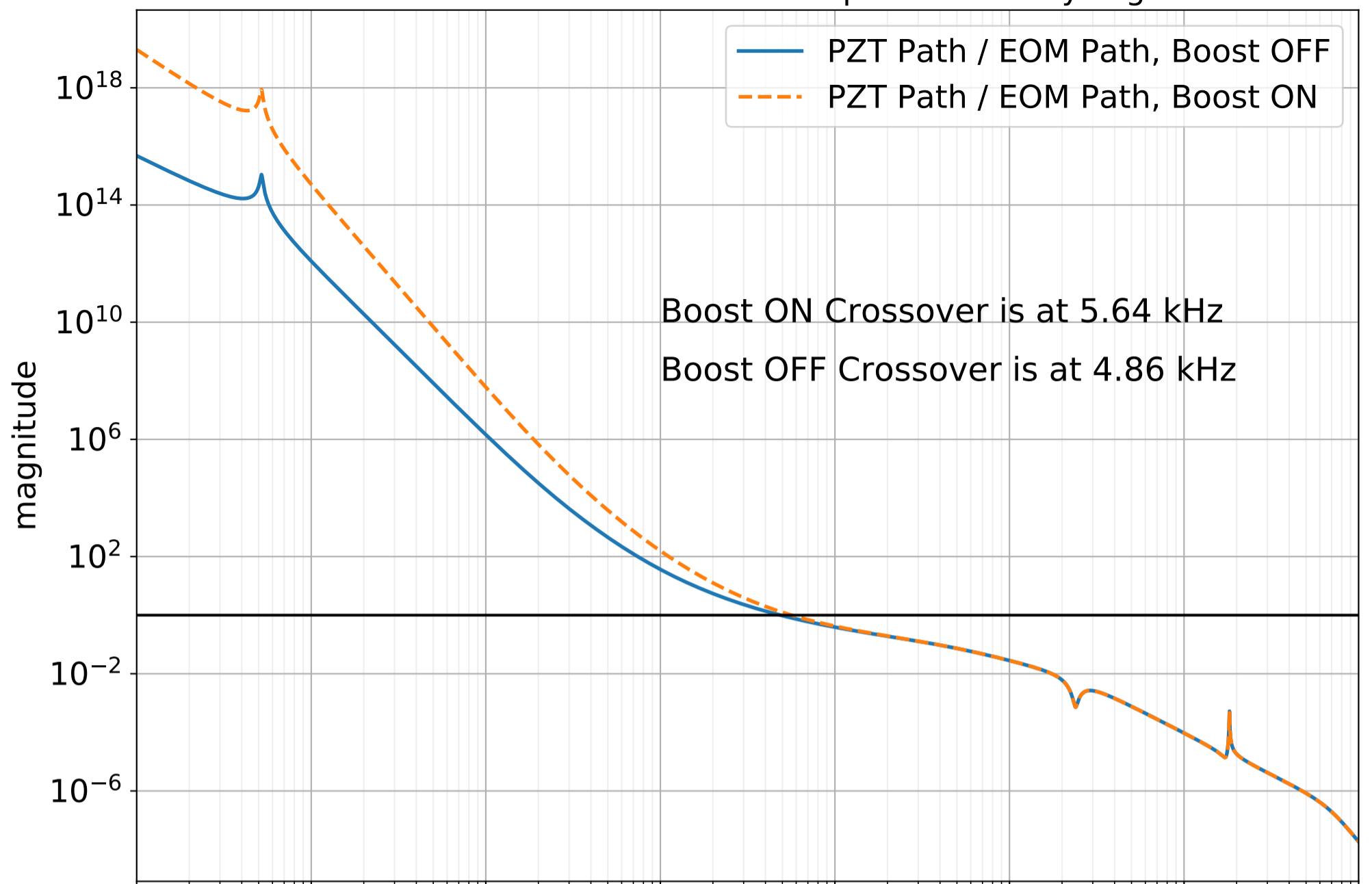
Ratio of transfer functions of PZT and EOM paths for analyzing crossover.
