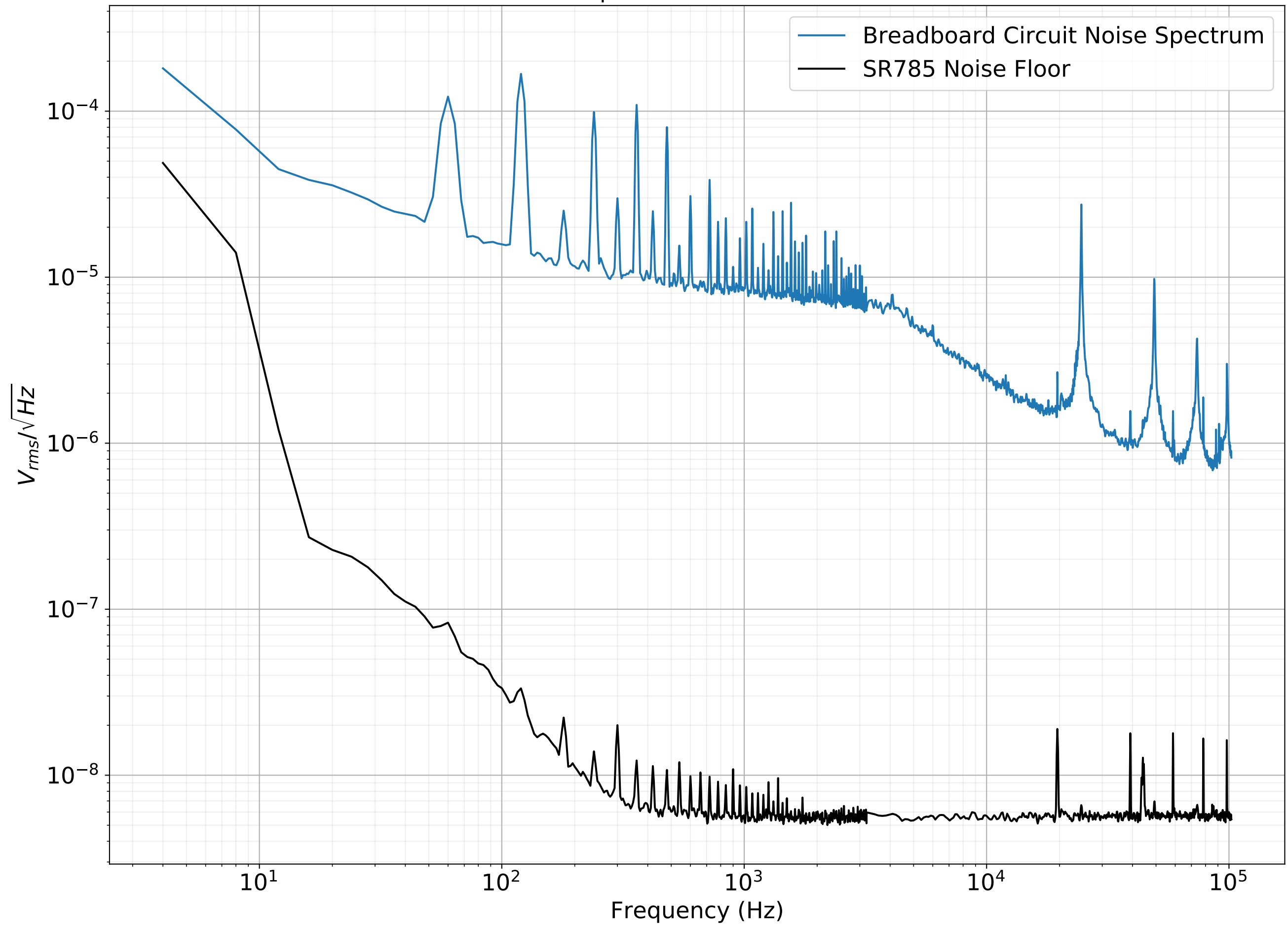
Measured output noise of breadboard circuit
