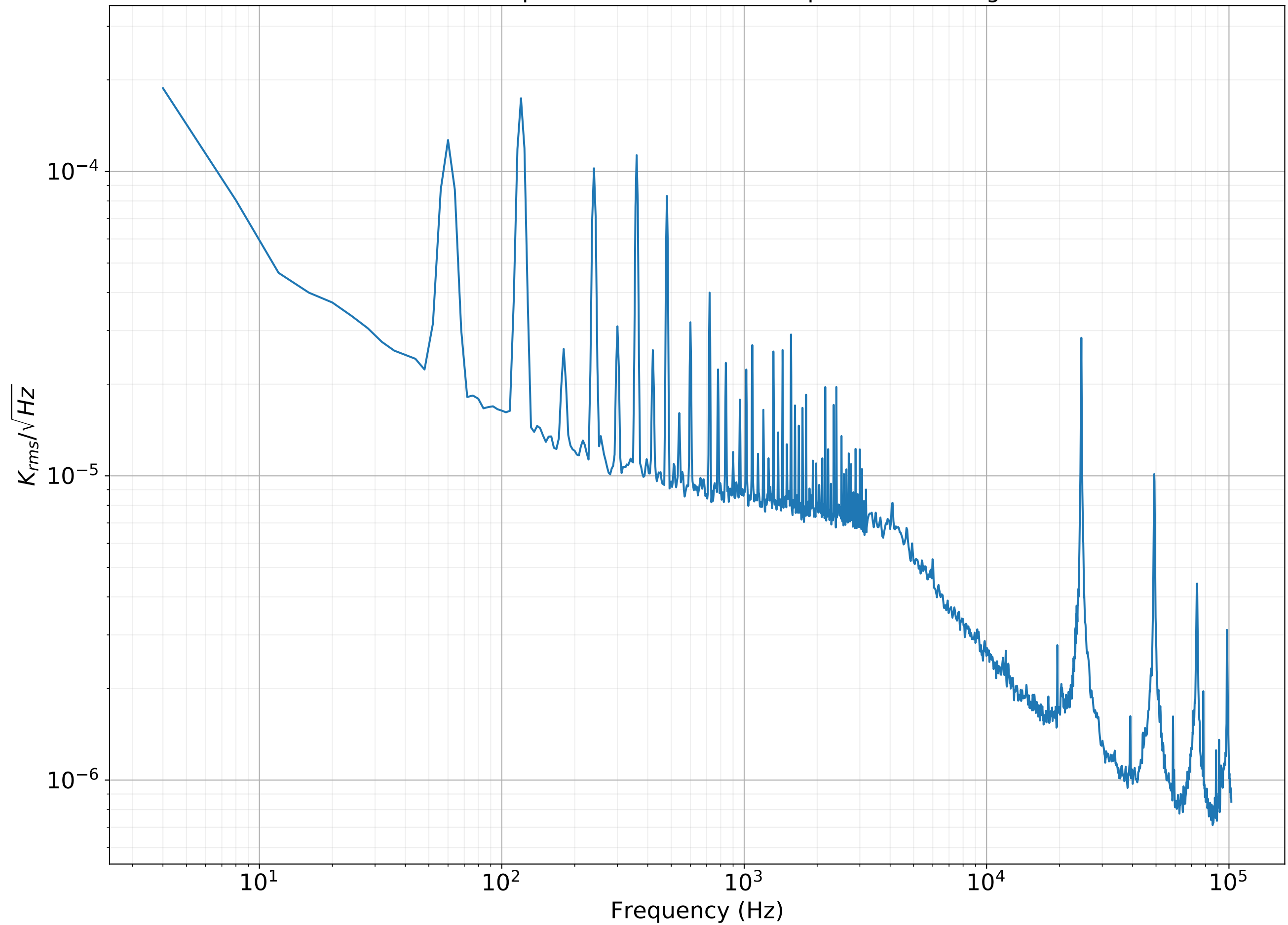
Effective input referred noise of temperature sensing
