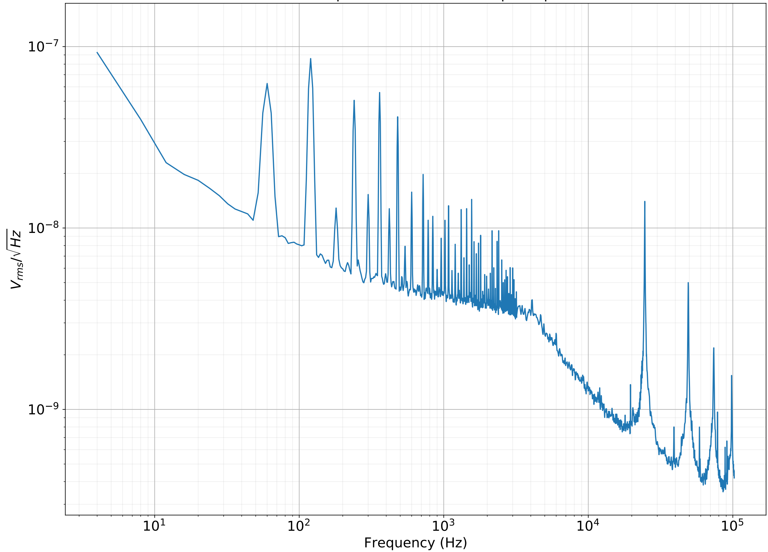
Effective input referred noise of amplifier part
