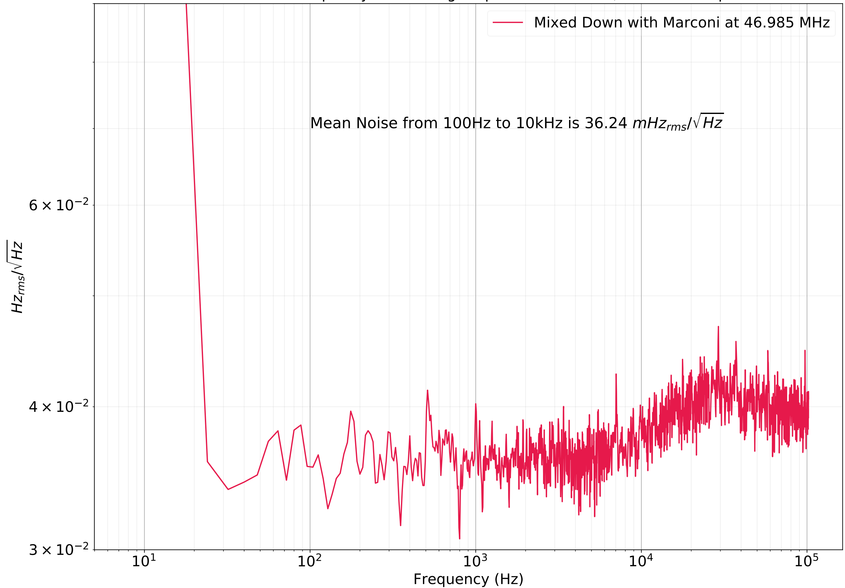
New Focus 1811-FC Dark Noise Contribution Spectrum (Mixed Down) Jan 23, 2019 Converted to effective frequency noise using Amplifier Gain = 200, Actuation Slope = 1kHz/V
