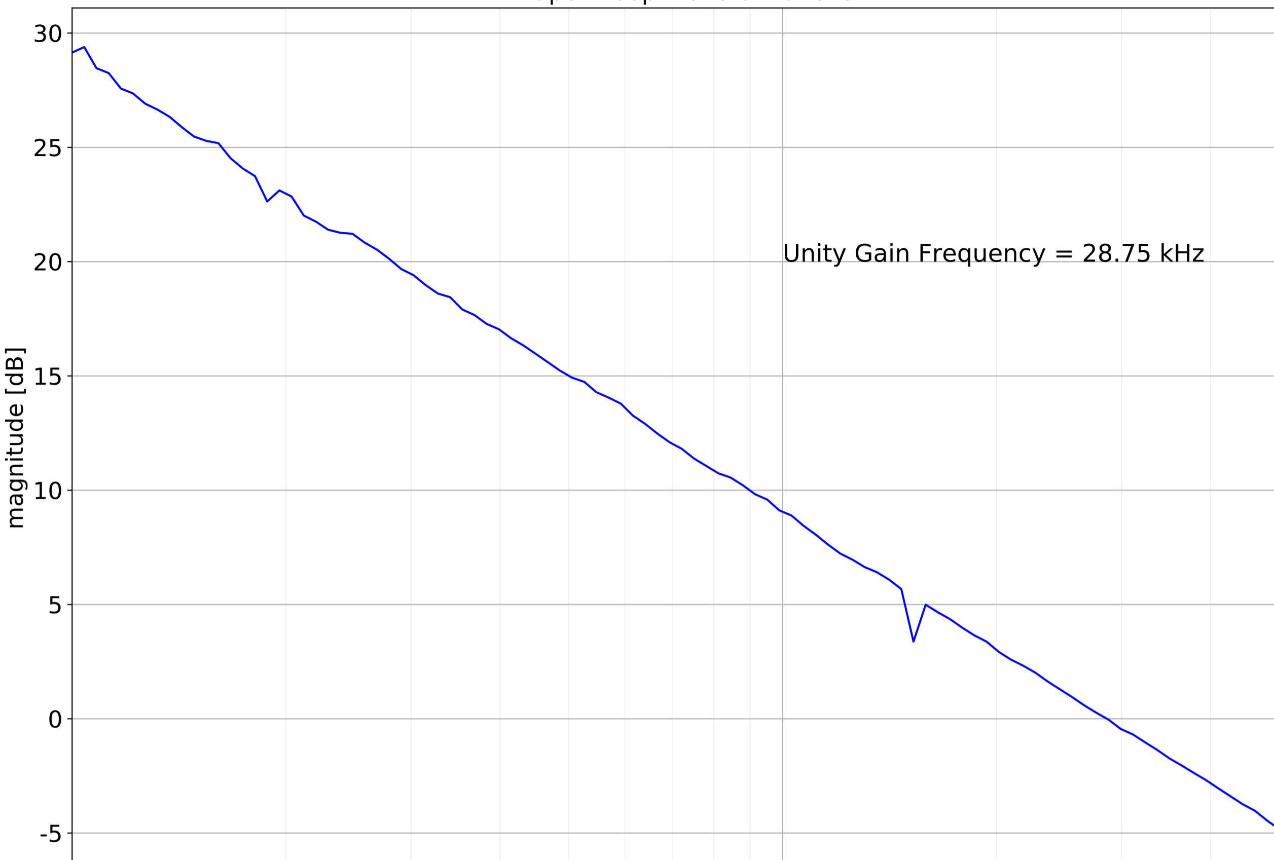
PLL Open Loop Transfer Function
