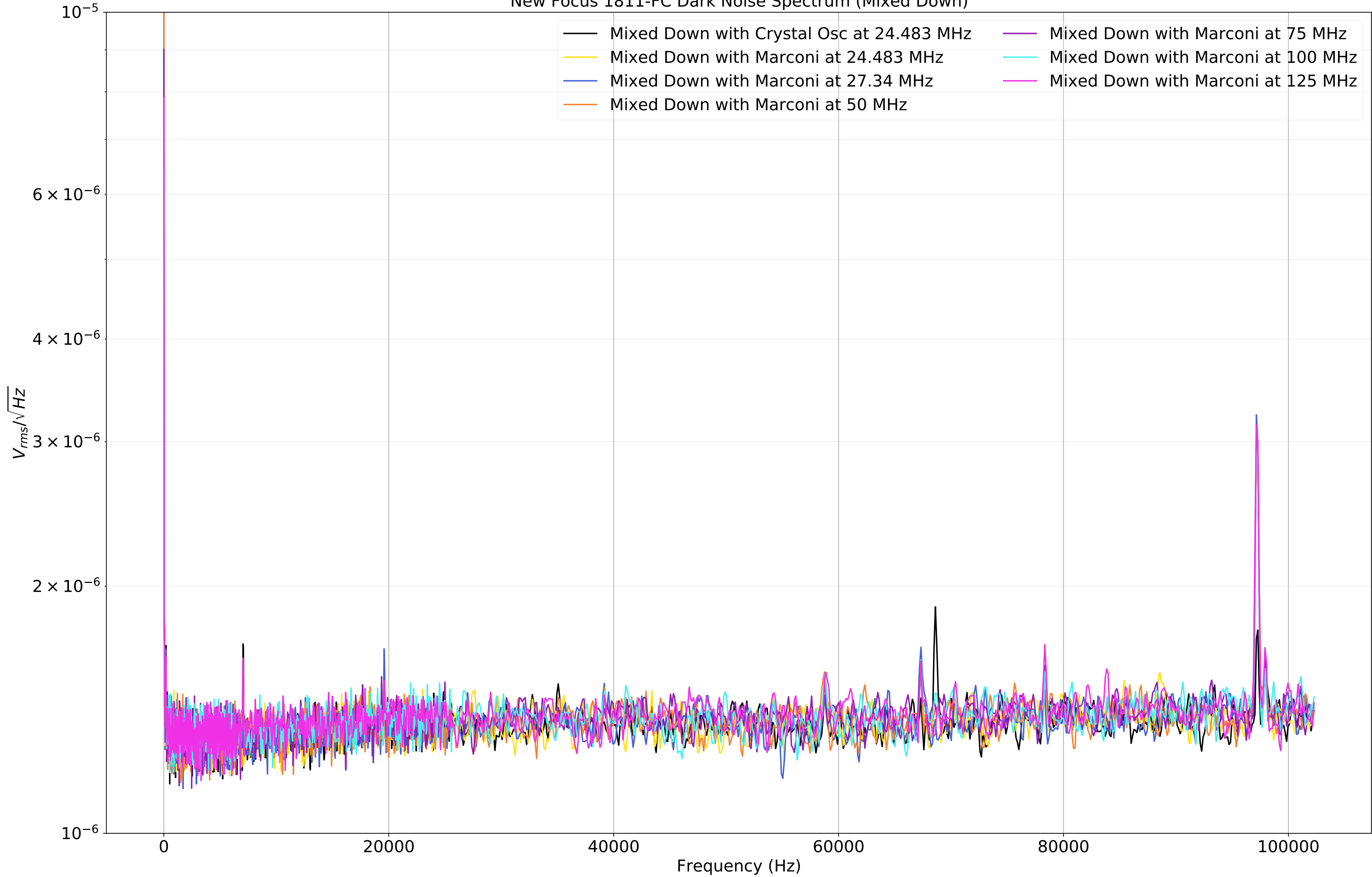
New Focus 1811-FC Dark Noise Spectrum (Mixed Down)
