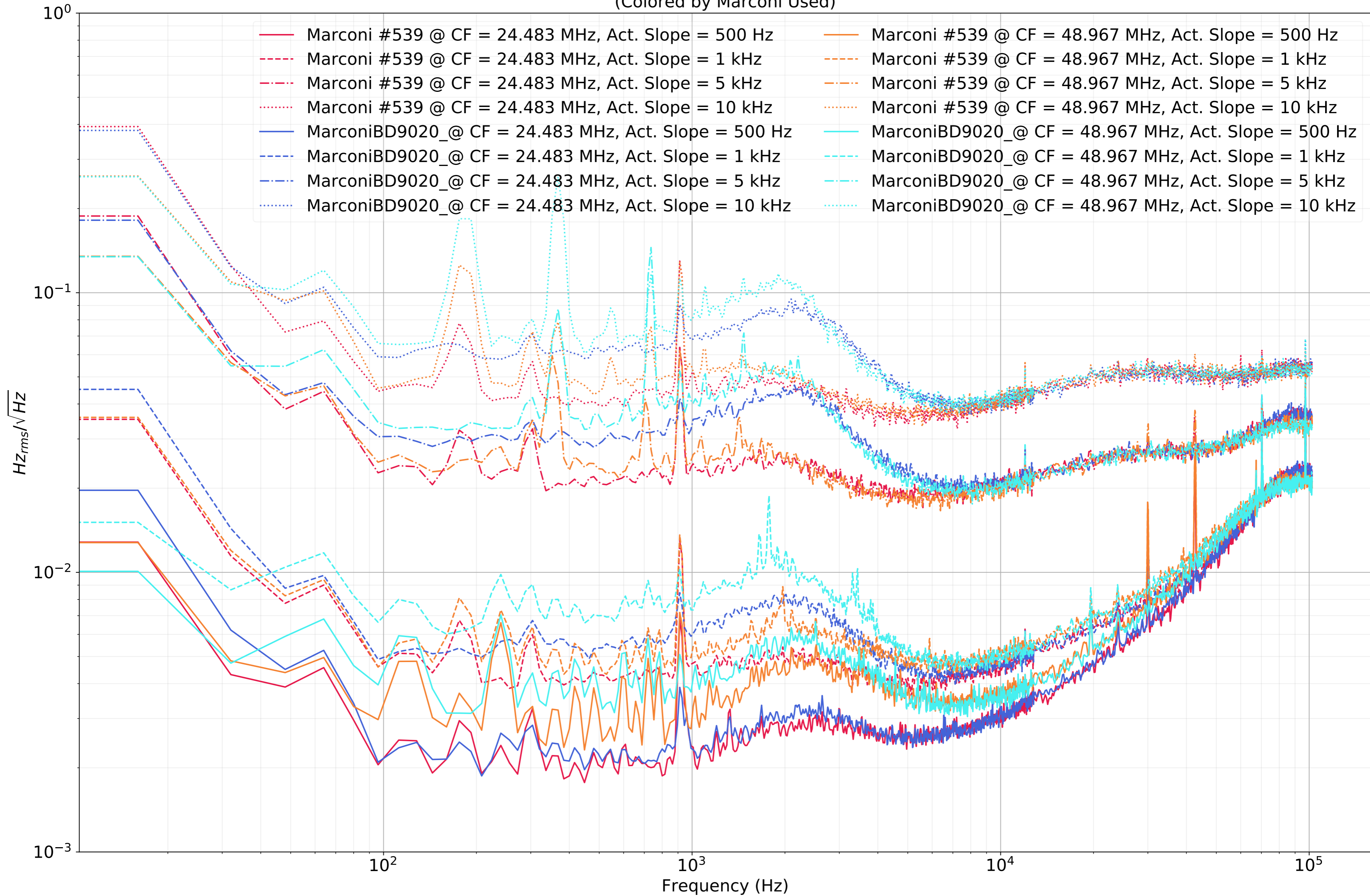
Beat Note Noise Spectrum for different Marconi in PLL At different Wenzel Crystal Frequency (CF) and actuation slopes (Act. Slope) (Colored by Marconi Used)
