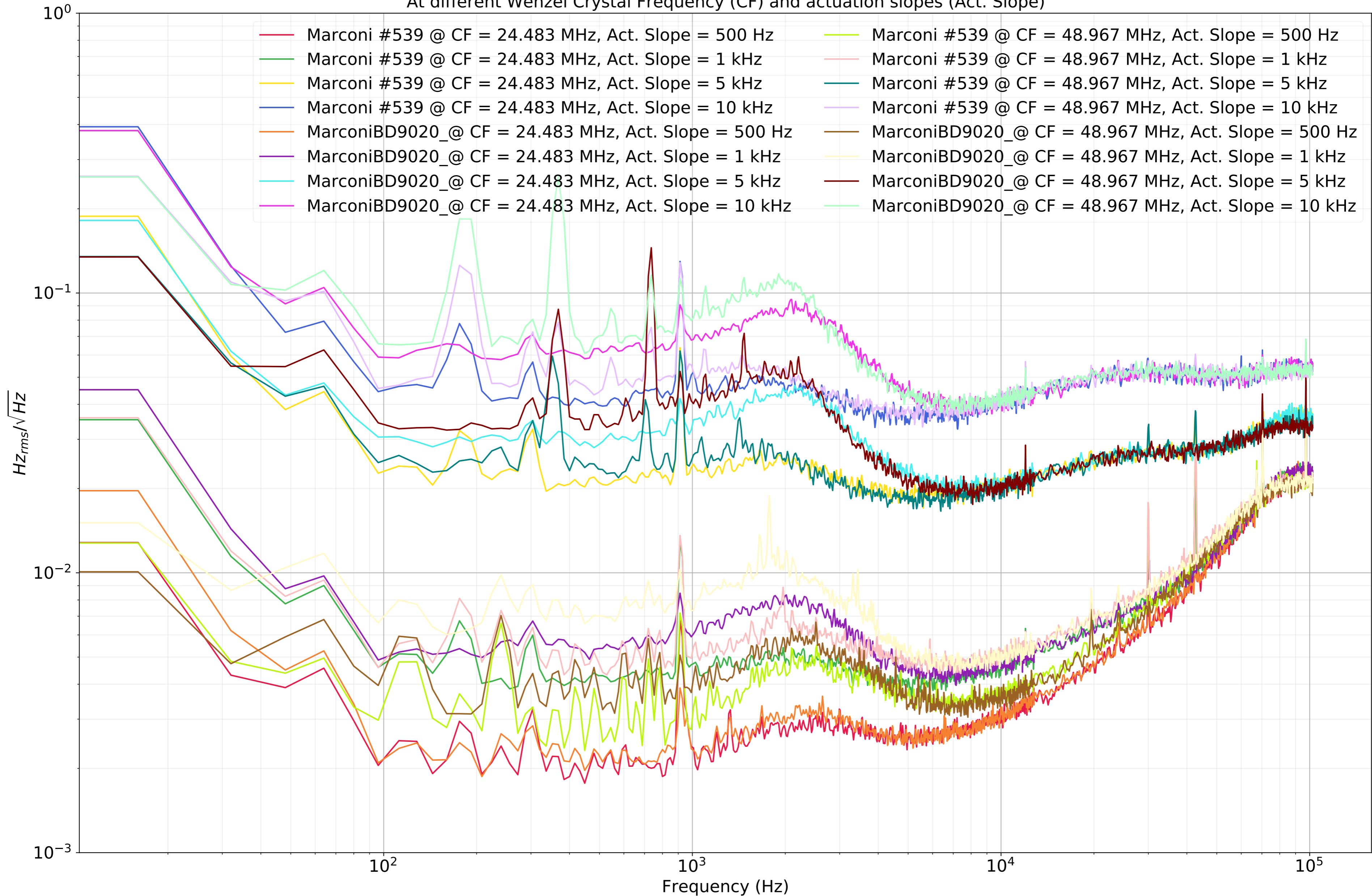
Beat Note Noise Spectrum for different Marconi in PLL At different Wenzel Crystal Frequency (CF) and actuation slopes (Act. Slope)
