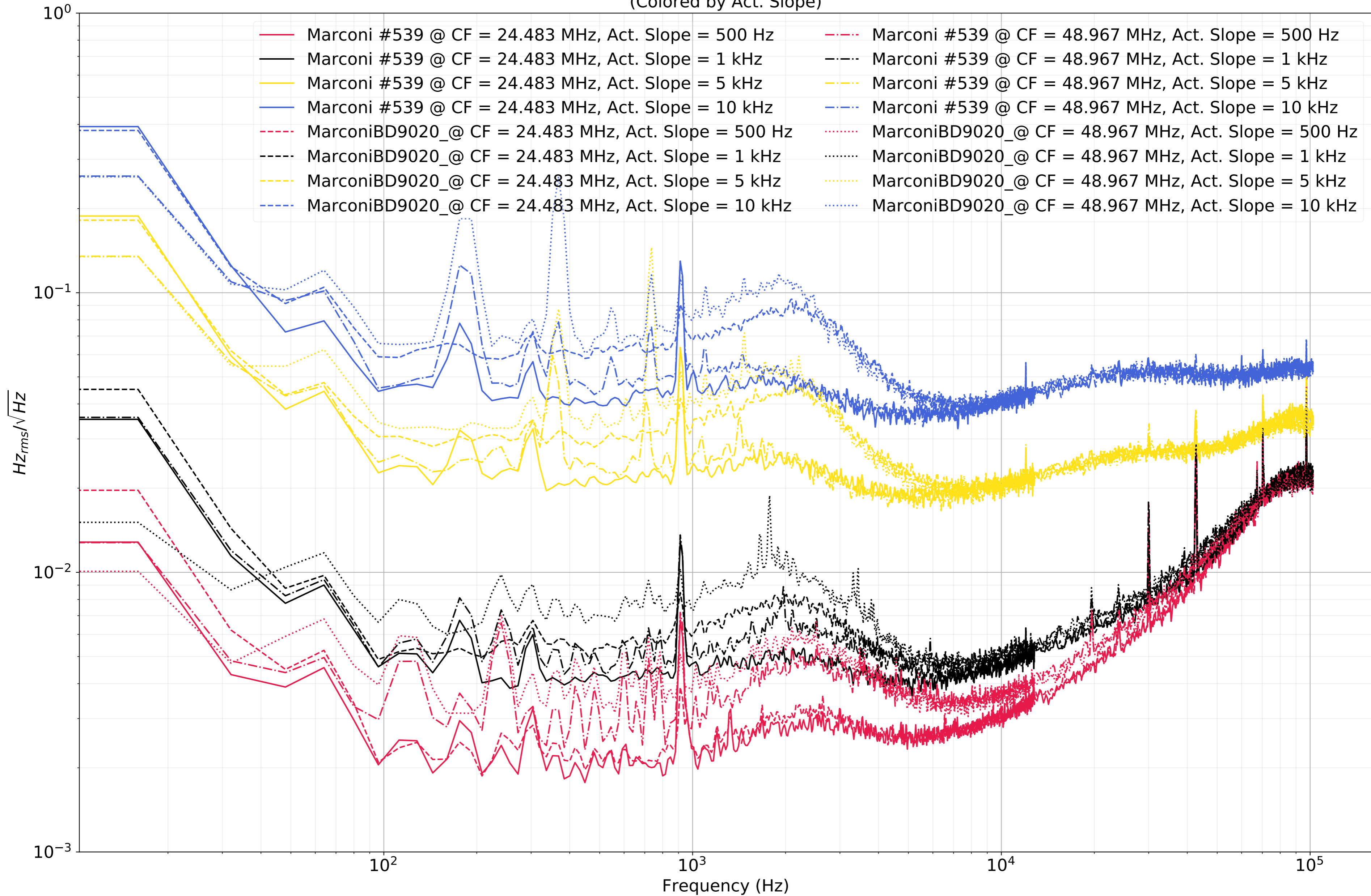
Beat Note Noise Spectrum for different Marconi in PLL At different Wenzel Crystal Frequency (CF) and actuation slopes (Act. Slope) (Colored by Act. Slope)
