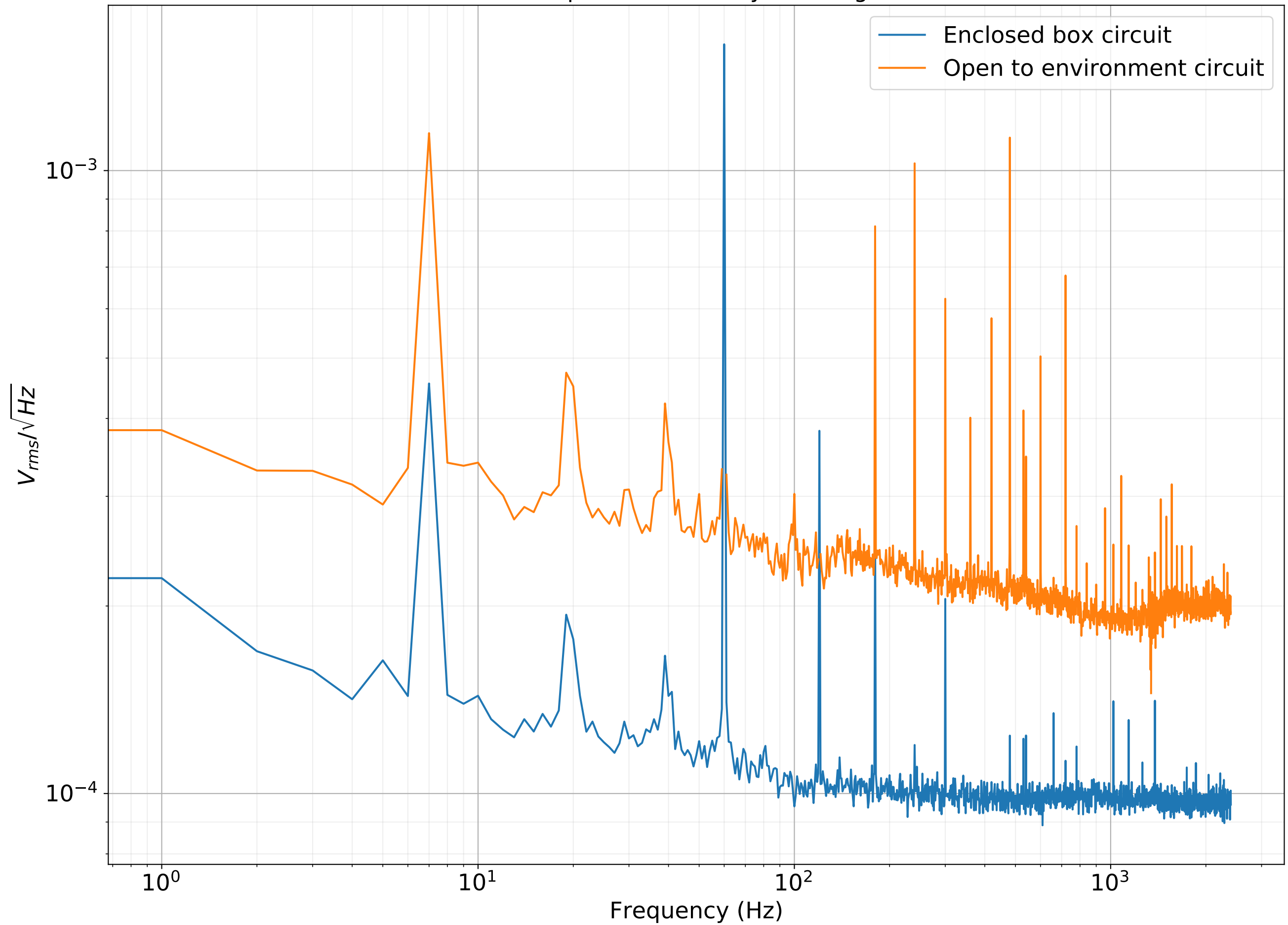
Estimated output noise density of a single channel
