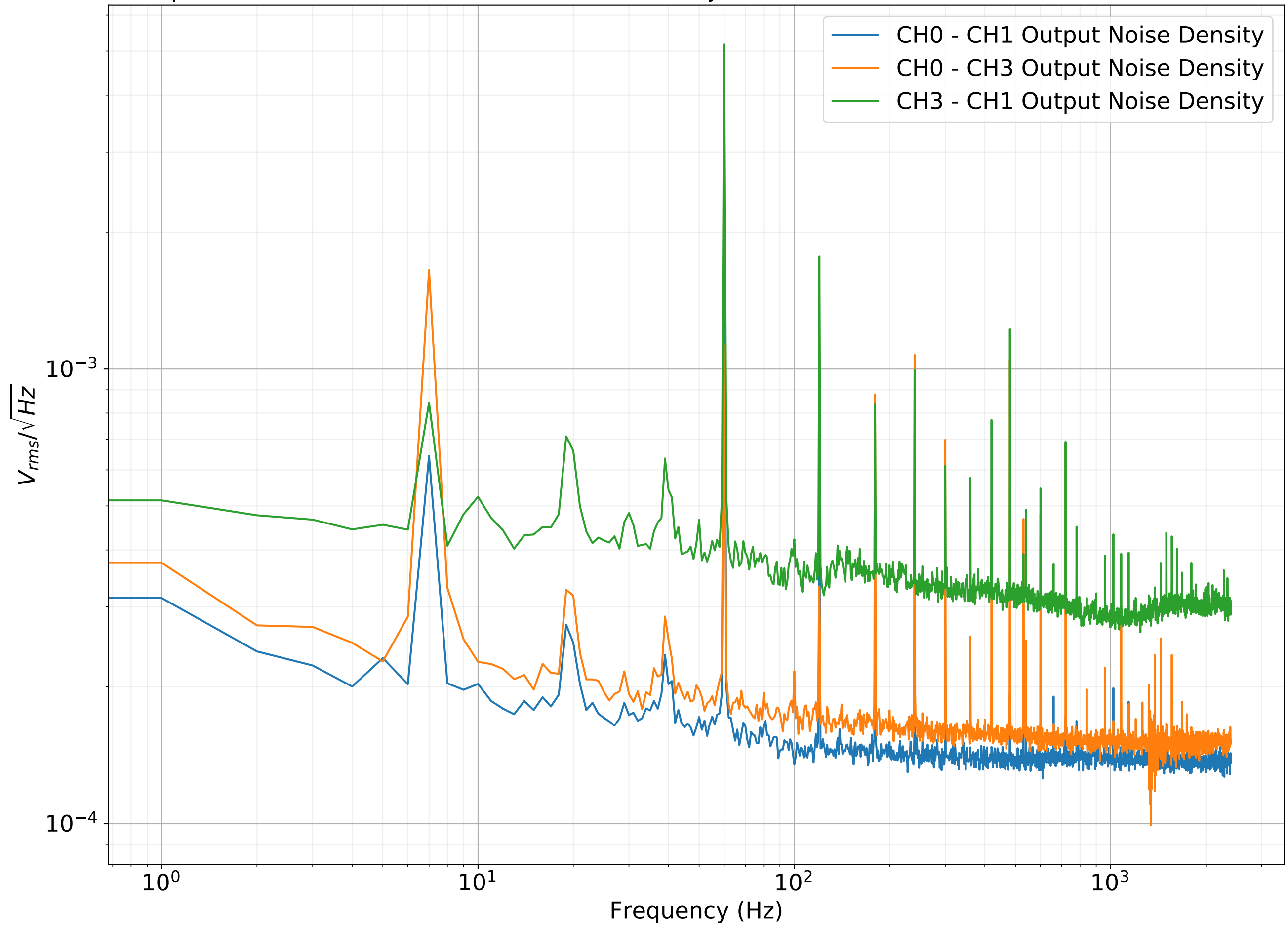
Output Noise of difference of different channels adjusted with noise of subtration circuit and SR785
