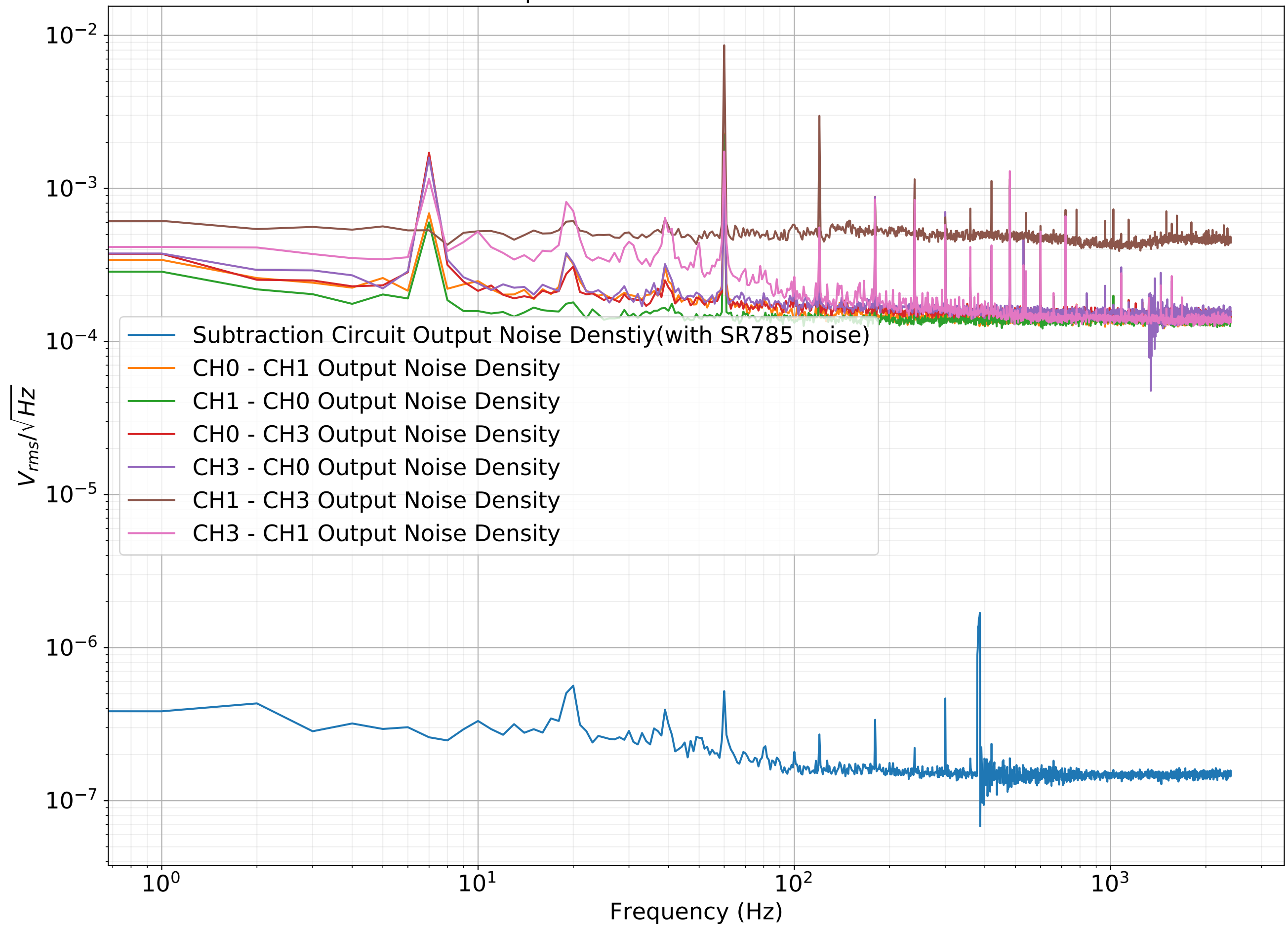
Measured output noise of difference of different channels
