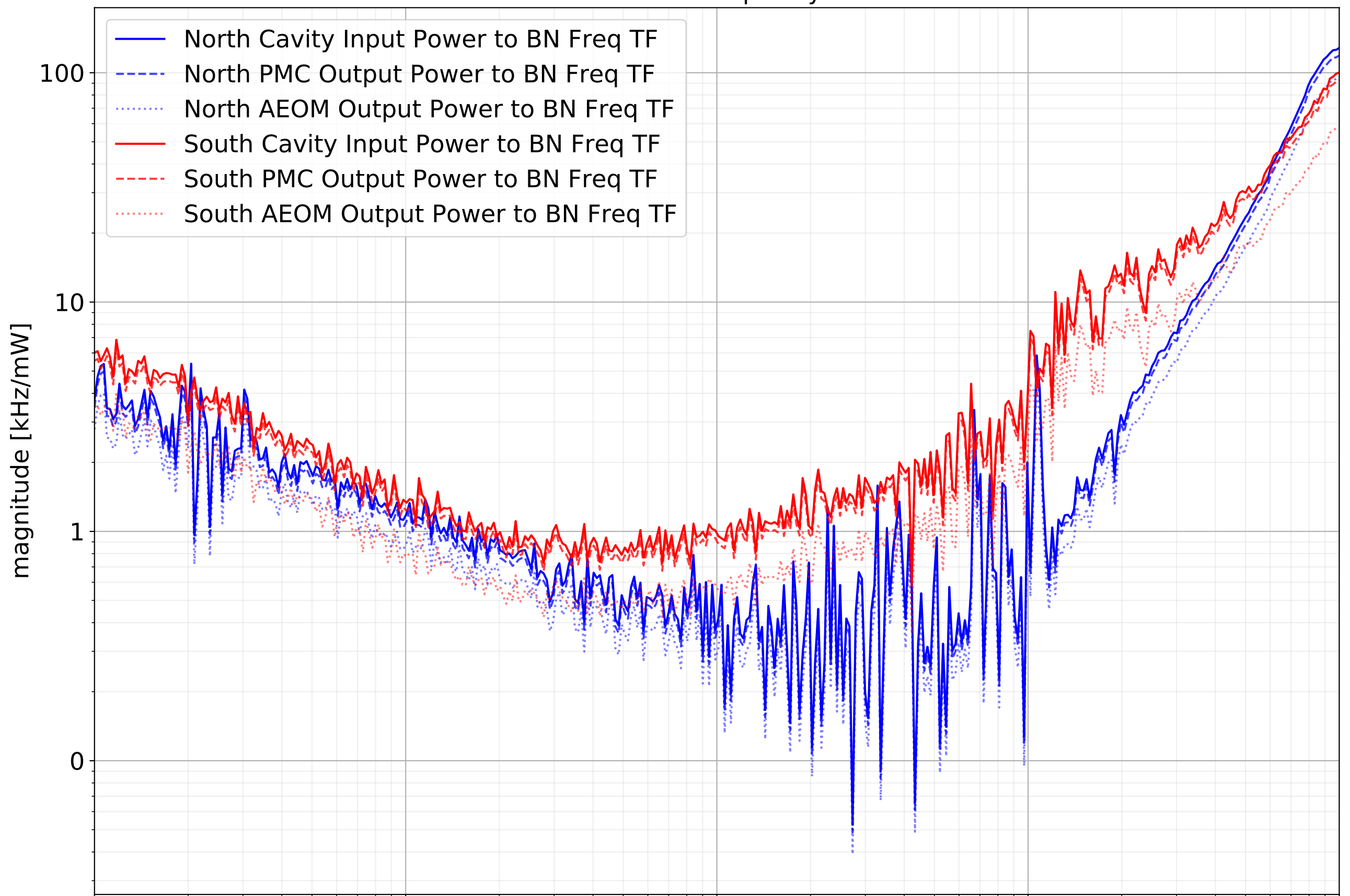
Laser Power Noise to Beat Note Frequency Noise Transfer Functions
