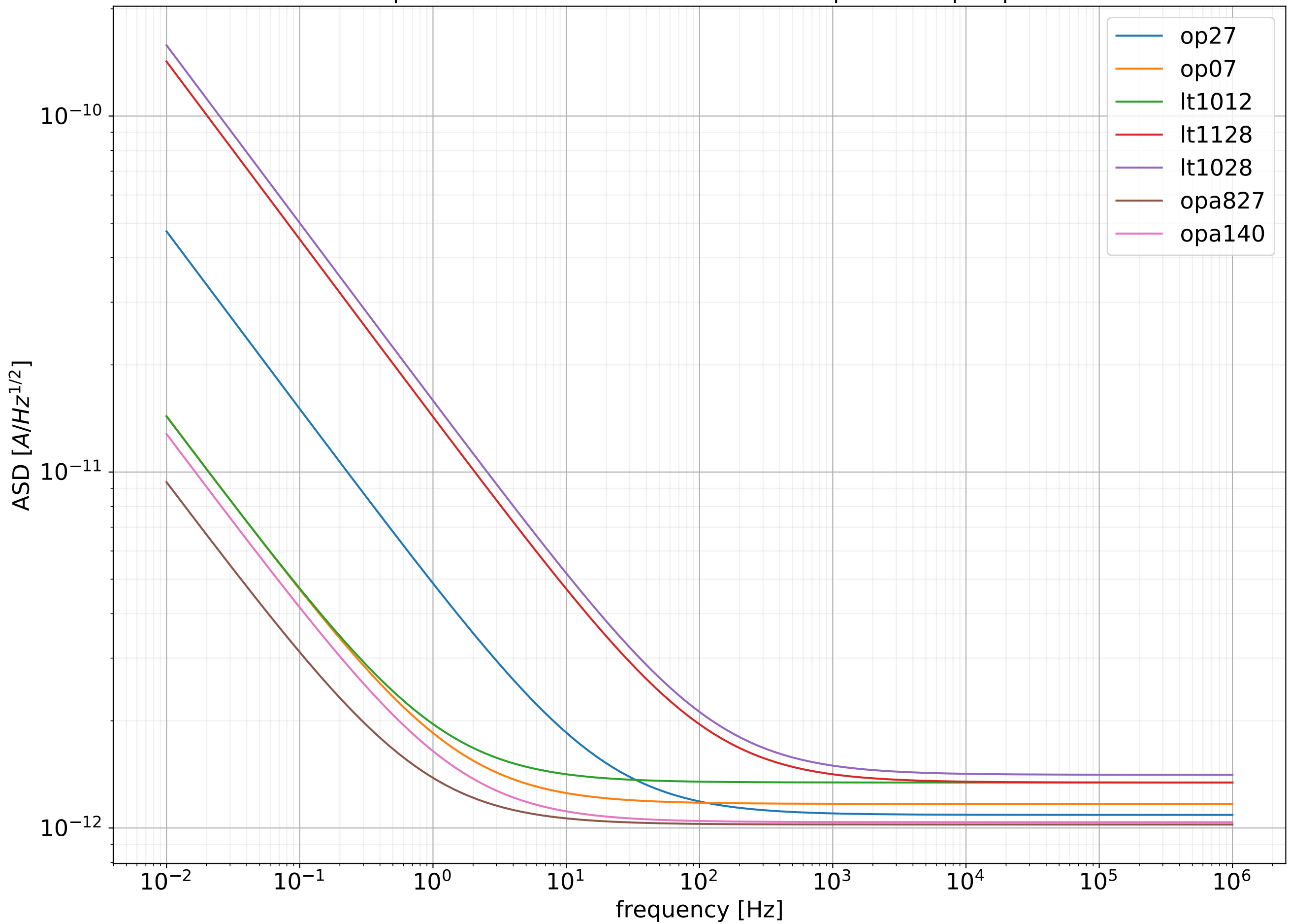
Input referred noise for different transimpedance opamps
